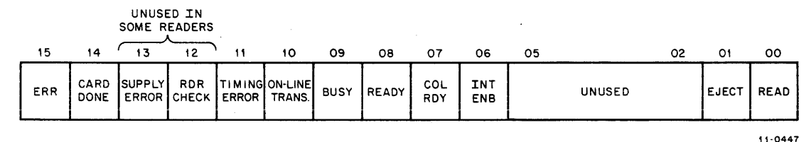
Figure 4-1 Status Register Bit Assignments
