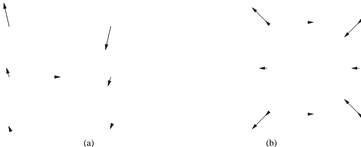
Figure 6: Minimum eigenvector for a three-frame perspective reconstruction problem with pure z translation: (a) top-down view ( x-z ), (b) frontal view ( x-y ). The main ambiguity is a rocking confusion between sideways camera translation and rotation, which affects the points furthest back.
