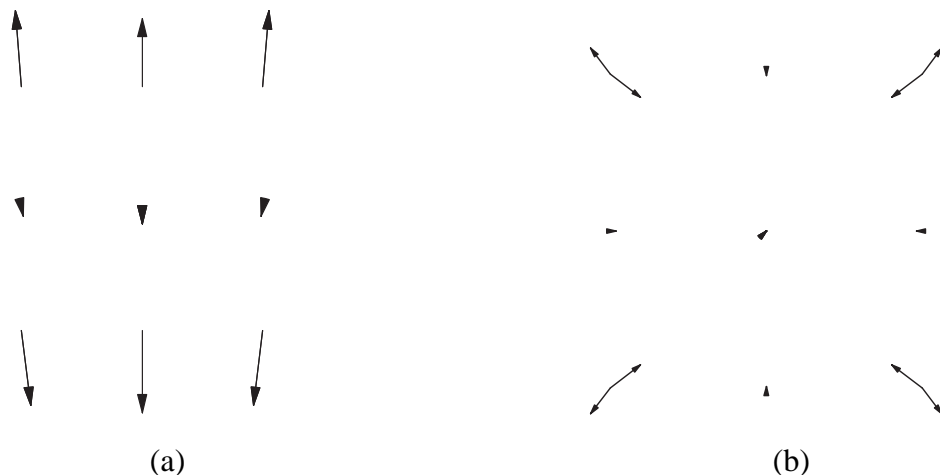
Figure 5: Minimum eigenvector for a three-frame perspective reconstruction problem: (a) top-down view ( x-z ), (b) frontal view ( x-y ). While the main ambiguity is a z scaling, the vector is not exactly an affine transform of the 3-D points on the unit cube.
