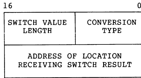
Figure 6-3 Format of Switch Value Descriptor Table Entry
