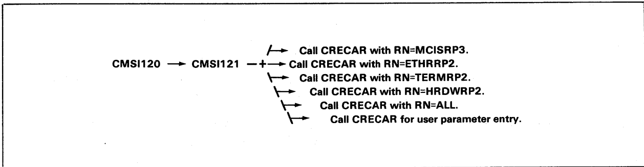
Figure 1-14. CDCNET NPA Interface Flowchart
