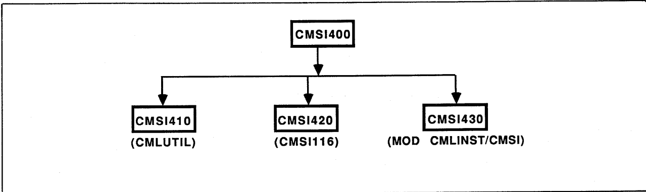
Figure 1-31. Utilities Interface Flowchart
