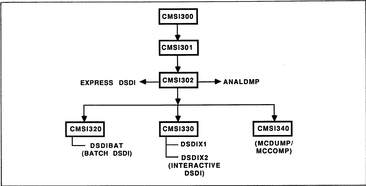
Figure 1-27. DUMP Interface Flowchart
