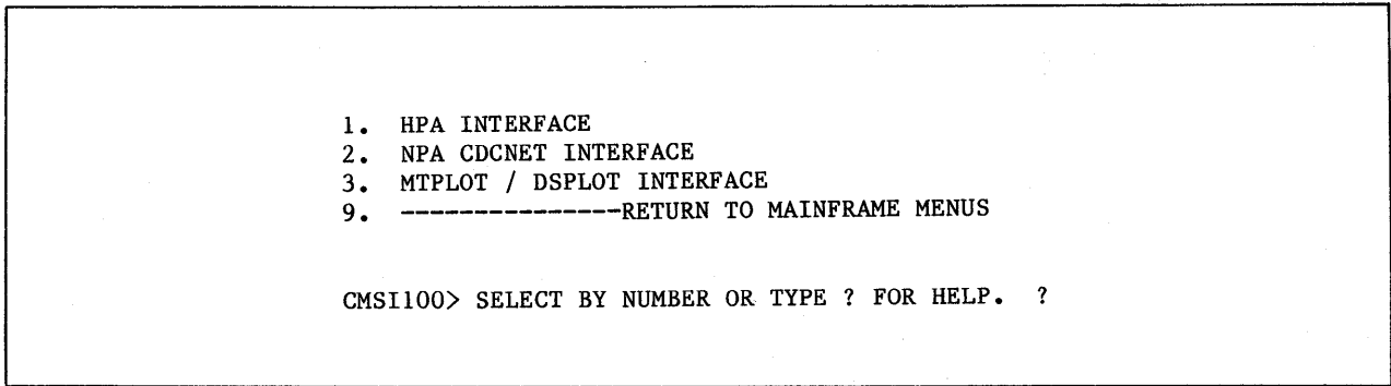
Figure 1-9. Analysis Interface
