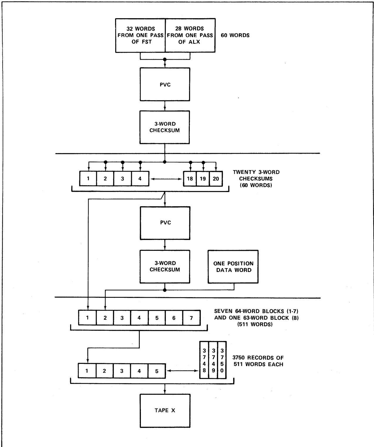
Figure 4-5. Generate Mode Flowchart
