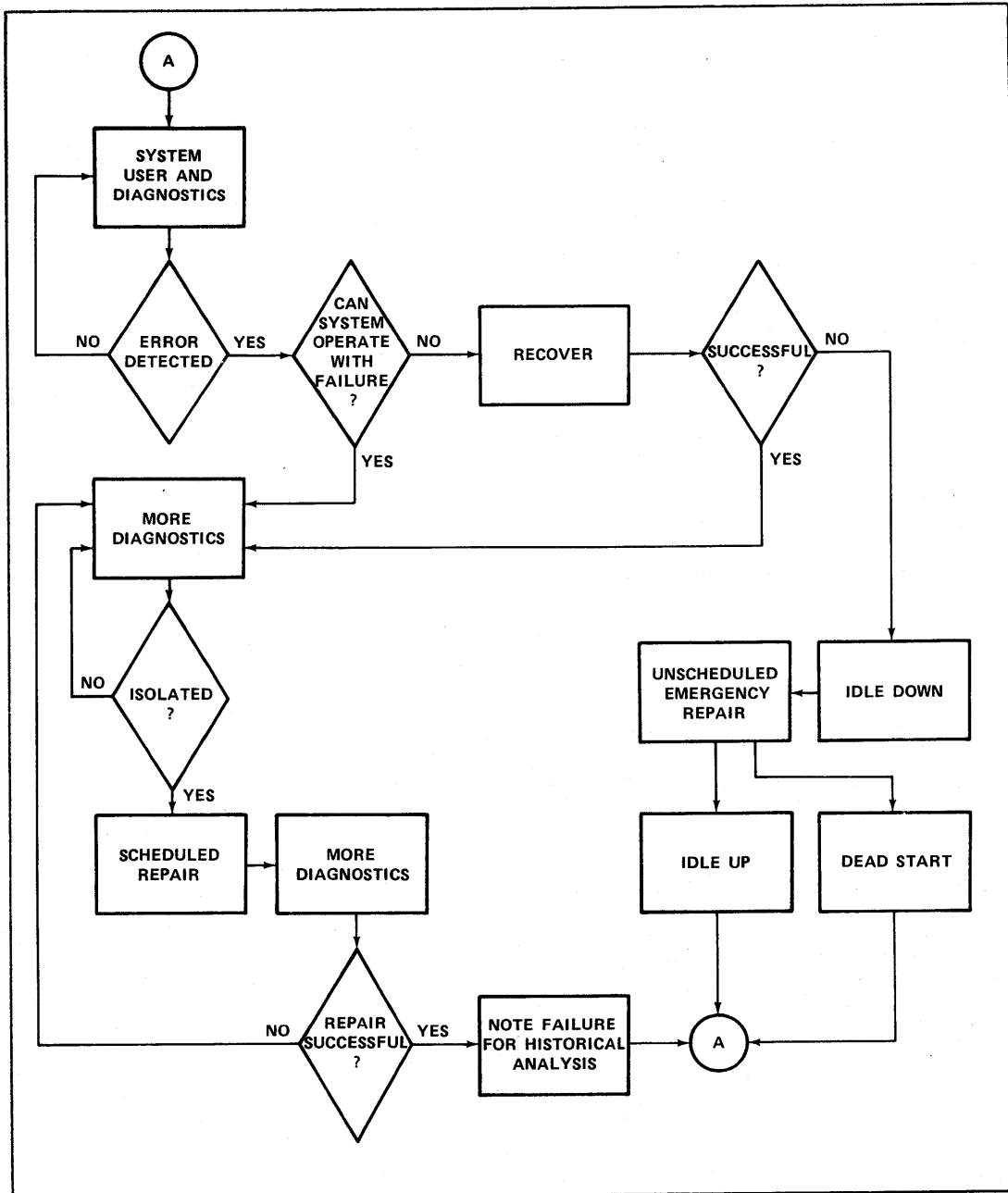
Figure 1-3. Maintenance Flowchart
