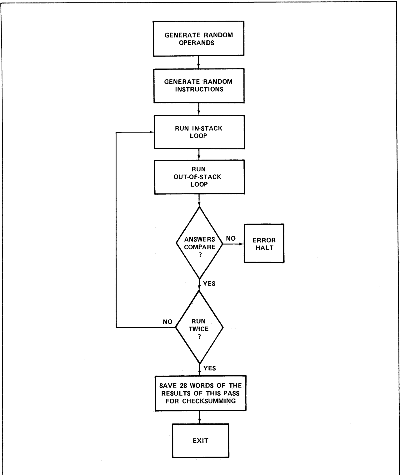
Figure 4-4. ALX Flowchart
