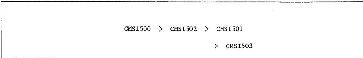
Figure 1-32. Reinitialization Flowchart
