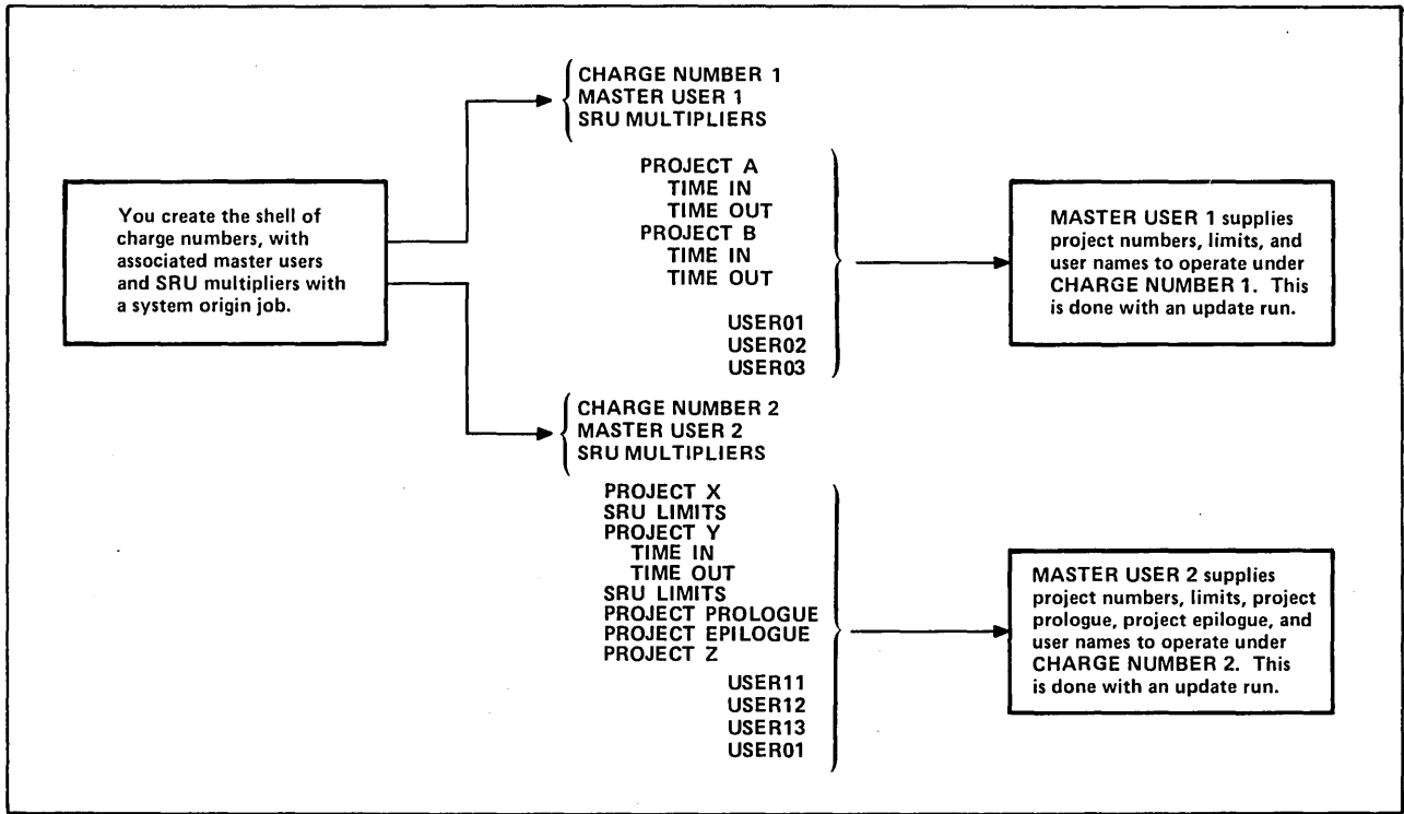
Figure 3-1. Representative Structure of a PROFILA File
