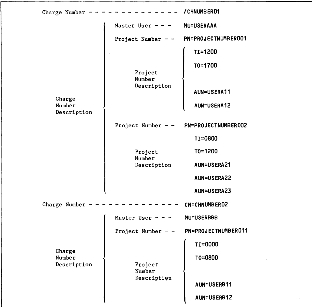
Figure 3-10. Sample Input Stream for Use with PROFILE
