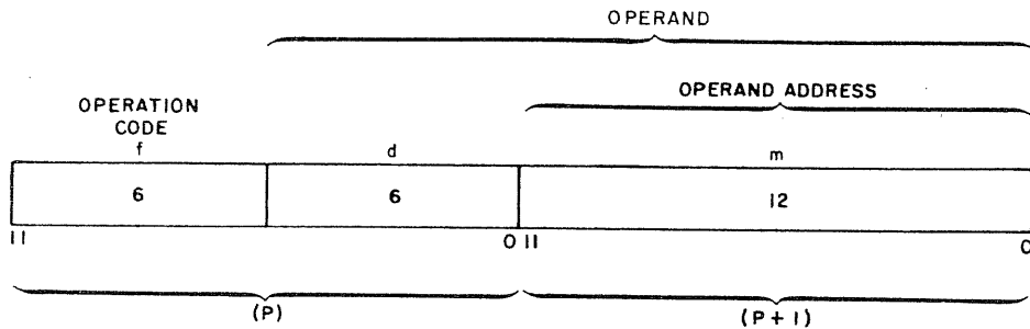
Figure 2-2. PPU and PP 24-Bit Instruction Format
