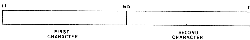
Figure 3-4. Display Station Character Data Word
