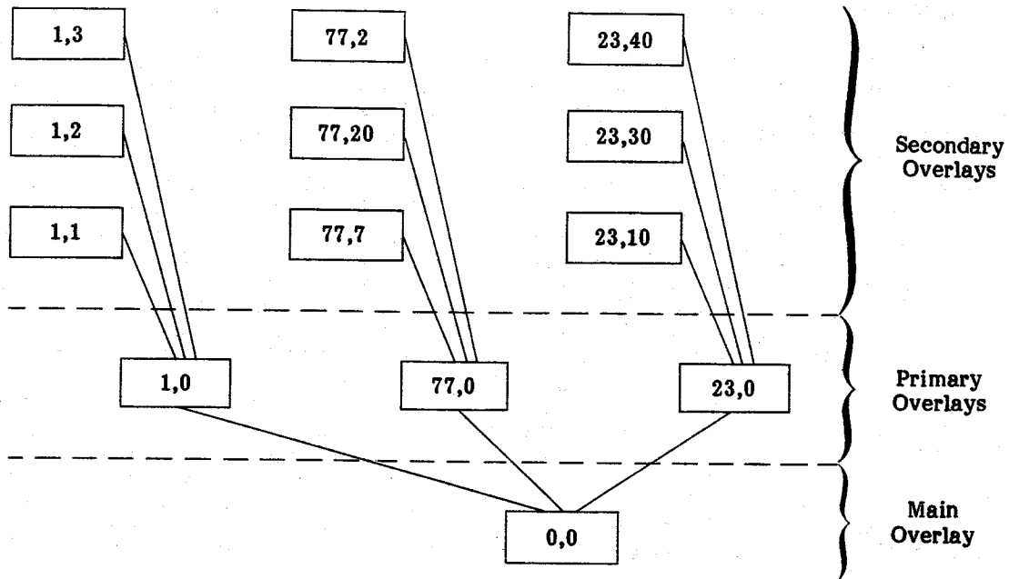
Figure 3-3. Overlay Hierarchy
