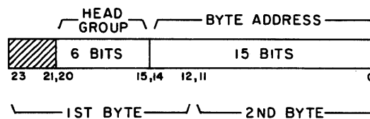
Figure 9. 863 Drum Address Format
