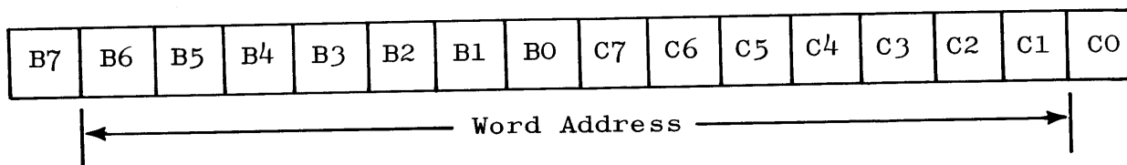
Figure 2-9. B:C Branch Address Format
