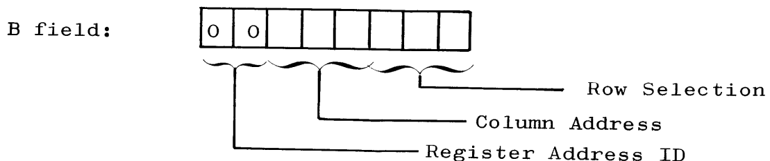
Figure 2-11. Register Address Formats
