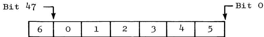
Figure 2-4. Byte Designation
