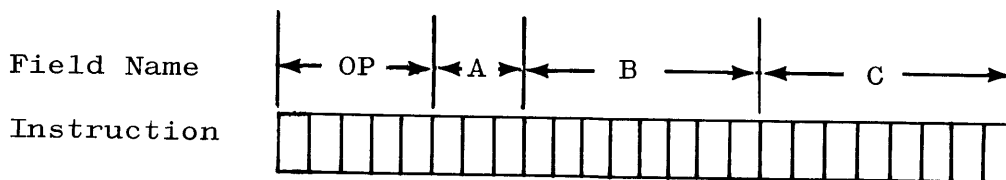
Figure 2-8. Instruction Half-Word Format
