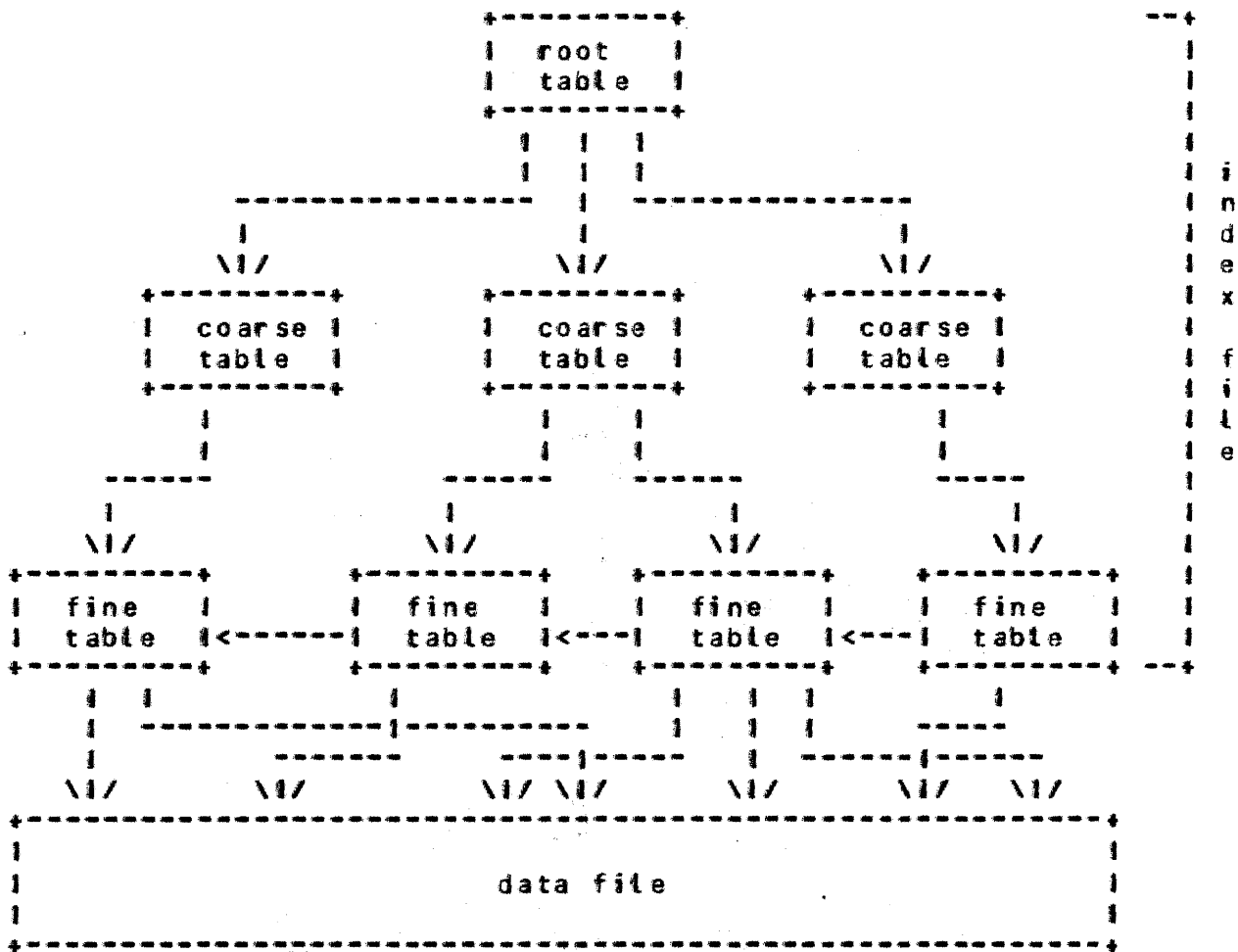
Figure 2 - Index File Organization
