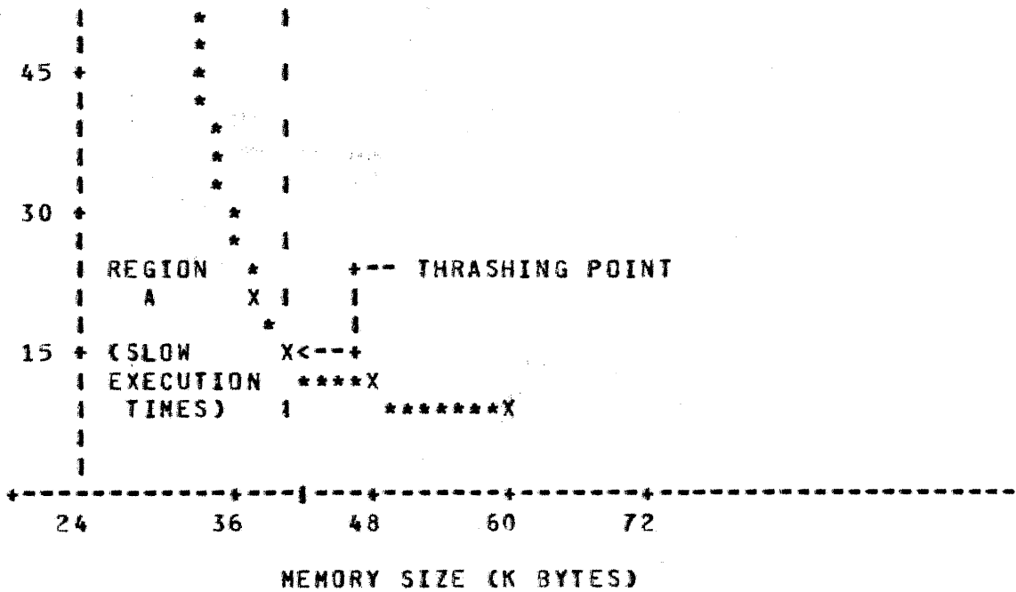
FIGURE 4.1: MEMORY VS EXECUTION TIME EXAMPLE PROGRAM ARM020
