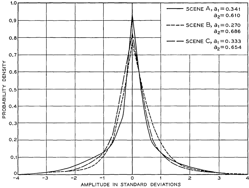
Fig. 10 — Probability density for amplitude of error sequence \{e_i\} for scenes A, B, and C using previous line-and-sample prediction, \hat{S}_0 = a_1s_1 + a_2s_2 . (The values of a_1 and a_2 are chosen to match each scene.)
