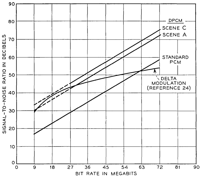
Fig. 15 — Comparison of previous-sample feedback DPCM with standard PCM and delta modulation for monochrome 4.5-Mc/s entertainment television. (Peak-to-peak composite signal to rms quantizing noise in the video is the signal-to-noise ratio shown. The sampling rate is 9 Mc/s.)
