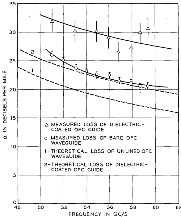
Fig. 3 — Attenuation of coated and uncoated waveguide.
