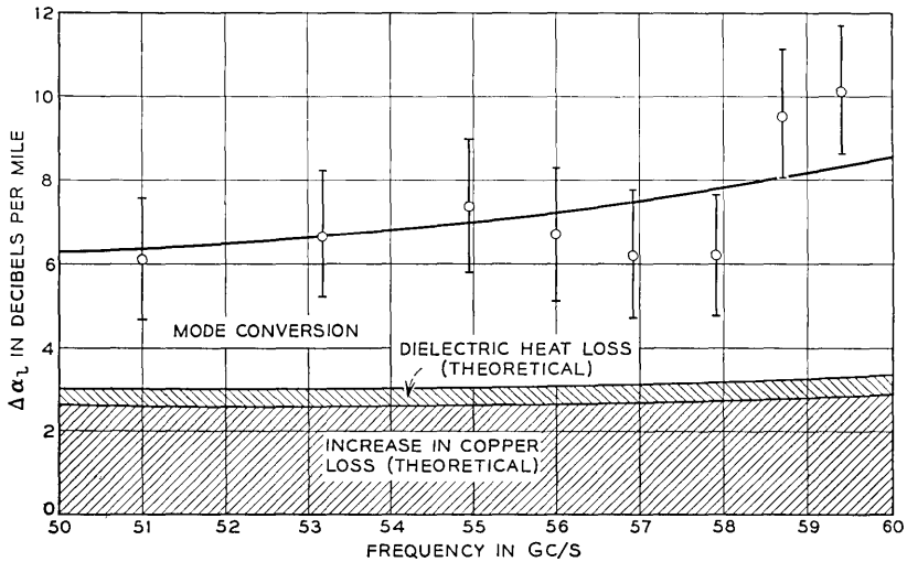
Fig. 4—Increase in attenuation \Delta\alpha_i of 0.875-inch i.d. copper waveguide due to linear.
