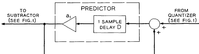
Fig. 4 — Previous-sample predictor.
