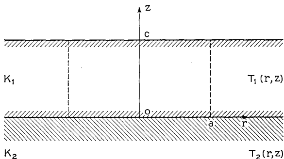
Fig. 1 — Cross section of plane film on semi-infinite substrate.
