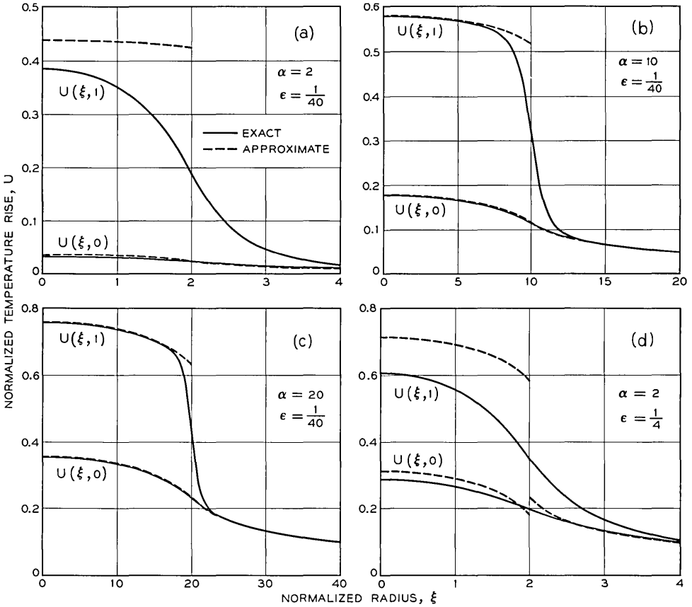
Fig. 4 — Normalized temperature rise at upper and lower surfaces of film: (a) \alpha = 2, \epsilon = 1/40 ; (b) \alpha = 10, \epsilon = 1/40 ; (c) \alpha = 20, \epsilon = 1/40 ; (d) \alpha = 2, \epsilon = 1/4 .
