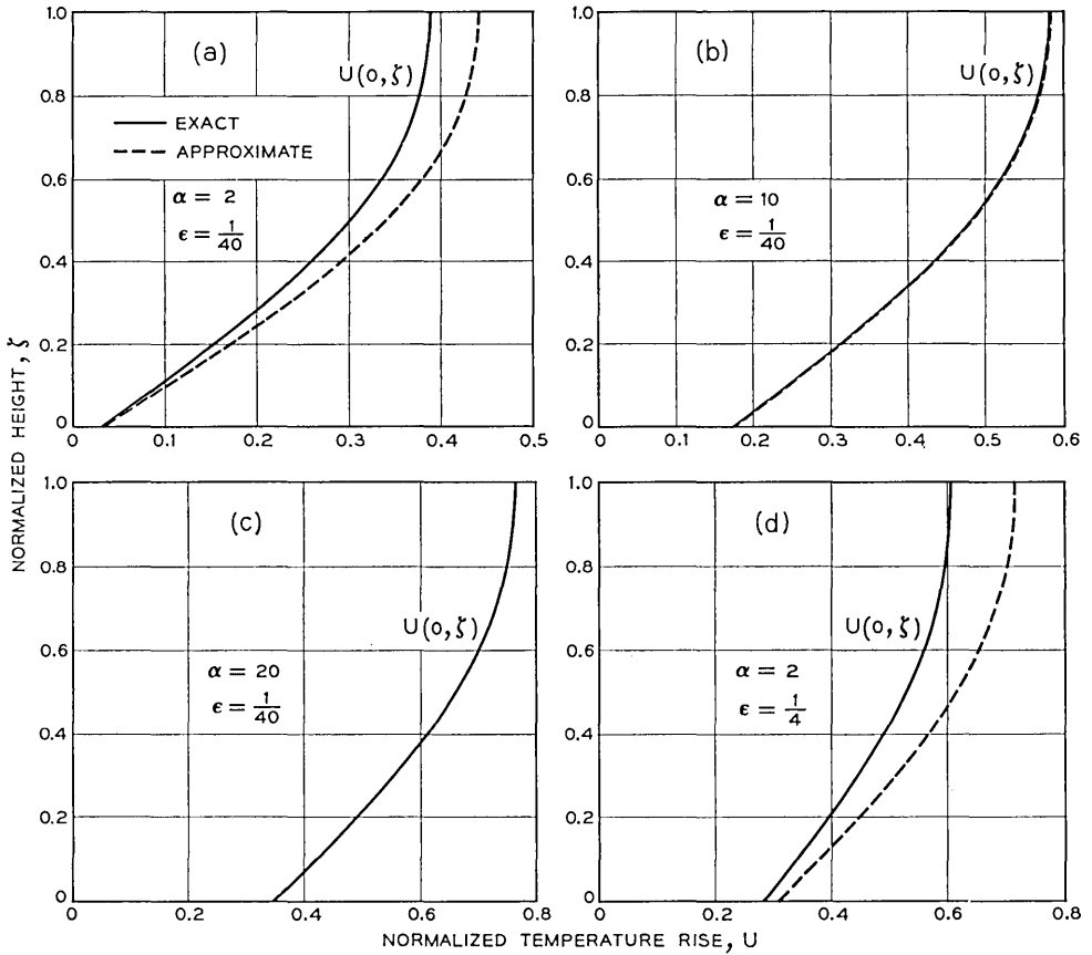
Fig. 5 — Normalized temperature rise along axis: (a) \alpha = 2, \epsilon = 1/40 ; (b) \alpha = 10, \epsilon = 1/40 ; (c) \alpha = 20, \epsilon = 1/40 ; (d) \alpha = 2, \epsilon = 1/4 .
