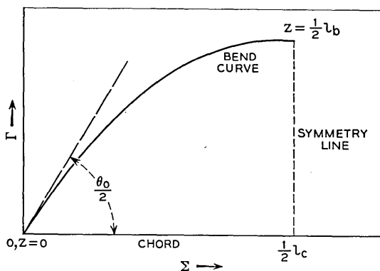
Fig. 5 — Coordinate system for half of the bend.
