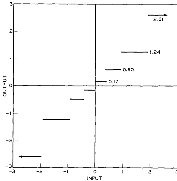
Fig. 11 — Typical 8-level exponential quantizer characteristic obtained from (21). (Case shown is for m = 5.5 and V = 7 .)
