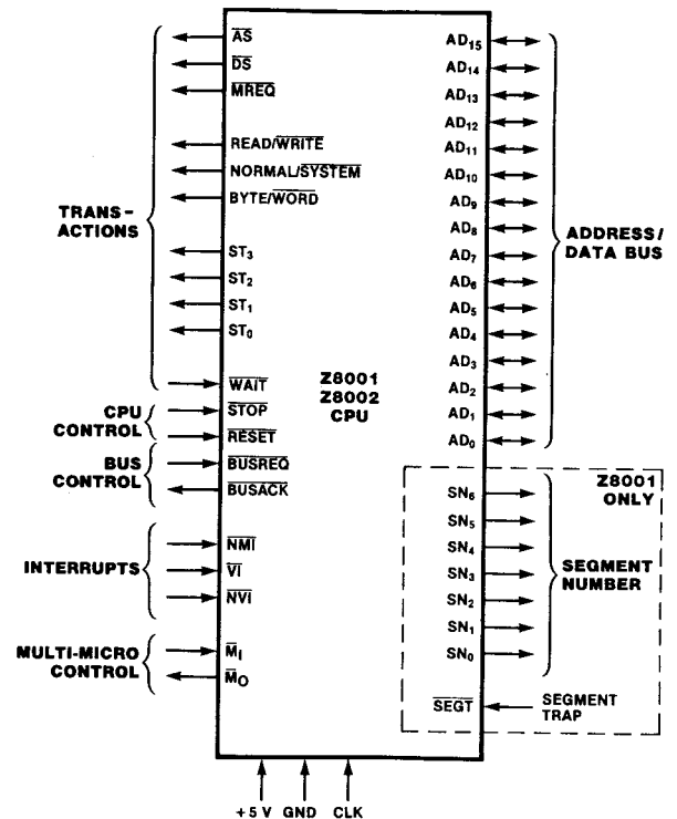
Figure 9-1. Pin Functions
