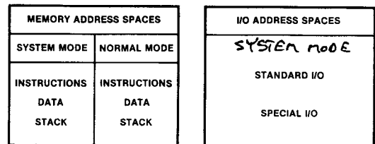
Figure 3-1. Address Spaces on the Z8001 and Z8002
