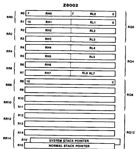
Figure 2-5b. Z8002 General-Purpose Registers (Registers Address Space)
