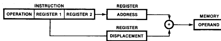
THE OPERAND VALUE IS THE CONTENTS OF THE LOCATION WHOSE ADDRESS IS THE CONTENTS OF THE ONE REGISTER OFFSET BY THE DISPLACEMENT IN THE SECOND REGISTER.
