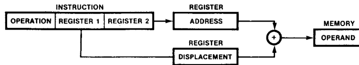
THE OPERAND VALUE IS THE CONTENTS OF THE LOCATION WHOSE ADDRESS IS THE CONTENTS OF THE ONE REGISTER OFFSET BY THE DISPLACEMENT IN THE SECOND REGISTER.
