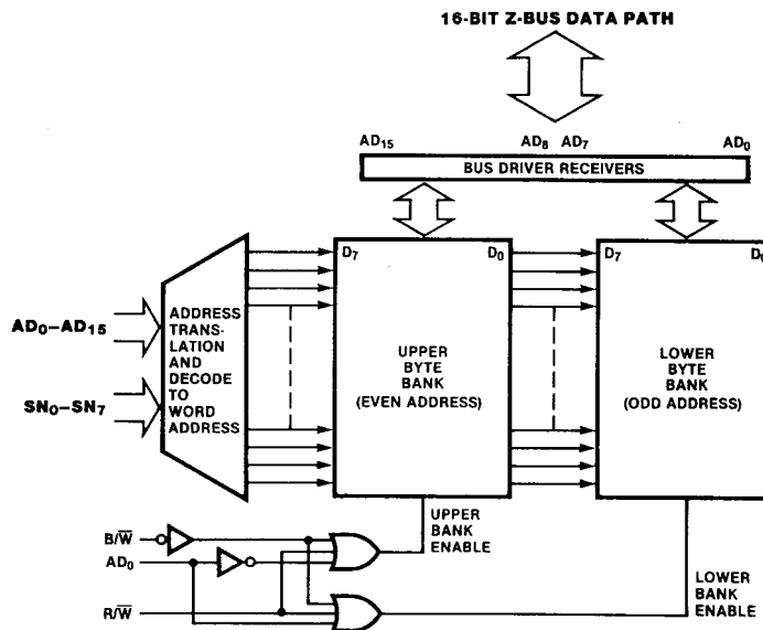
Figure 9-4. Memory Organization
