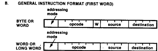
Figure 2-7. Instruction Formats
