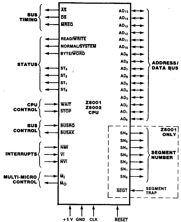
Figure 2-3. Z8000 Pin Functions
