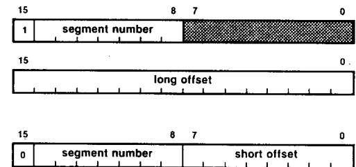
Figure 5-2. Segmented Memory Address Within Instruction.
