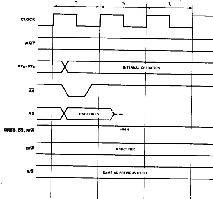
Figure 9-7. Internal Operation Timing
