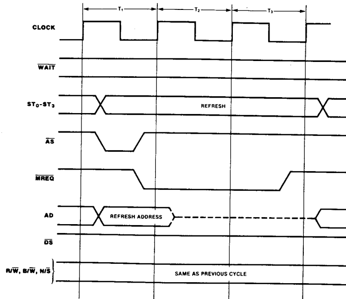
Figure 9-8. Memory Refresh Timing
