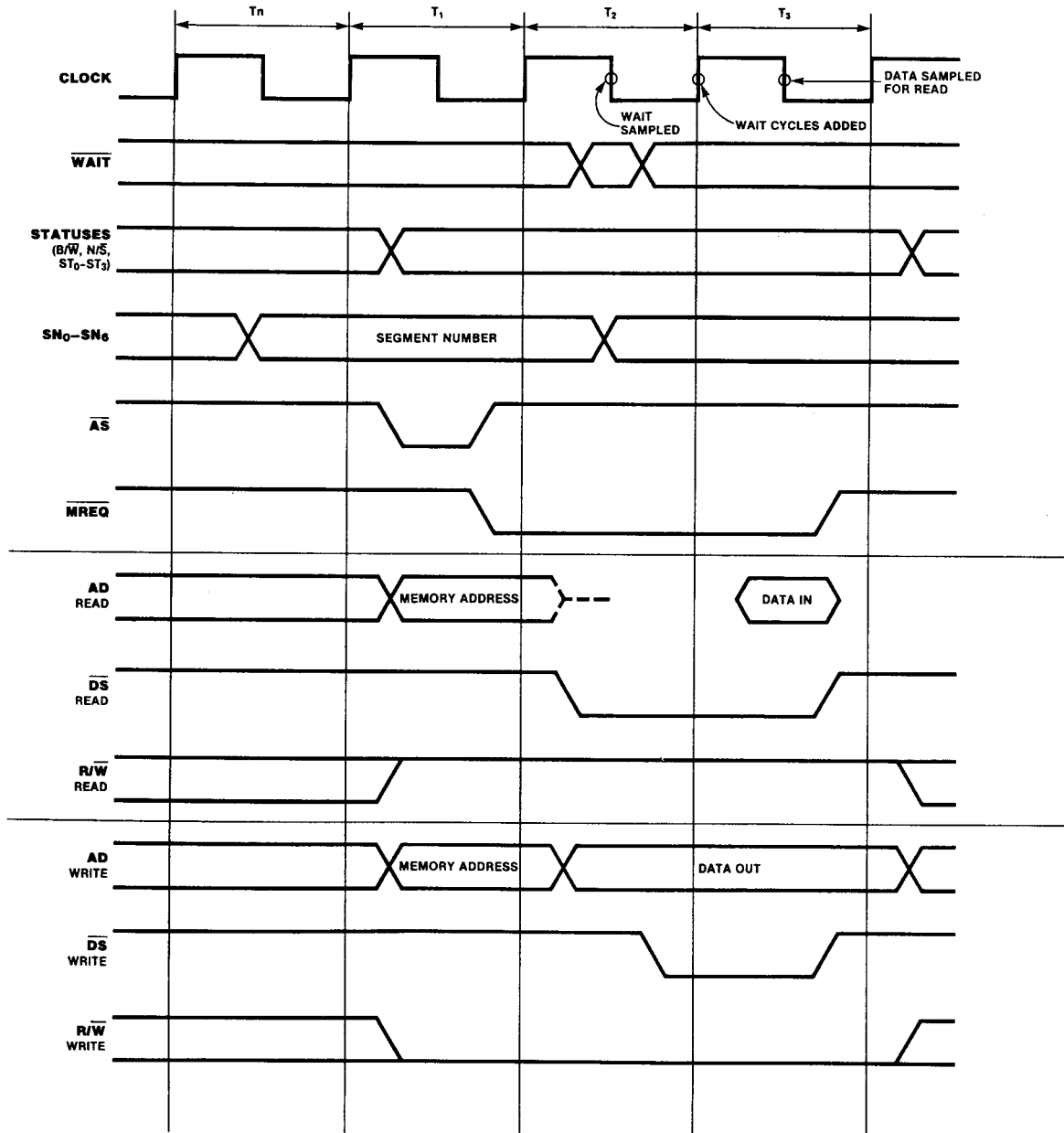
Figure 9-3. Memory Read and Write Transaction
