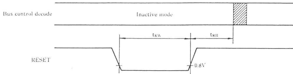
Fig. 3 Reset timing
