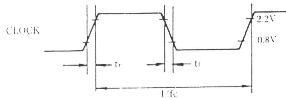
Fig. 1 Clock timing
