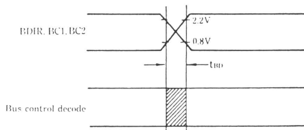
Fig. 2 Bus control timing
