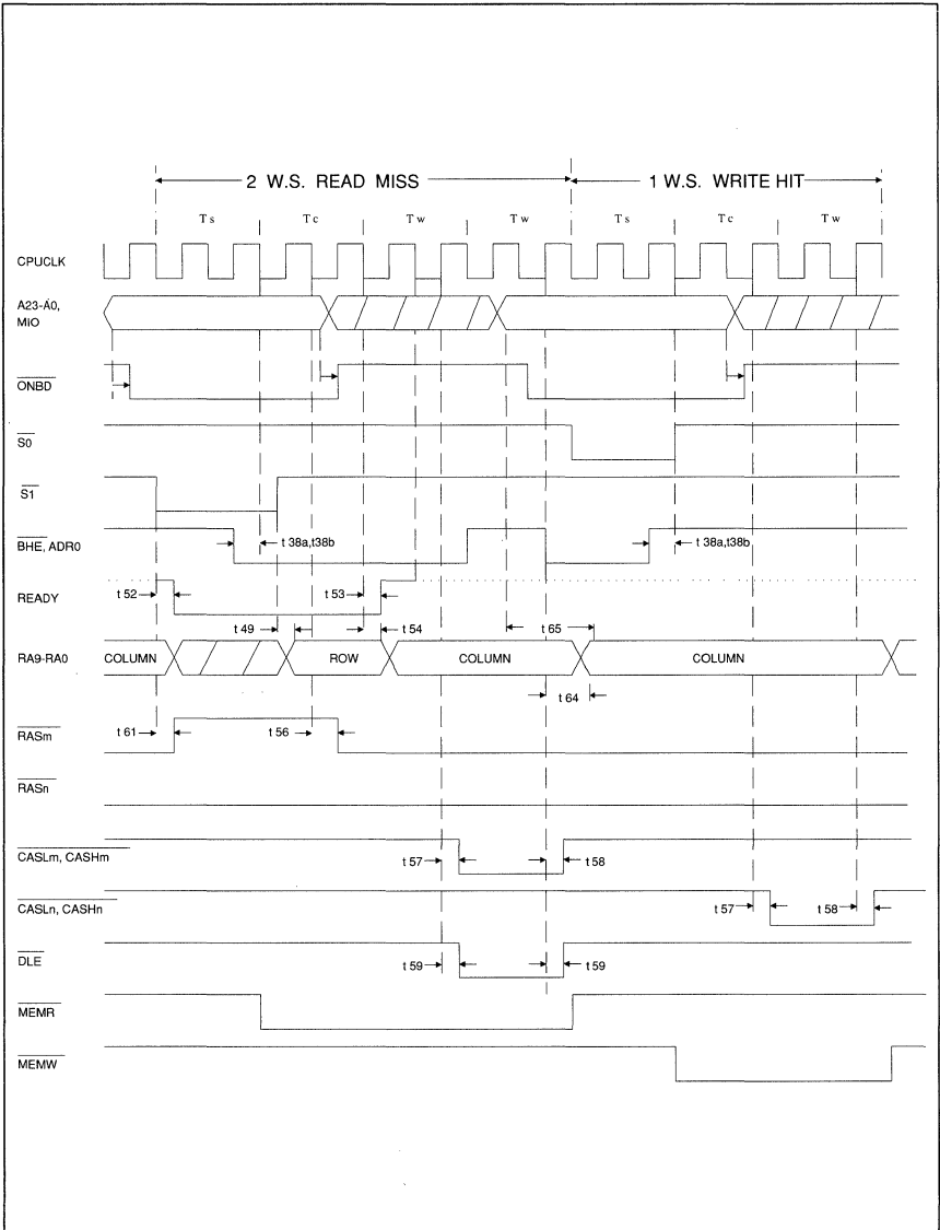
Figure 12. Memory Mode 2 (PAGE) 2 OF 2
