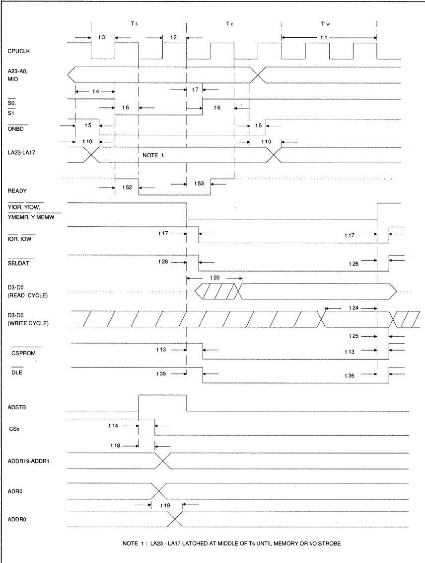
Figure 6. Basic Timing
