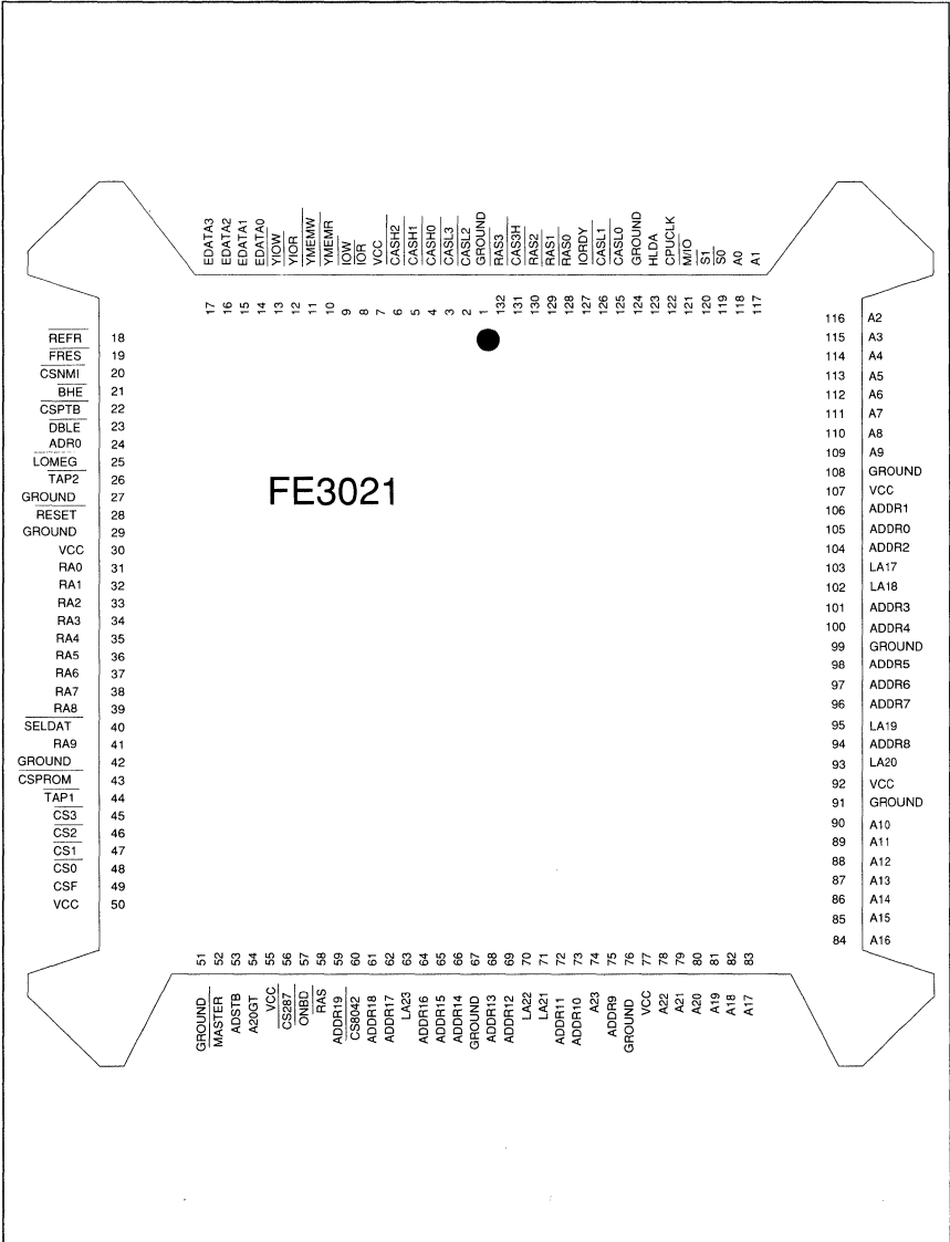
Figure 2. FE3021 Pin Assignment Information
