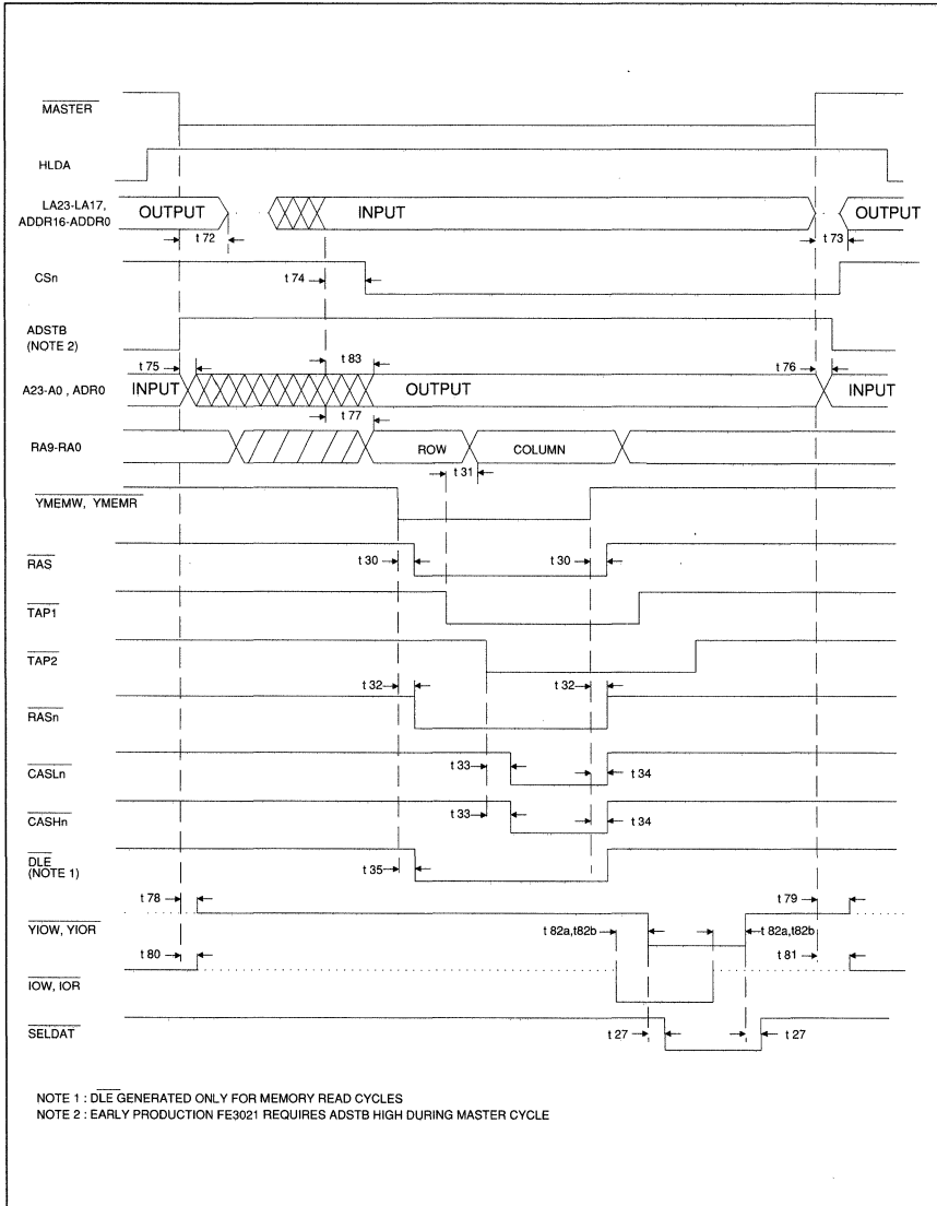
Figure 17. Bus Master Cycle
