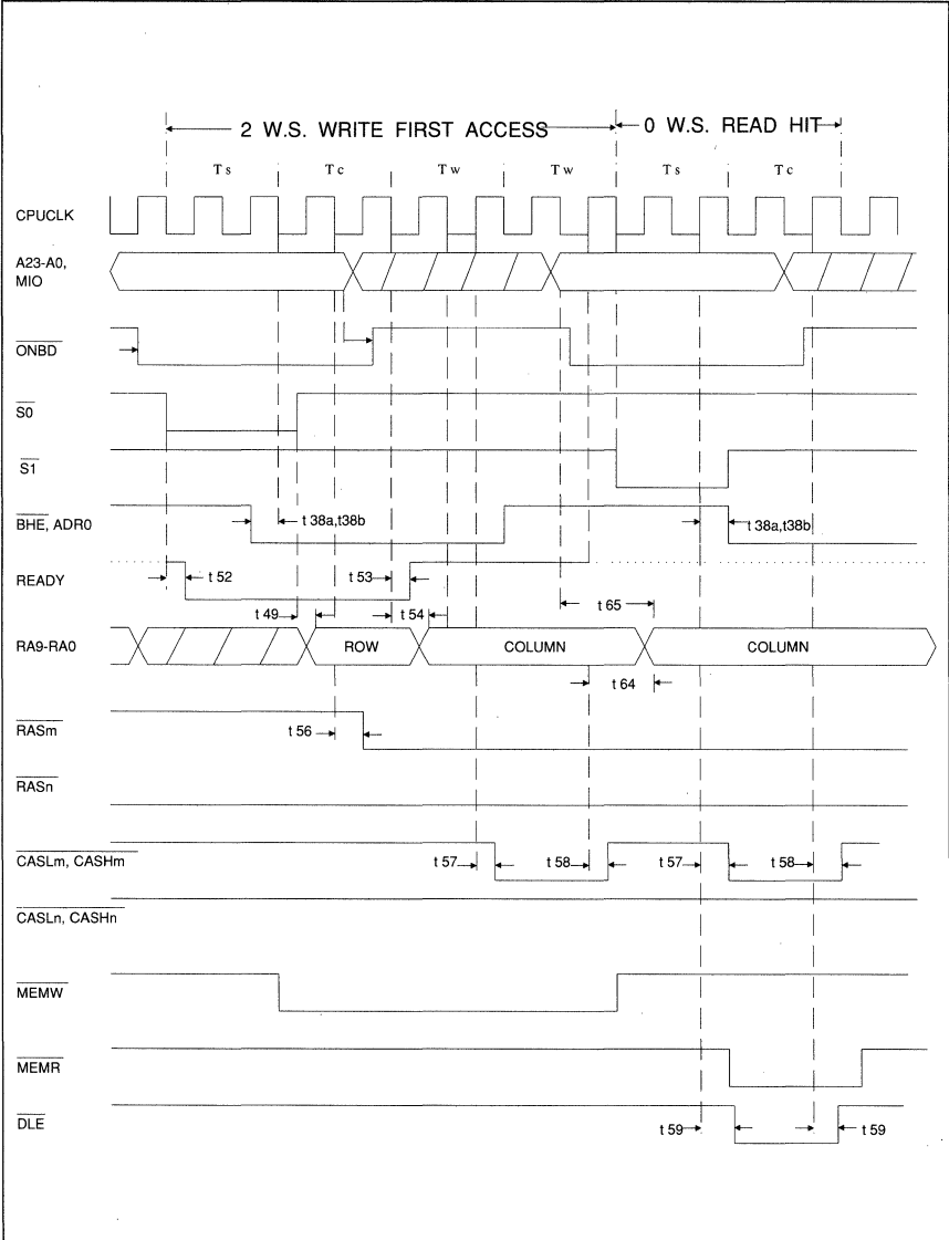
Figure 11. Memory Mode 2 (PAGE) 1 OF 2
