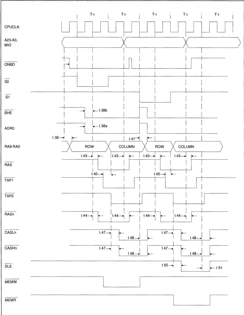
Figure 15. Memory Mode 5 (Non-Page) 0 WS Read & Write
