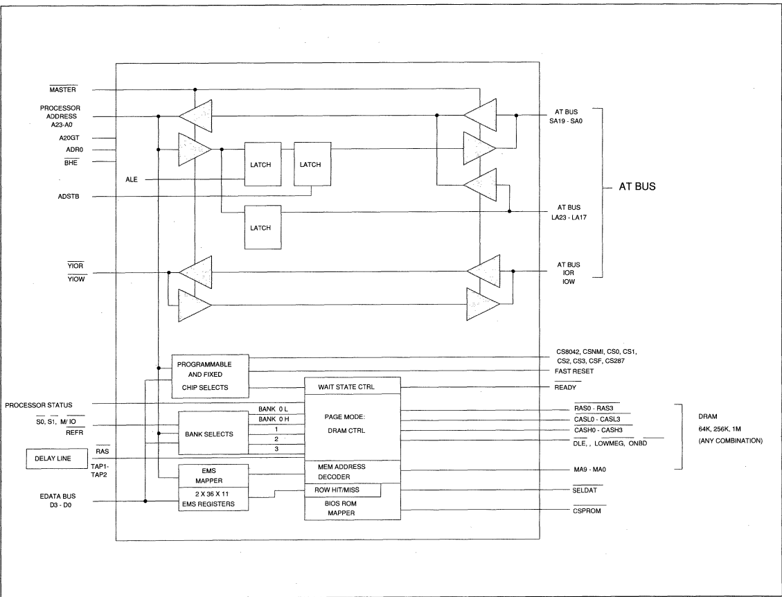
Figure 3. FE3021 Functional Block Diagram
