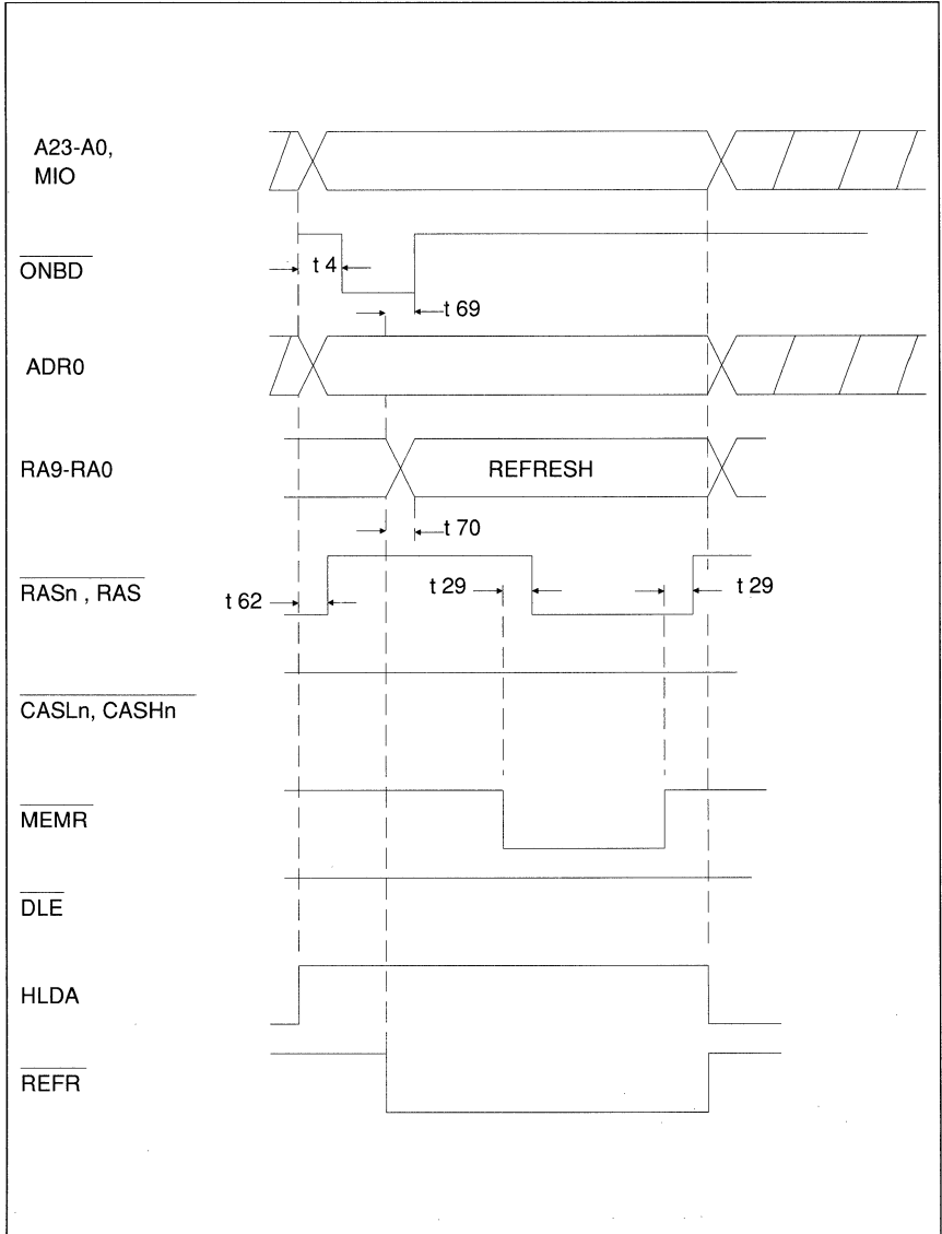
Figure 16. Refresh Cycle
