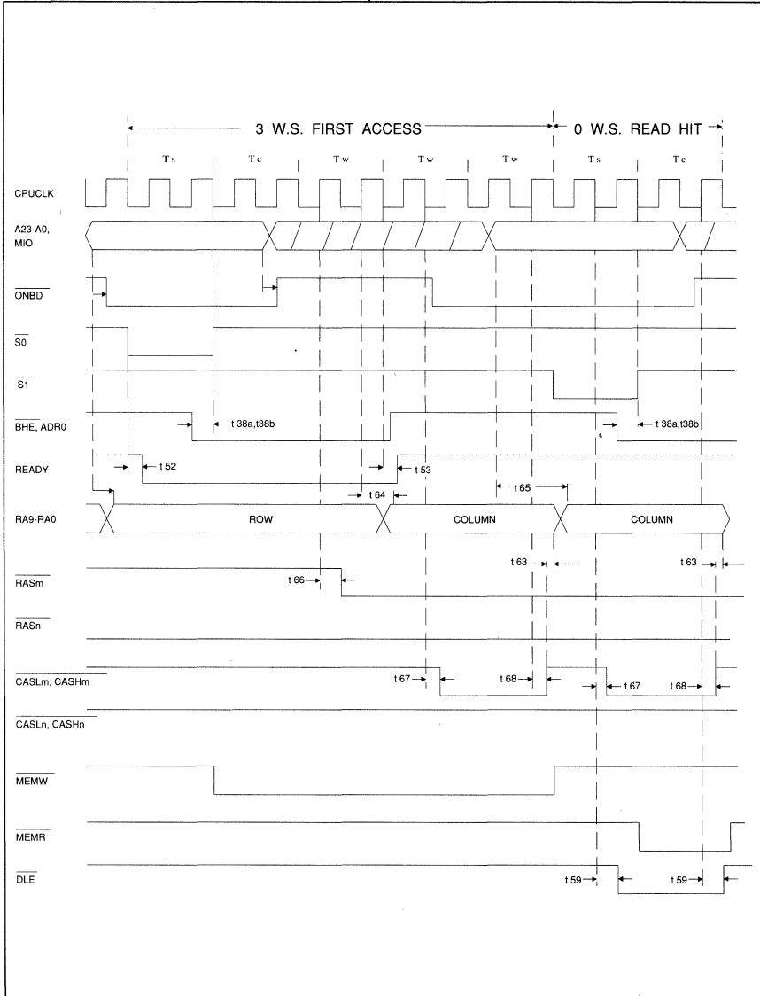
Figure 13. Memory Mode 3 (PAGE) 1 OF 2
