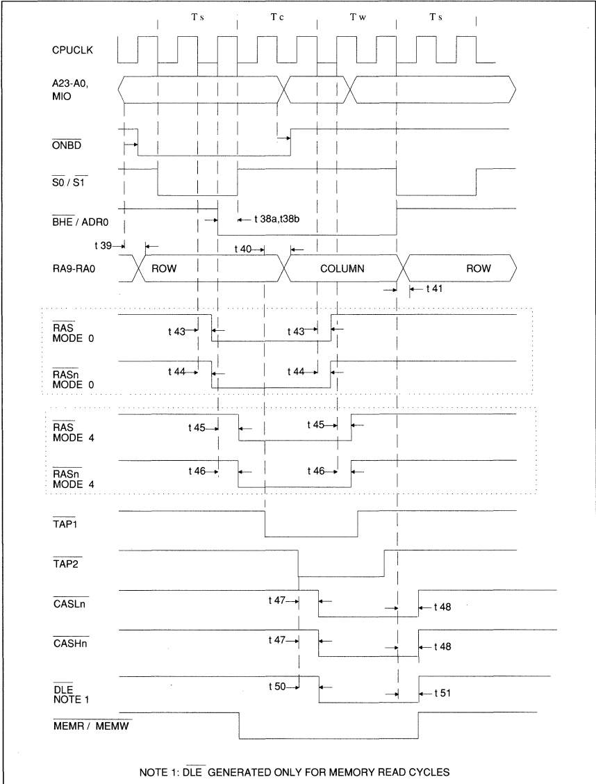
Figure 9. Memory Modes 0 & 4 (Non-page Mode)
