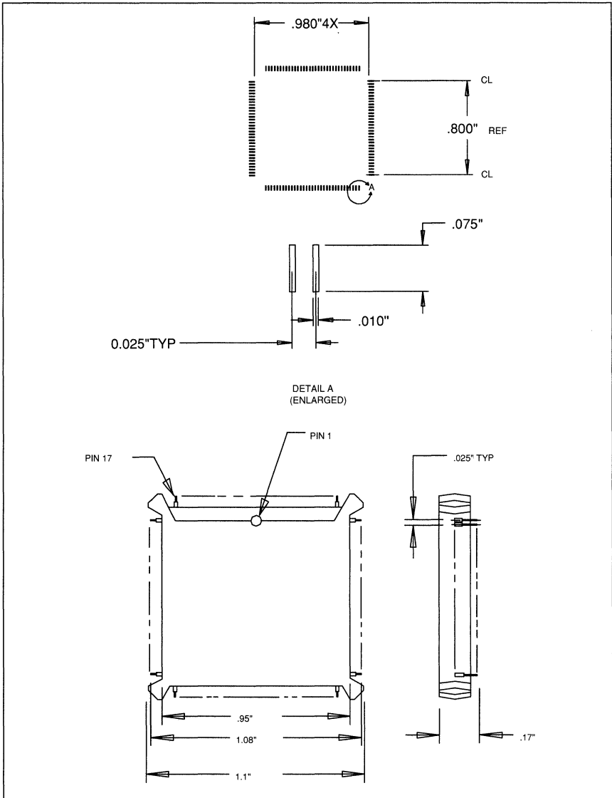
Figure 18. 132-Pin JEDEC Flat Pack Packaging Diagram
