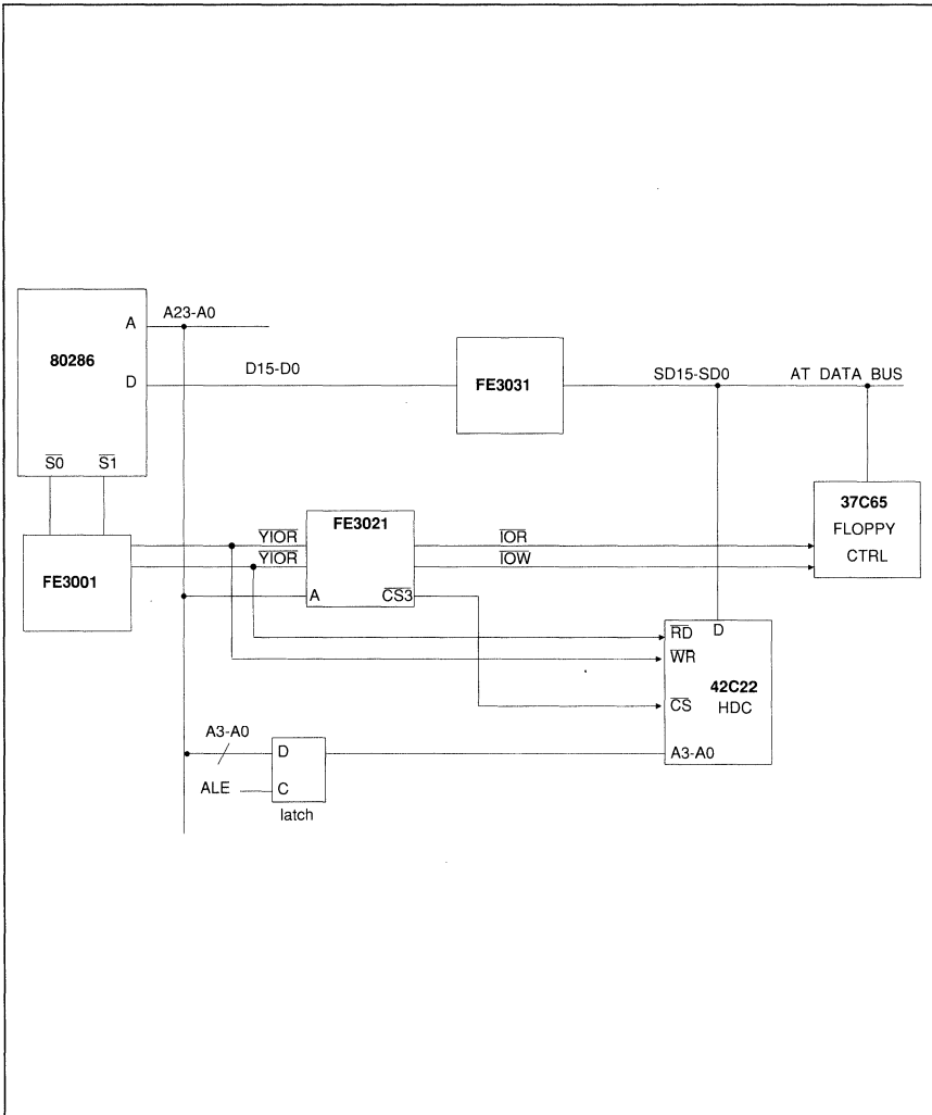
Figure 4. High Speed HDC Configuration
