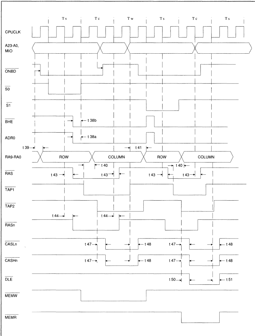
Figure 10. Memory Mode 1 (Non-Page 0 WS Read/1 WS Write)
