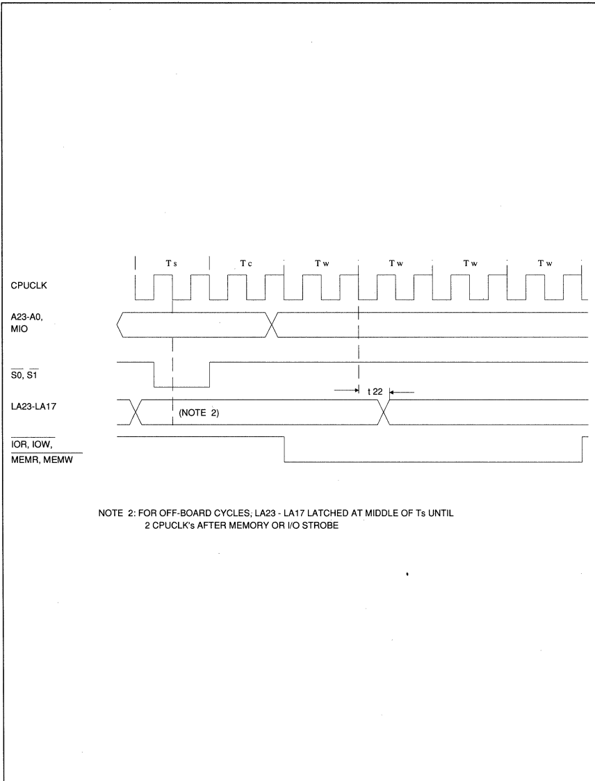
Figure 7. High Speed Mode LA23-LA17 Timing
