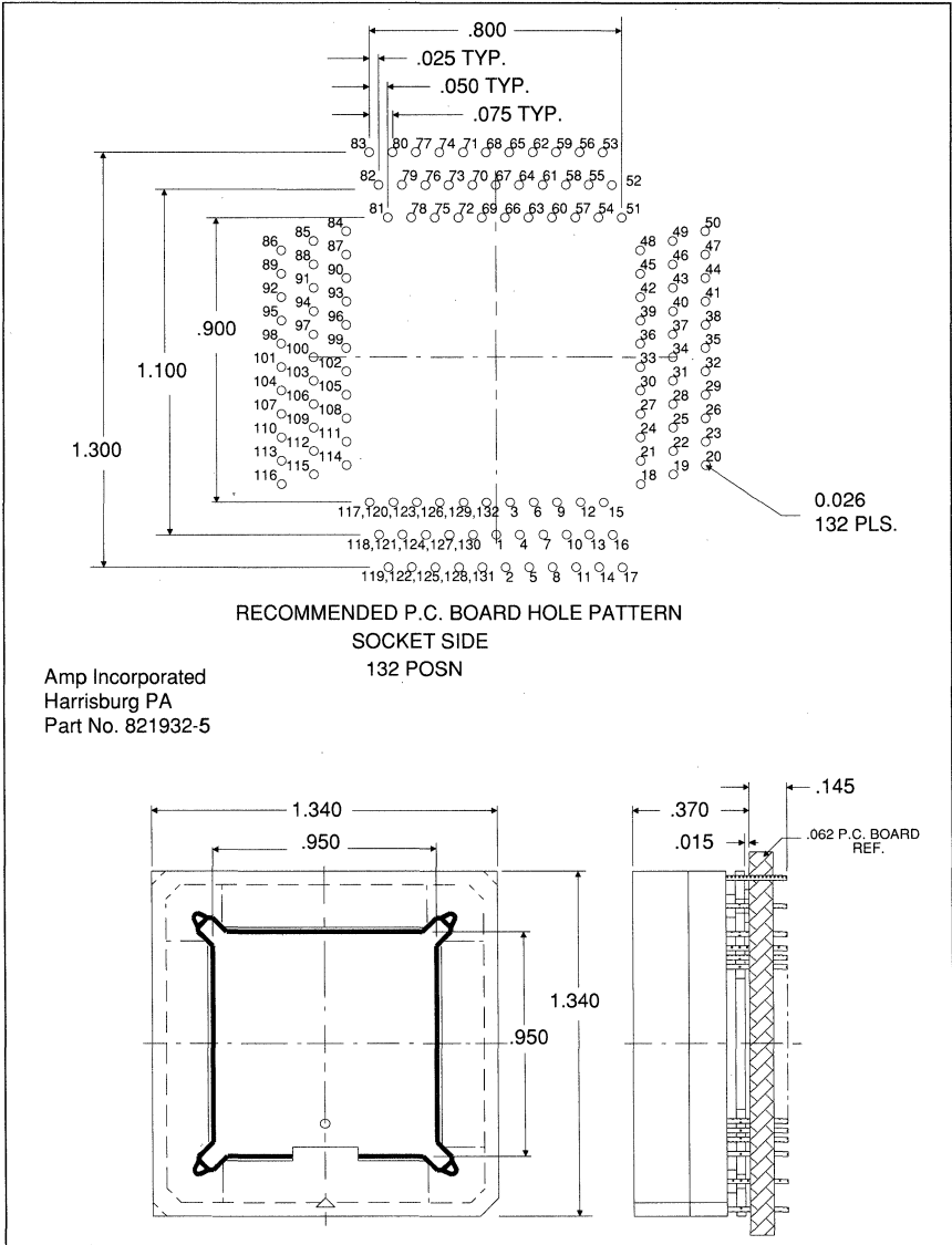
Figure 19. Socket Diagram
