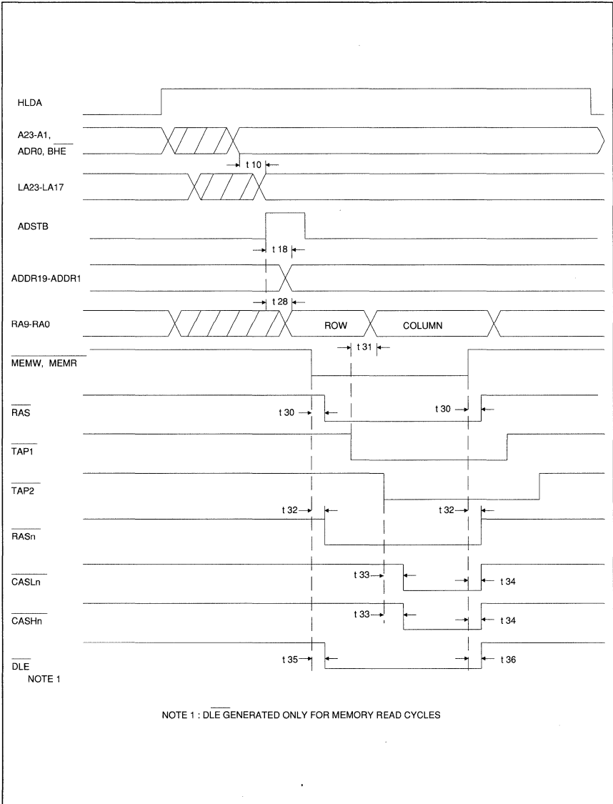
Figure 8. DMA Memory Cycle
