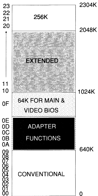
Figure 5. EMS Memory Map Configurations
