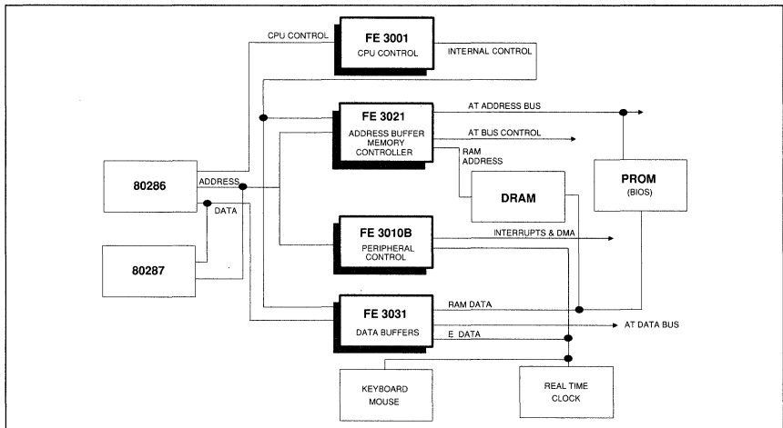
Figure 1. FE3600B Chip Set Functional Block Diagram
