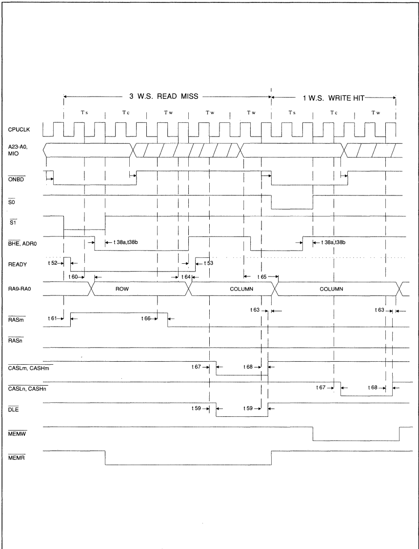
Figure 14. Memory Mode 3 (PAGE) 2 OF 2
