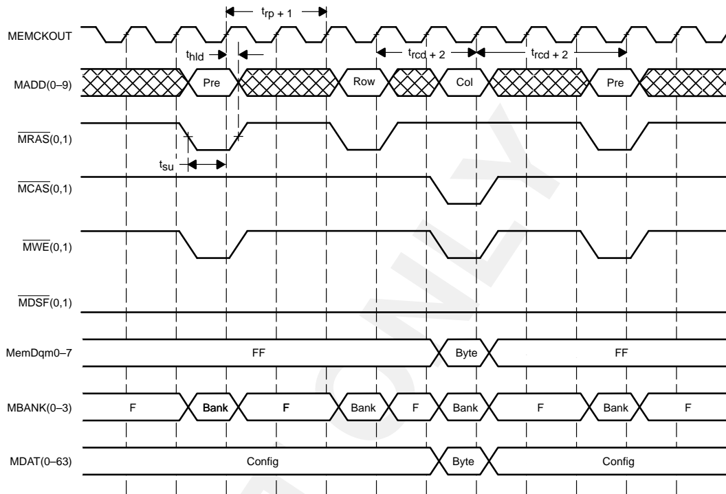
Figure 4-13. RAS Minimum Access Timing
