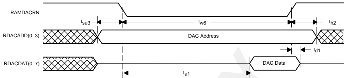
Figure 4-4. DAC Read Timing
