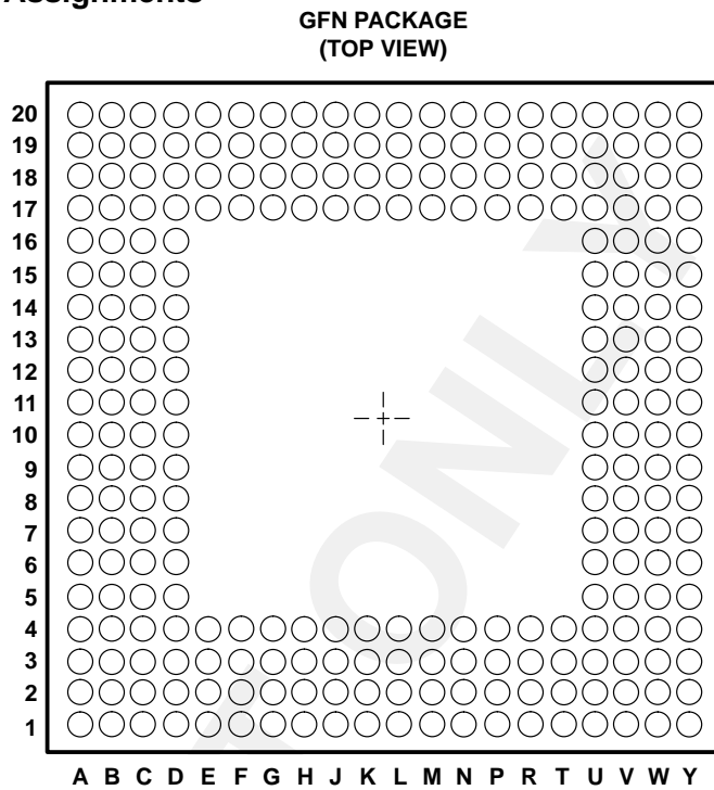
Figure 1-2. Terminal Assignments
