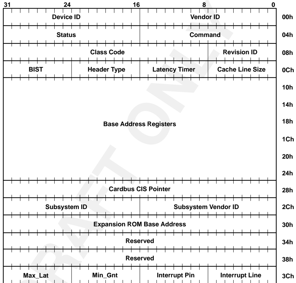
Figure 2-1. PCI Configuration Region
