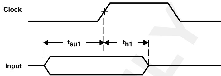
Figure 4-1. Input Timing Parameters
