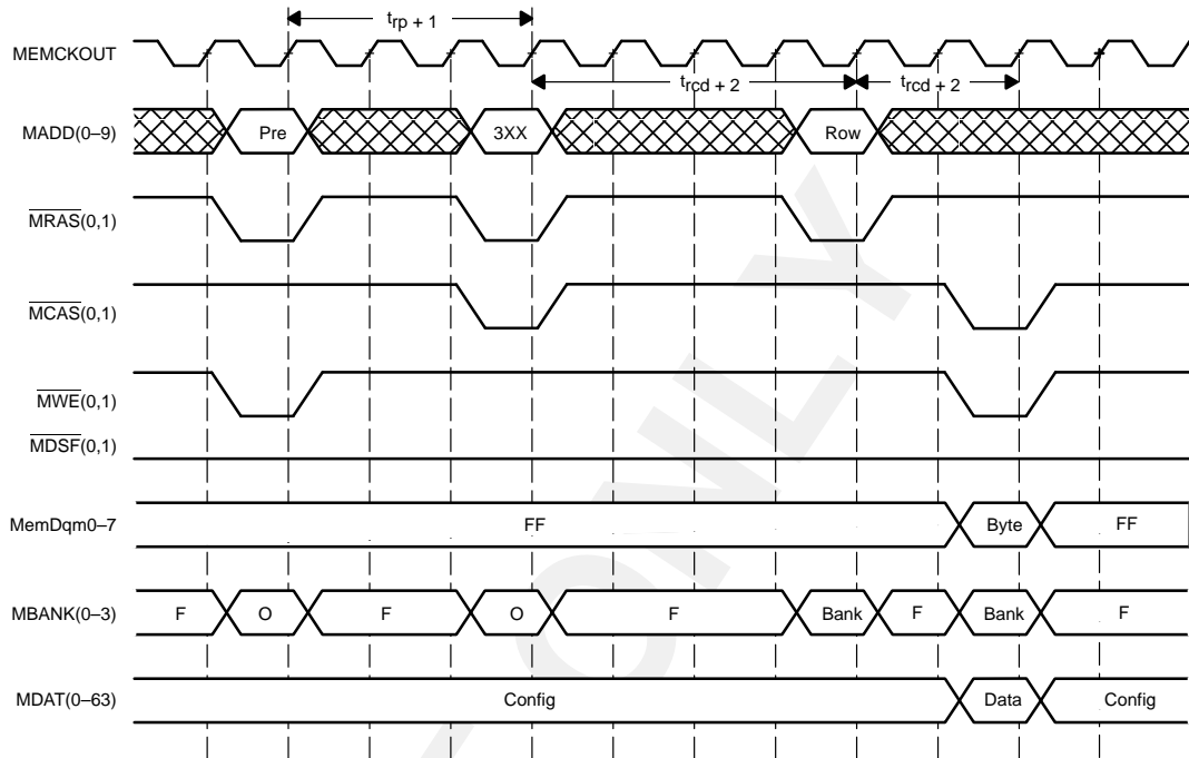
Figure 4-11. Refresh Followed by Access Timing
