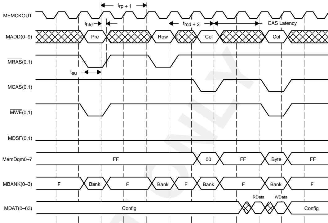
Figure 4-15. Read Followed by Write - No Dead Cycle Timing
