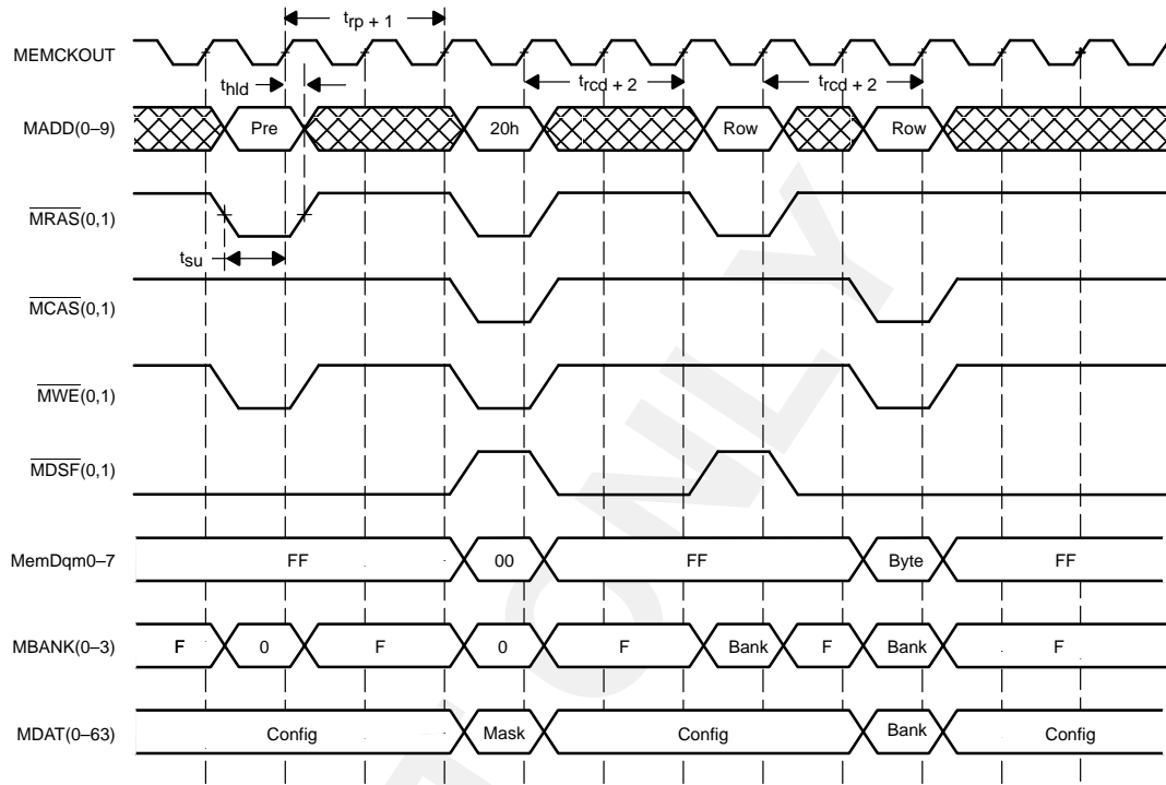
Figure 4-14. Mask Load Followed by Masked Write Timing
