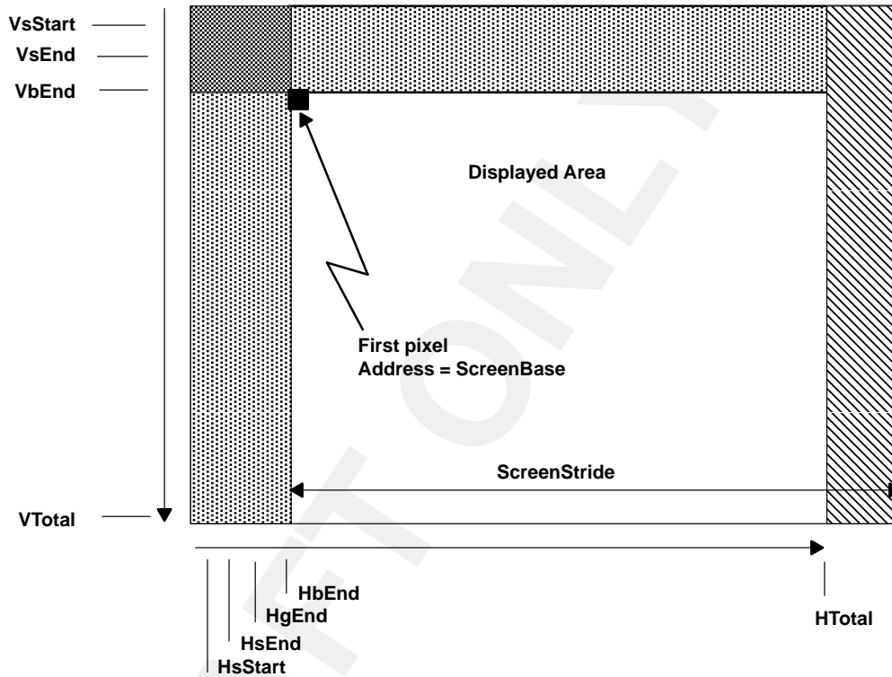
Figure 2-3. Video Timing Parameters
