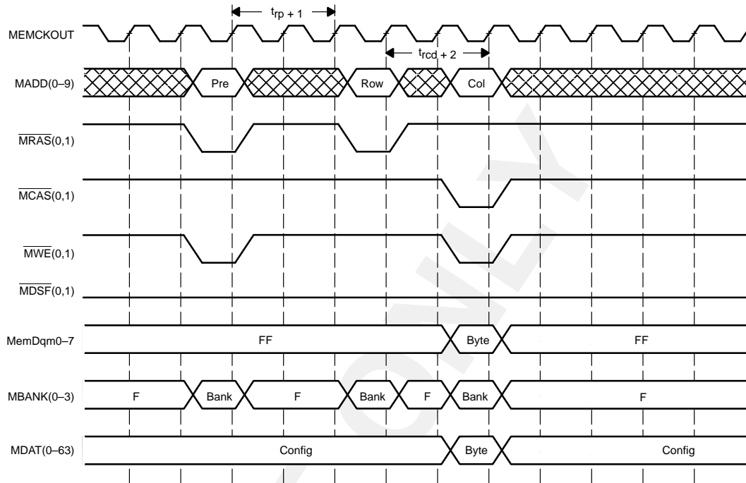
Figure 4-9. Single Write with Precharge Timing
