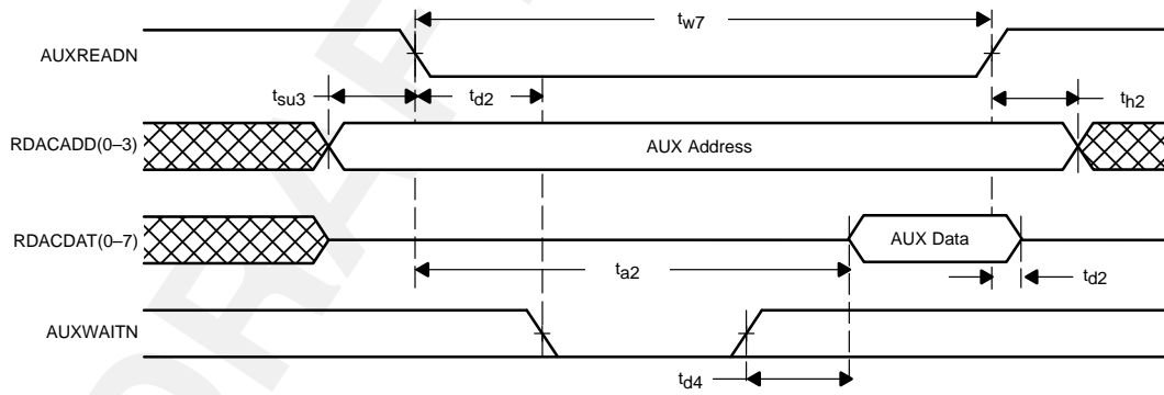
Figure 4-6. AUX Read Timing
