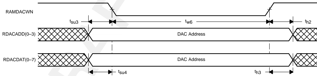
Figure 4-3. DAC Write Timing
