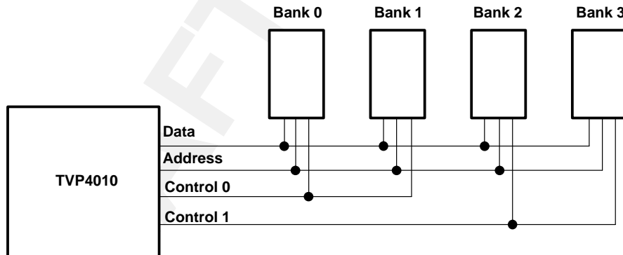
Figure 2–2. Organization of Memory Devices
