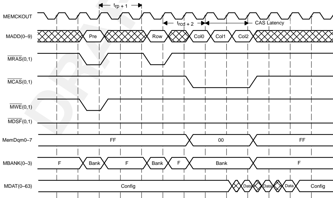
Figure 4-7. Single Read with Precharge Timing
