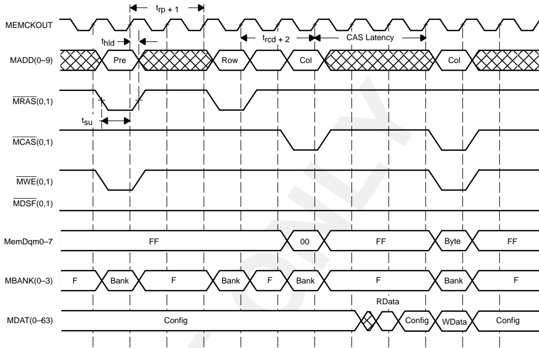
Figure 4-16. Read Followed by Write - With Dead Cycle Timing
