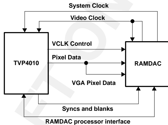
Figure 5–1. Typical RAMDAC Organization
