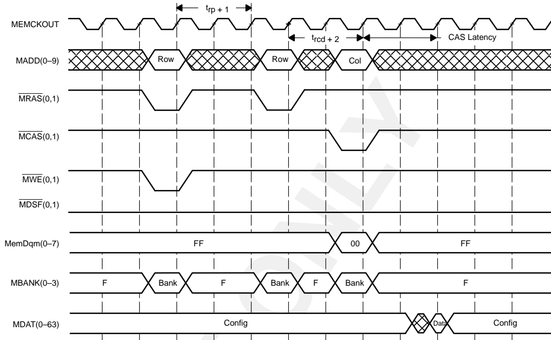
Figure 4-7. Single Read with Precharge Timing
