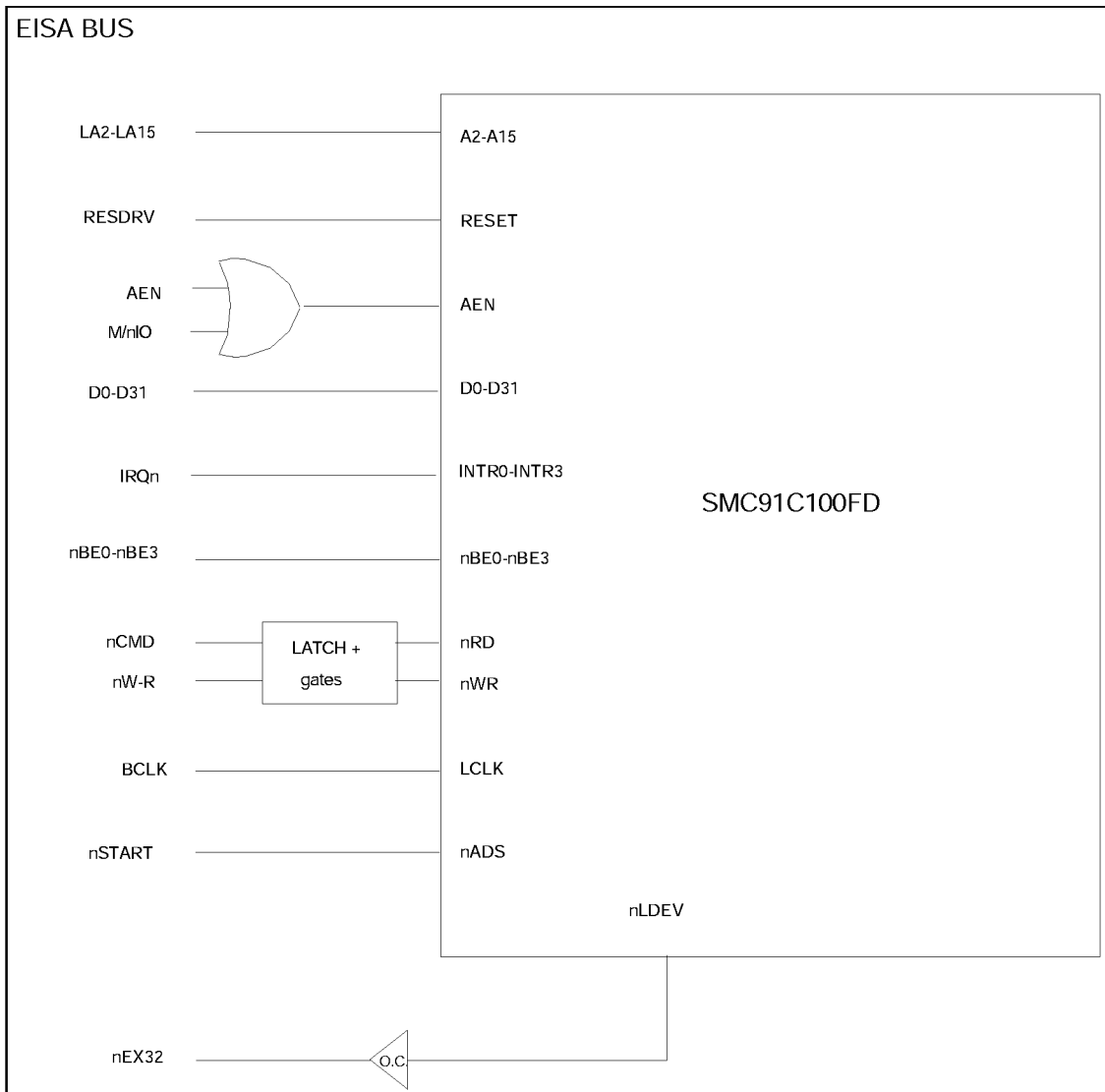
FIGURE 15 - SMC91C100FD ON EISA BUS
