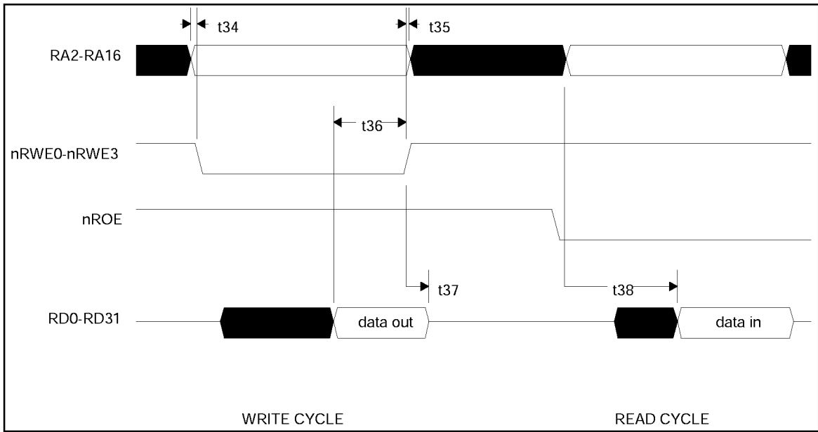
FIGURE 24 - SRAM INTERFACE
