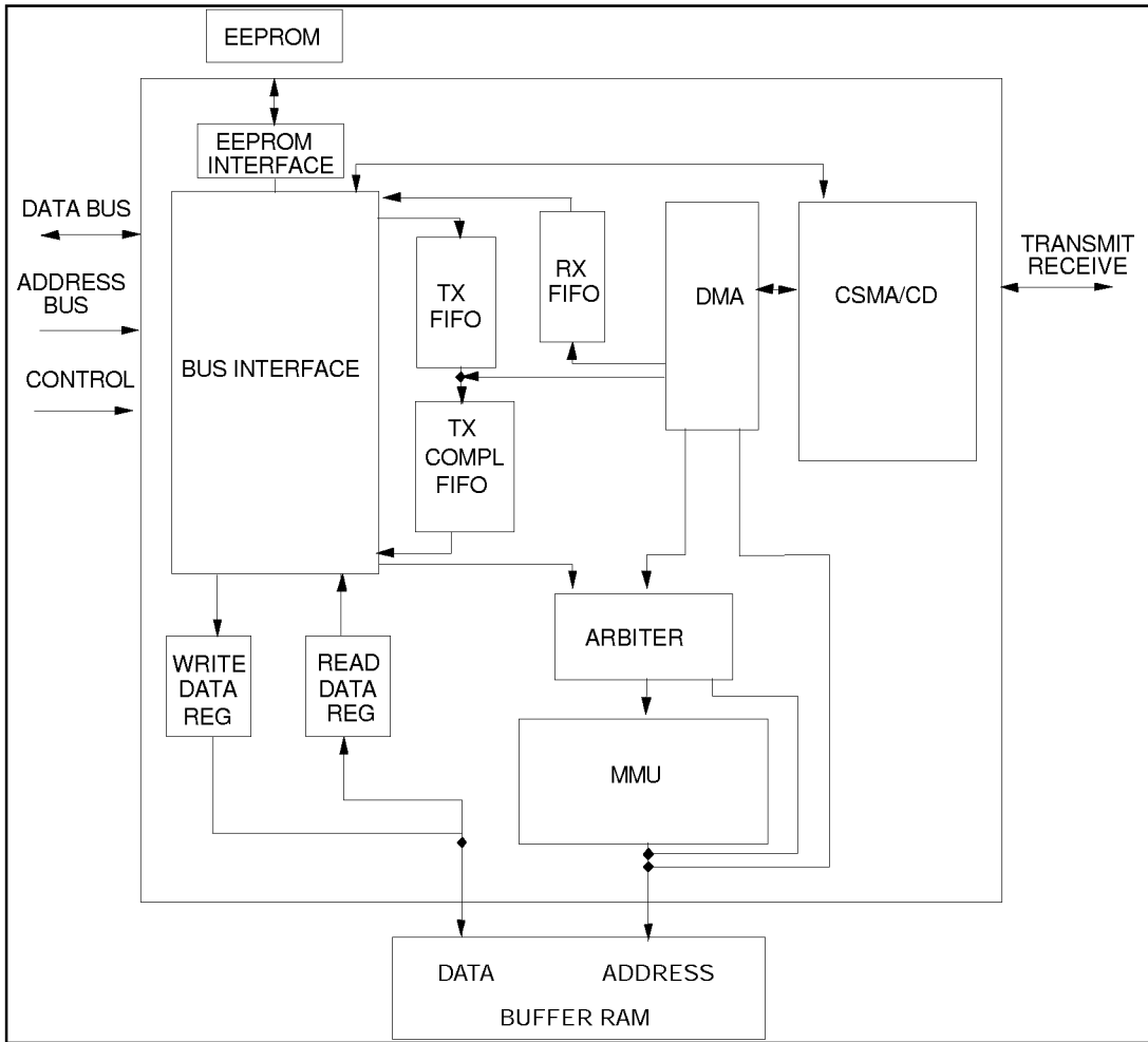
FIGURE 3 - SMC91C100FD INTERNAL BLOCK DIAGRAM WITH DATA PATH
