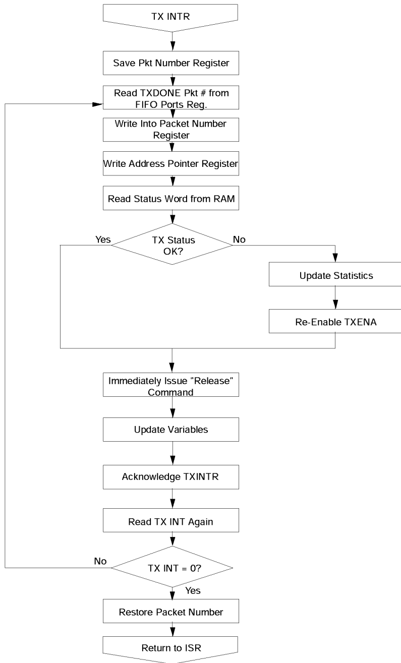
FIGURE 8 - TX INTR
