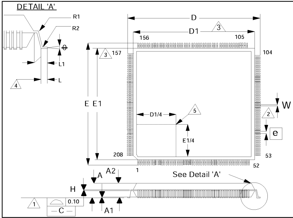
FIGURE 27 - 208 PIN QFP PACKAGE OUTLINES
