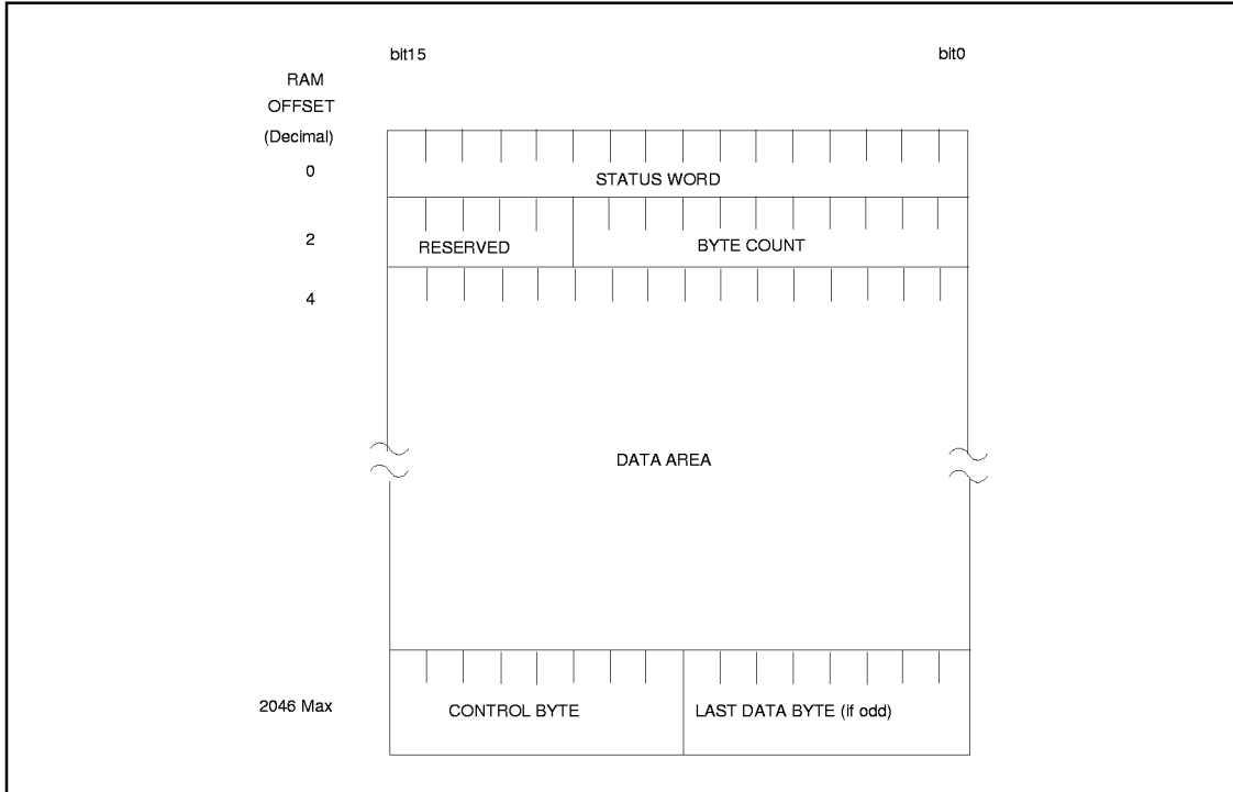
FIGURE 4 - DATA PACKET FORMAT
