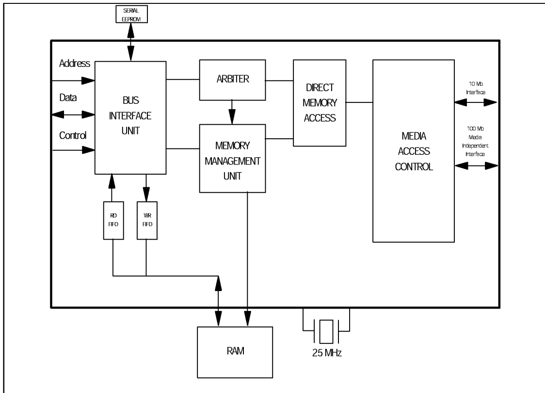
FIGURE 1 - SMC91C100FD BLOCK DIAGRAM
