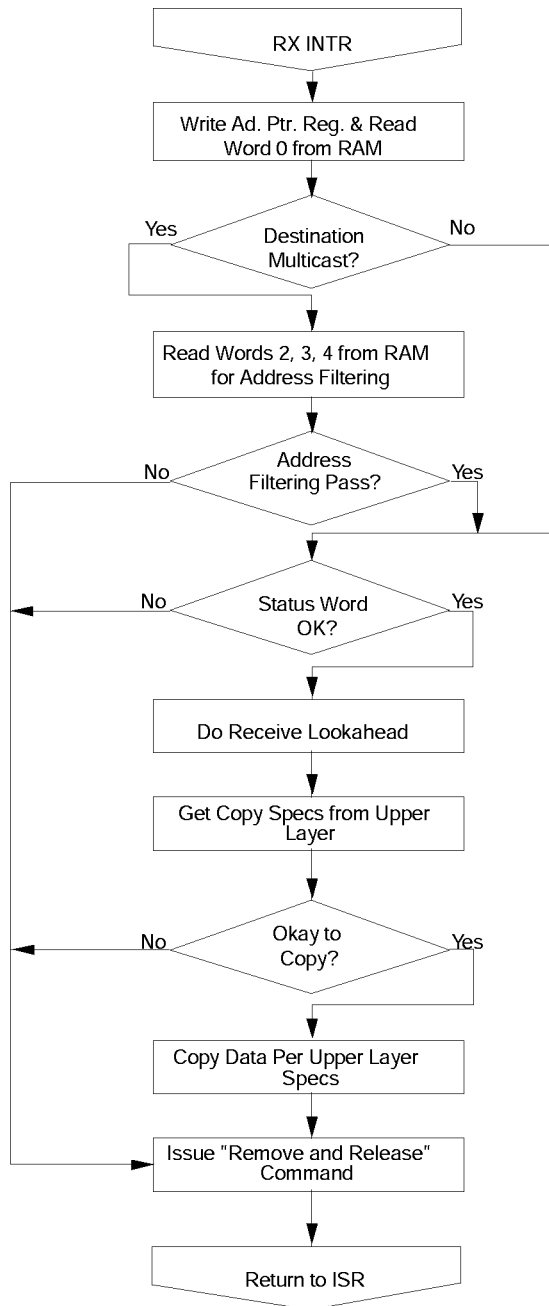
FIGURE 7 - RX INTR
