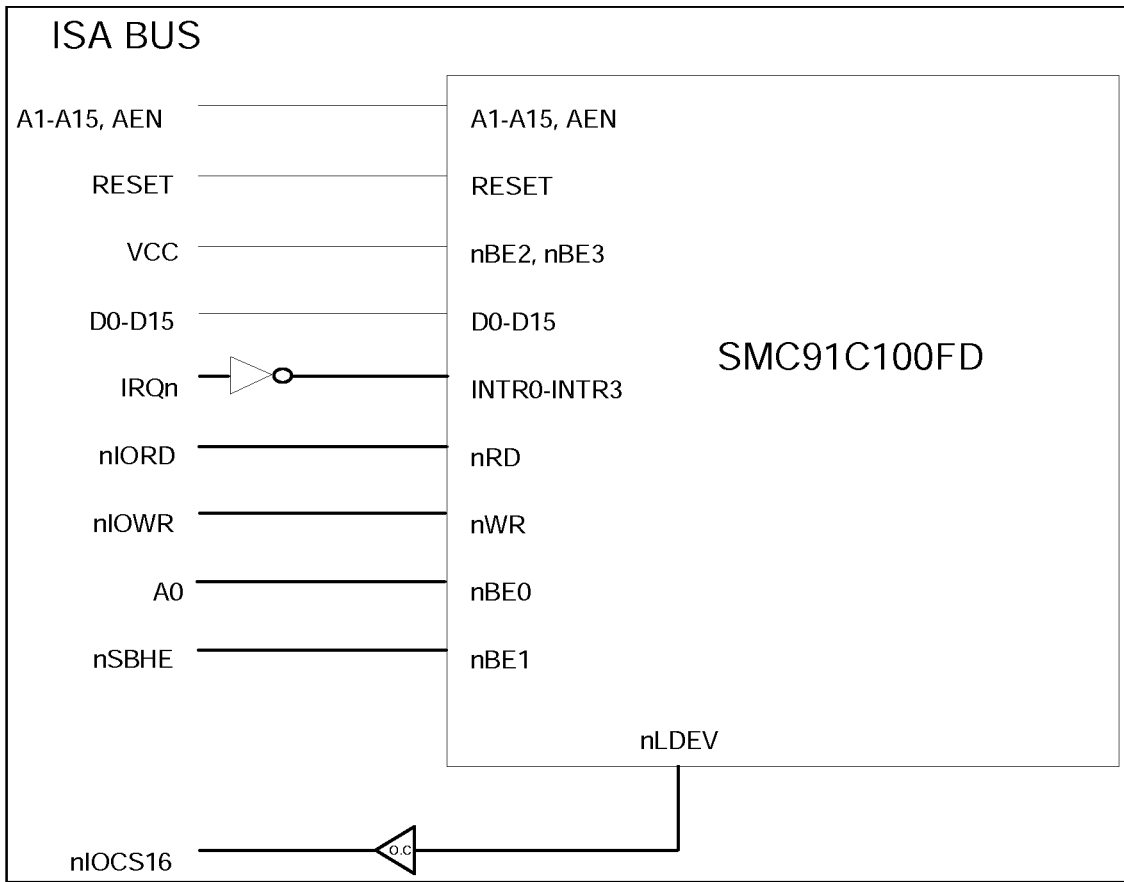
FIGURE 14 - SMC91C100FD ON ISA BUS
