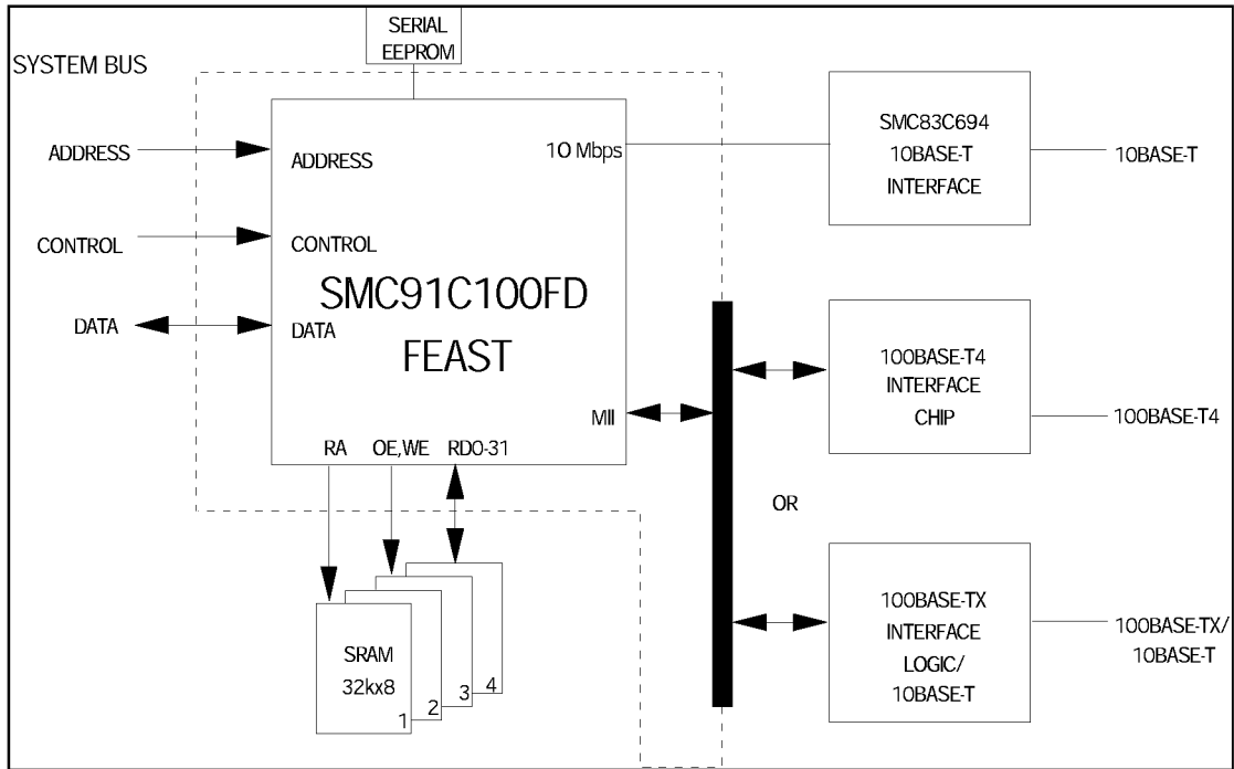
FIGURE 2 - SMC91C100FD SYSTEM DIAGRAM
