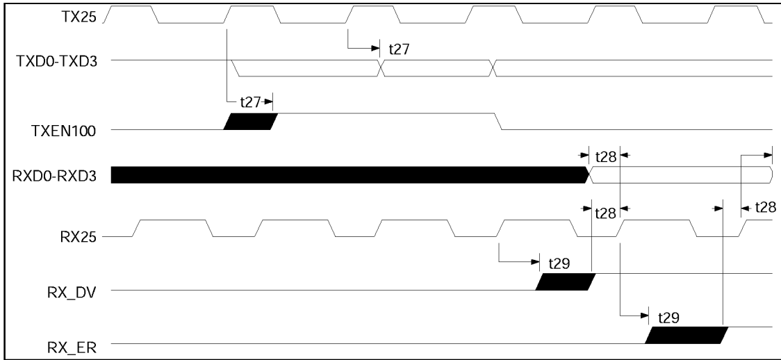
FIGURE 26 - MII INTERFACE
