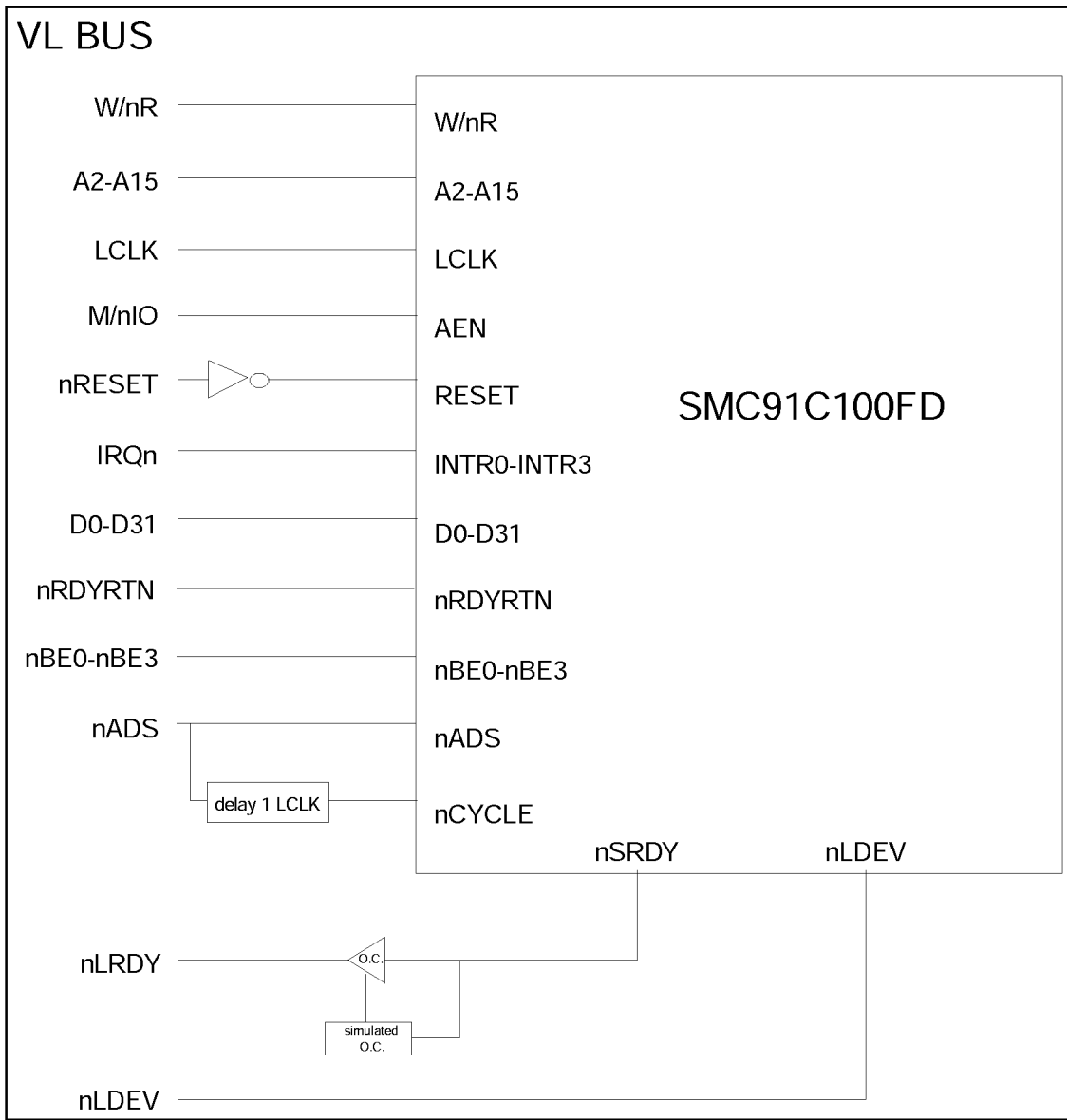
FIGURE 13 - SMC91C100FD ON VL BUS
