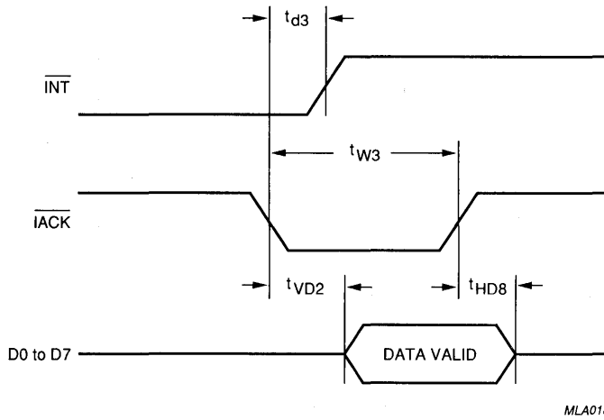
Fig.7 Interrupt timing; 80XX-mode.
