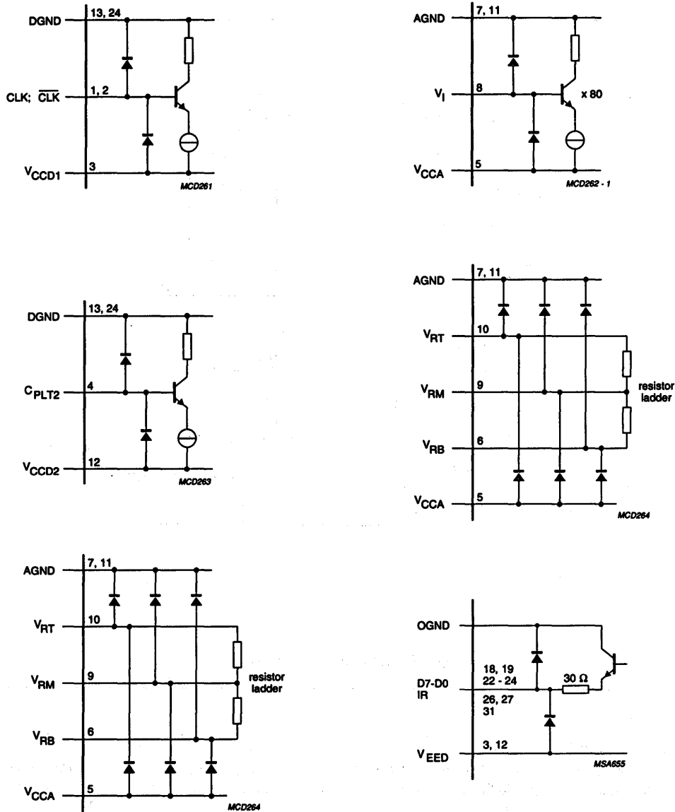
Fig.7 Internal pin configuration diagram.
