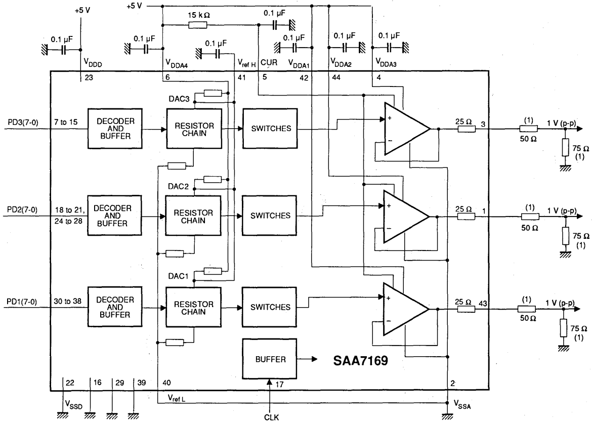
Fig.1 Block diagram and application circuit.
