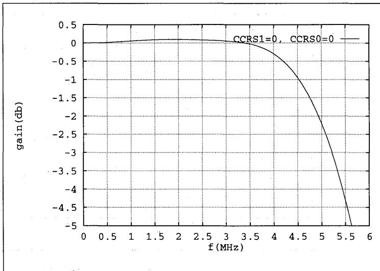
Fig. 6: Luminance transfer characteristic [60 Hz]
