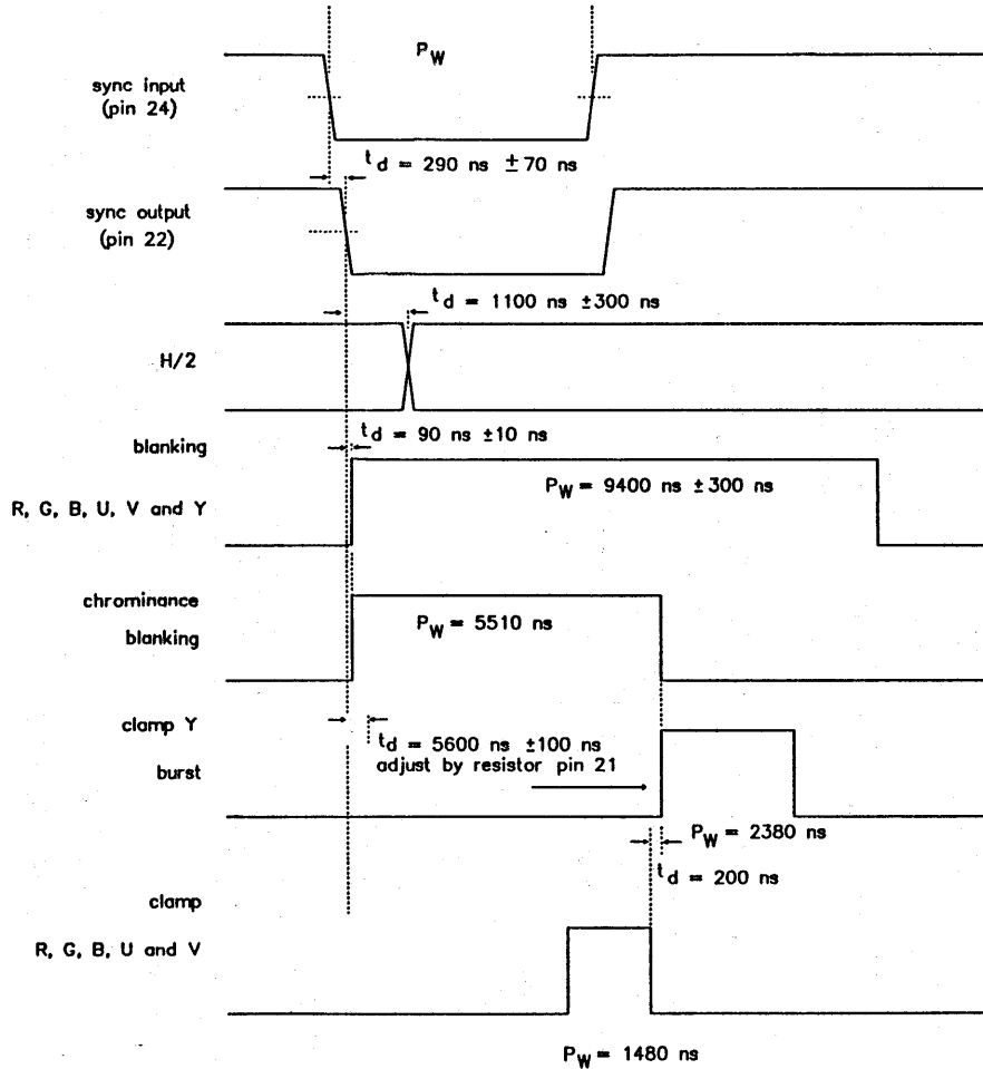
Fig.13 Sync separator and pulse shaper pulse timing levels.
