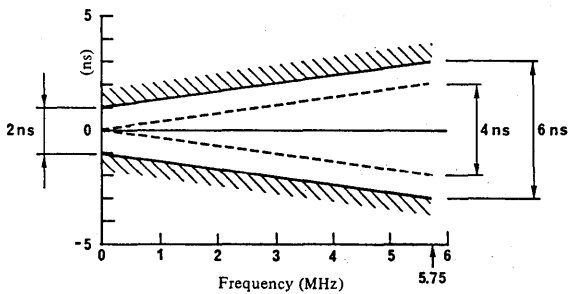
c) Passband group-delay tolerance
