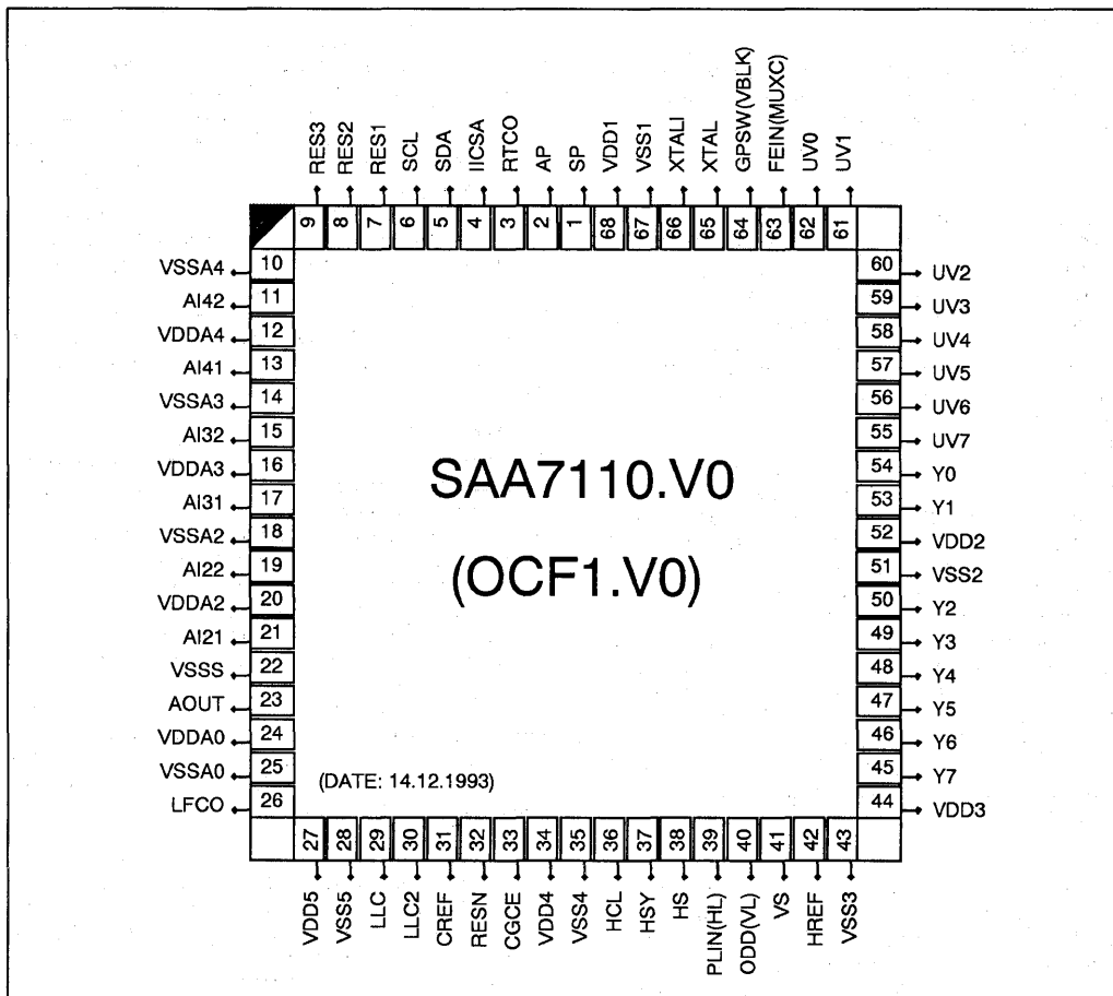
FIGURE 3. PINNING OCF1-SAA7110
