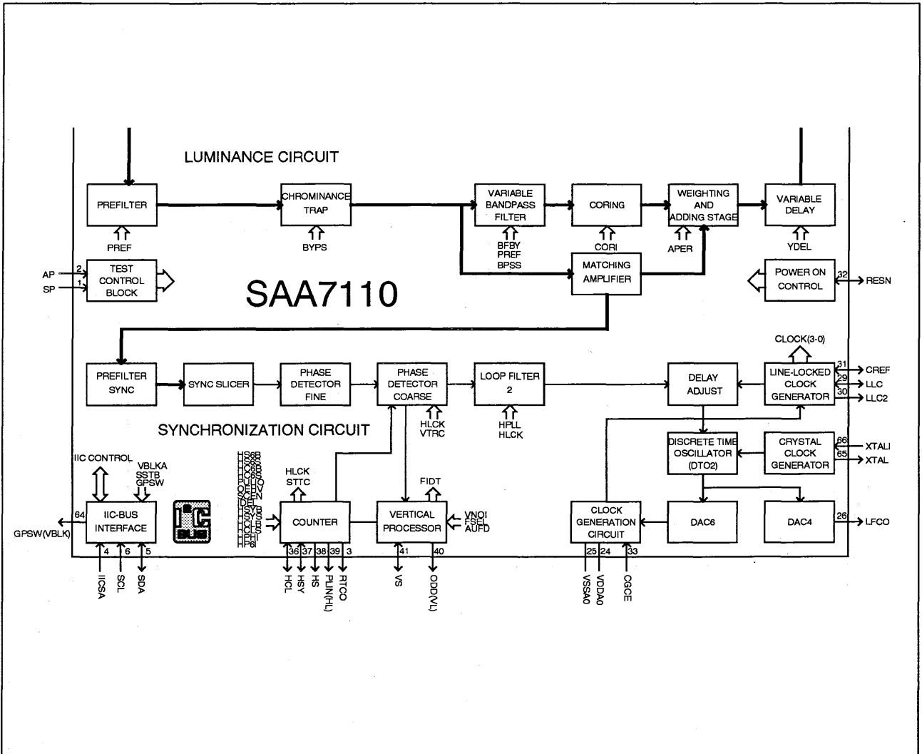
FIGURE 6. BLOCK PICTURE Luminance and Synchronization Part
