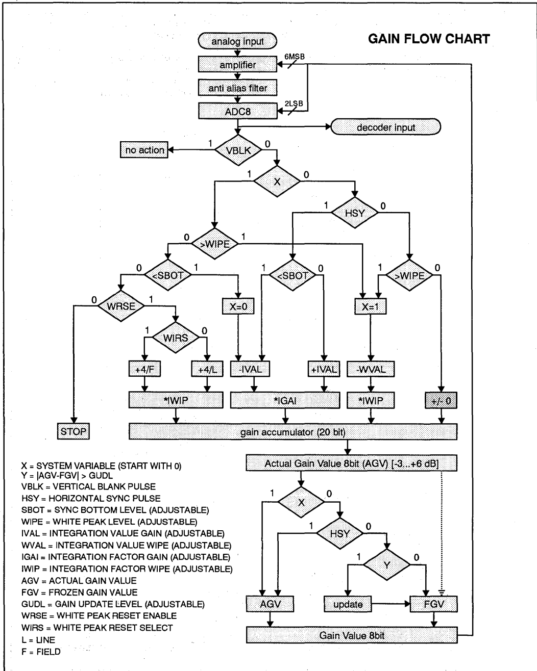
FIGURE 9. LUMINANCE AGC FLOWCHART
