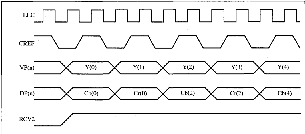
Fig.8 : Dig.TV - Timing
