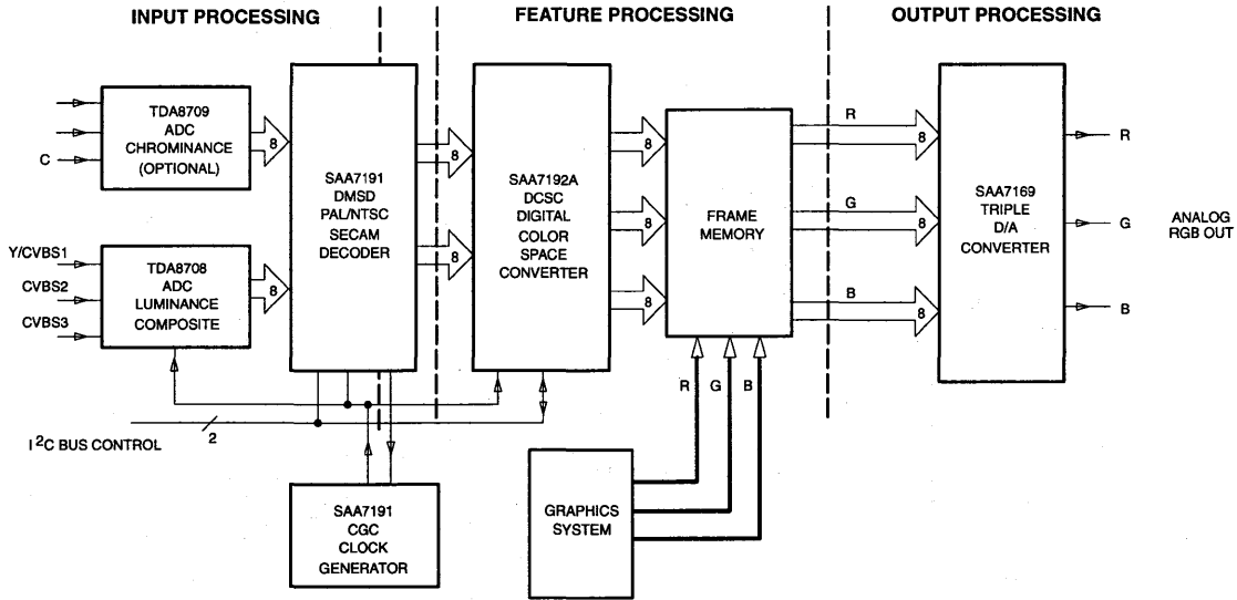
Figure 2. 8-Bit RGB Frame Buffer with Analog RGB Output
