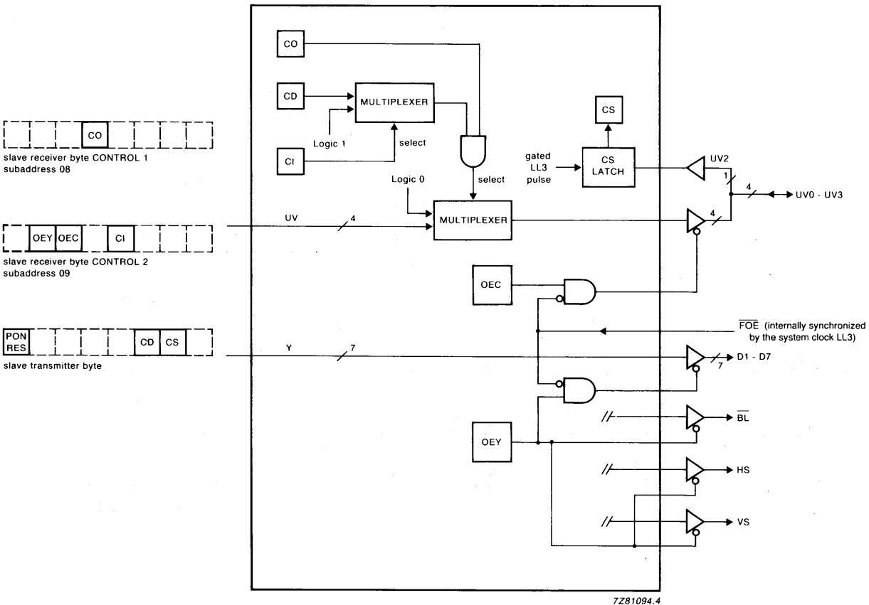
Fig.6 Schematic diagram of control signals at the output interface.
