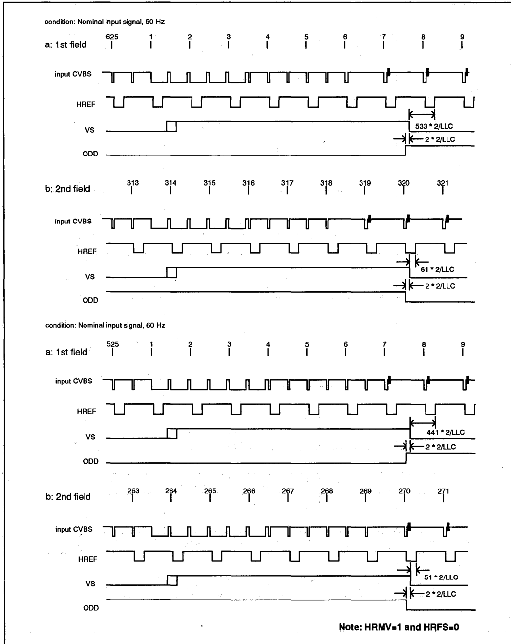
FIGURE 13. VERTICAL TIMING
