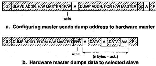
Figure 18. Data Transfer by a Hardware-Transmitter Capable of Dumping Data Directly to Slave Devices
