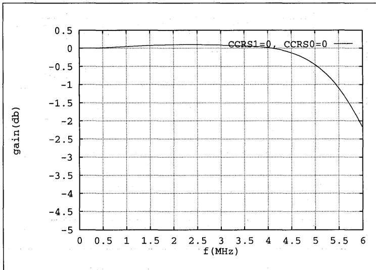
Fig. 10: Luminance transfer characteristic [50 Hz]
