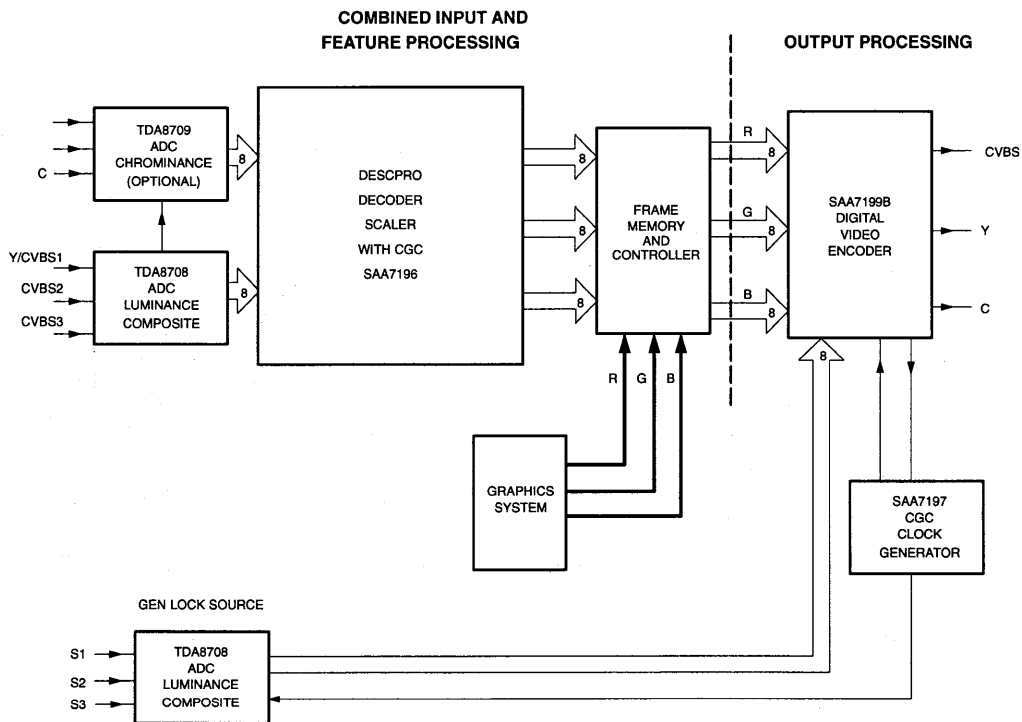
Figure 4. 8-Bit Video Window Graphics with Encoder Gen-Locked to an External Source Using SAA7196 Desco
