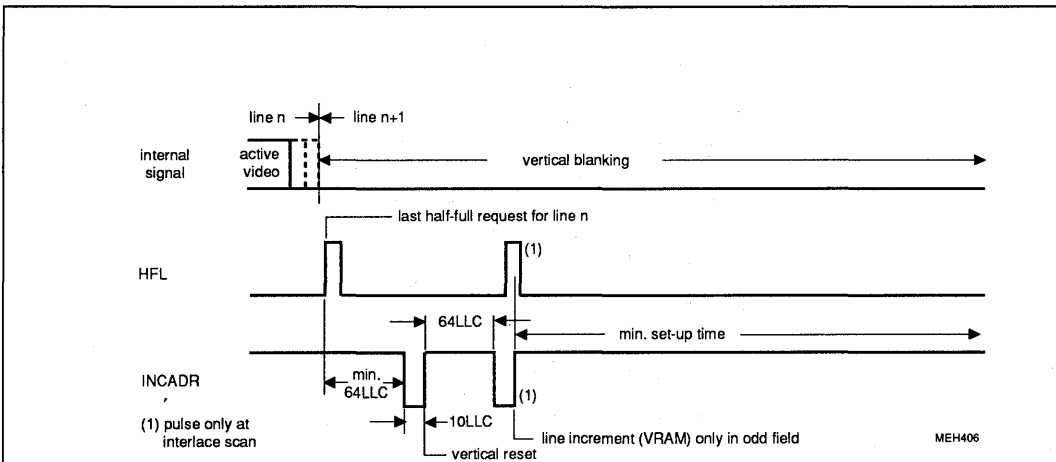
Fig.5 Output port transfer to VRAM at 32-bit data format without scaling. If VCLK cycles occur at VOEN = HIGH, the FIFO register is unchanged, but the outputs VRO(31-0) remain in 3-state position.
