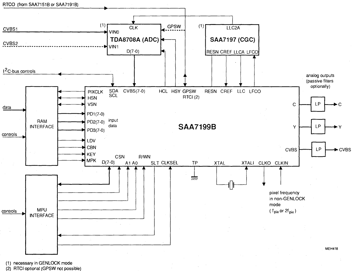
Fig.3 System configuration.
