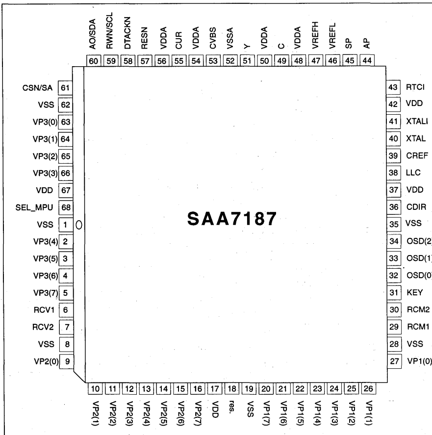
Fig. 2: Pinning Diagram
