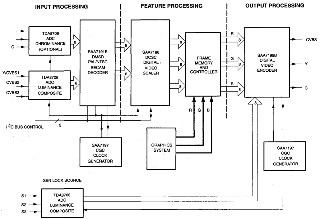
Figure 3. 8-Bit Video Window Graphics with Encoder Gen-Locked to an External Source
