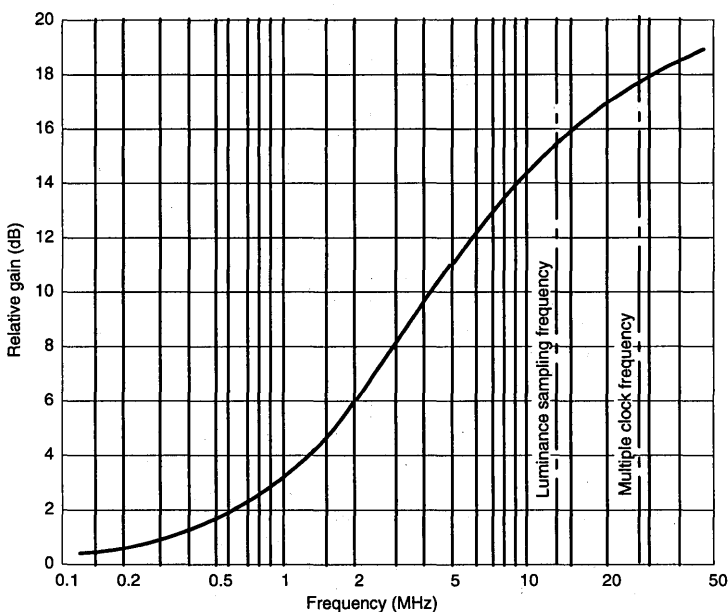
FIGURE 5 — Line receiver equalization characteristic for small signals
