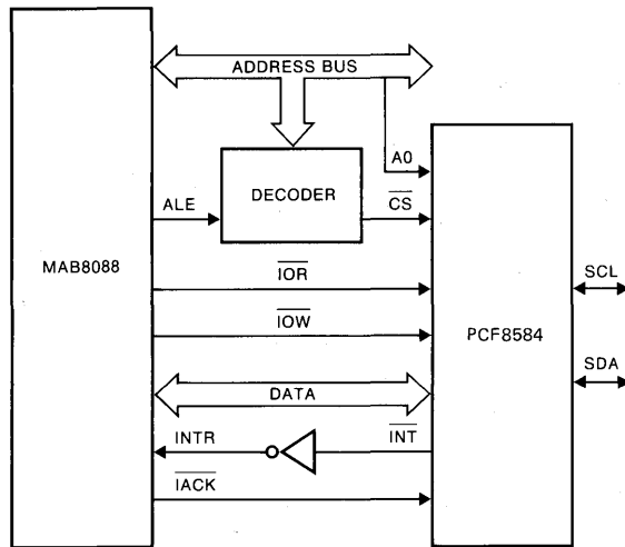
Fig.13 Application diagram using the 8088.
