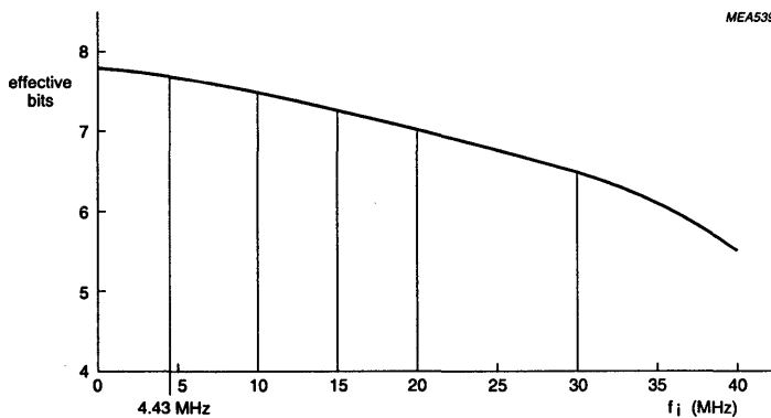
Fig.13 Typical effective bit as a function of input signal at f_{CLK} = 100 MHz.
