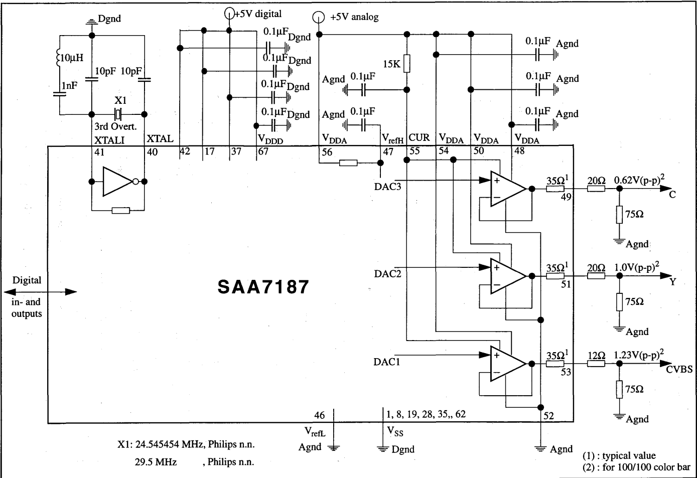
Fig.16: Application Environment of the DENC2-SQ
