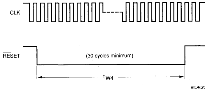
Fig.9 Reset timing.
