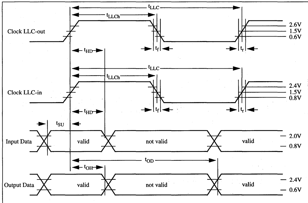
Fig. 7 : Clock Data Timing
