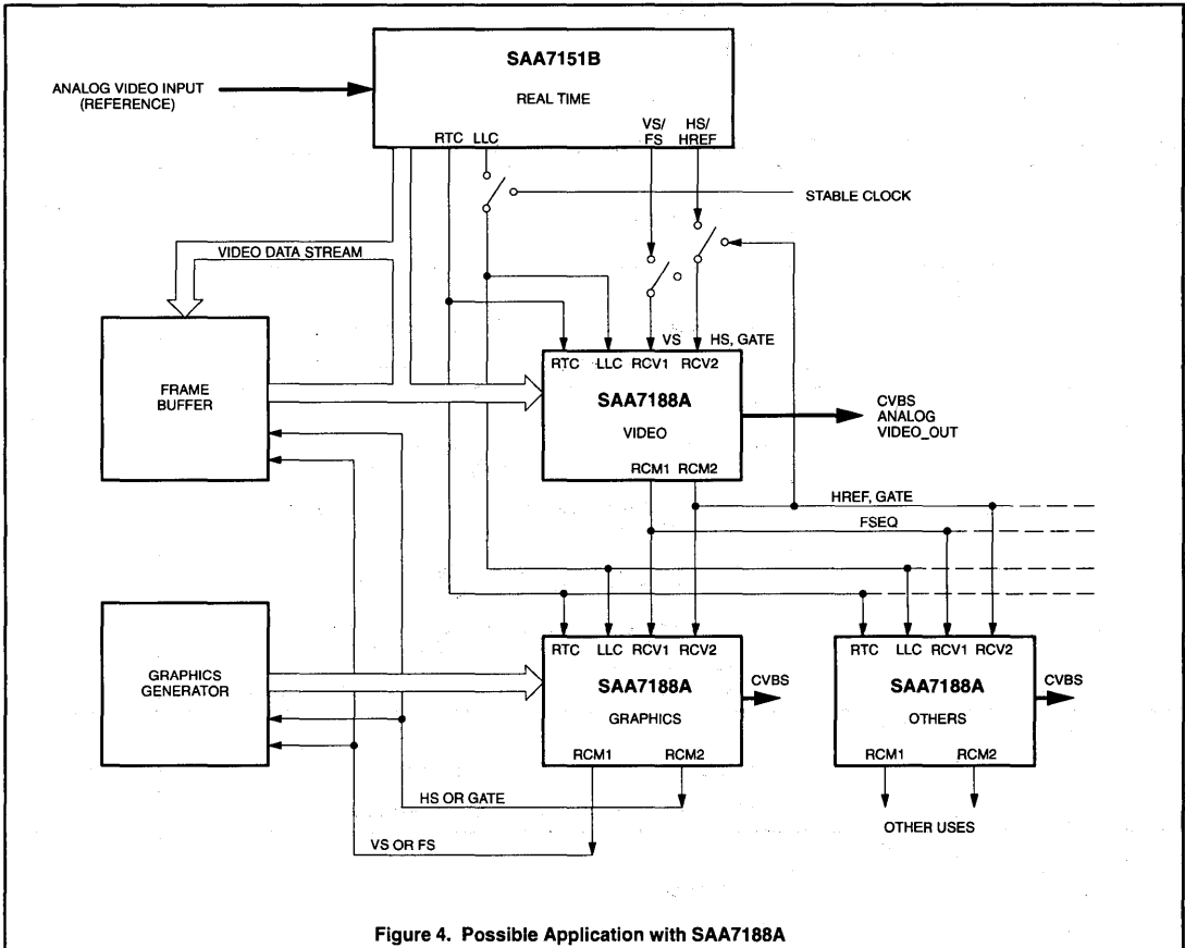
Figure 4. Possible Application with SAA7188A
