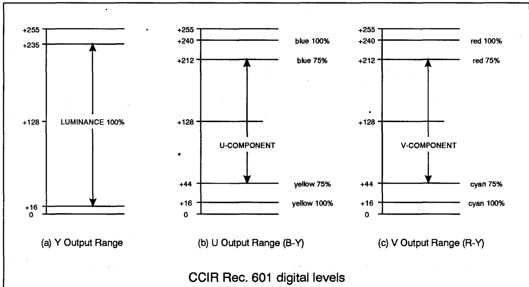
FIGURE 16. YUV OUTPUT SIGNAL RANGE
