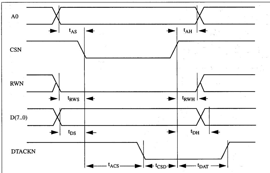
Fig. 15: MPU Interface Timing (Write cycle)
