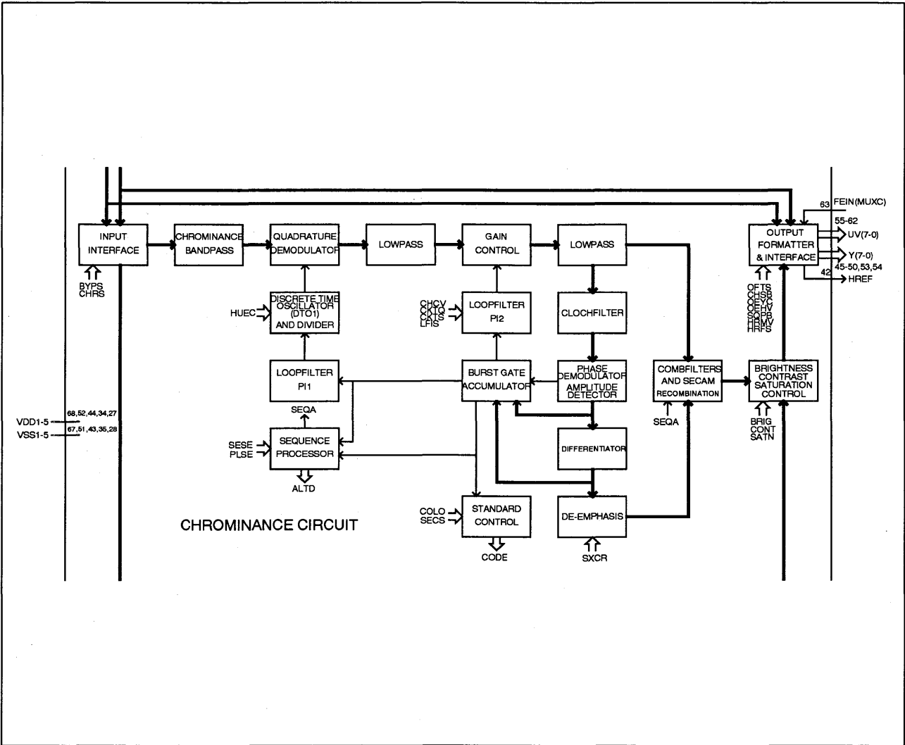
FIGURE 5. BLOCK PICTURE Multi-Standard Decoder Part
