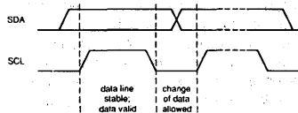
Figure 5. Bit Transfer on the I 2 C-Bus
