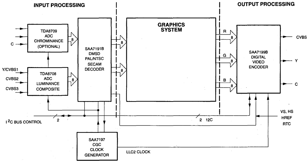
Figure 5. RTC Genlock Mode (Uses Single CGC)
