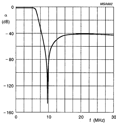
Fig.14 Frequency response for filter shown in Fig.13.
