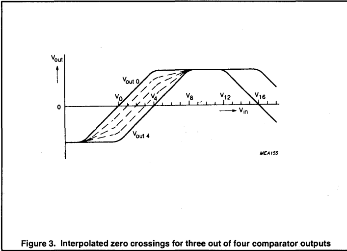
Figure 3. Interpolated zero crossings for three out of four comparator outputs
