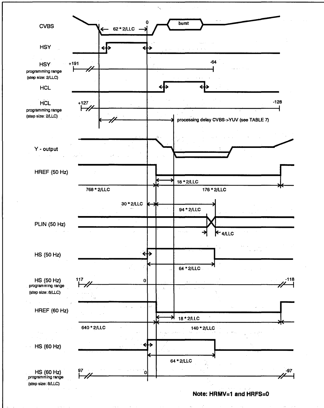
FIGURE 11. HORIZONTAL TIMING
