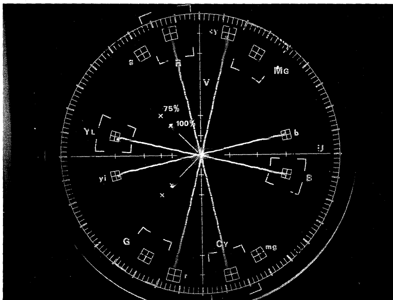
Figure 2. Color transients
