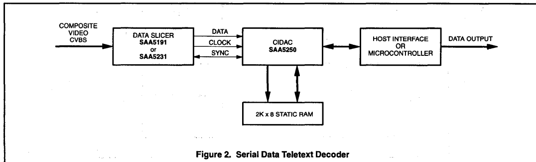
Figure 2. Serial Data Teletext Decoder
