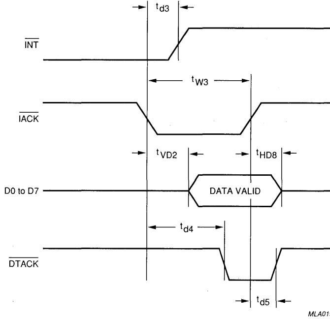
Fig.8 Interrupt timing; 68000-mode.
