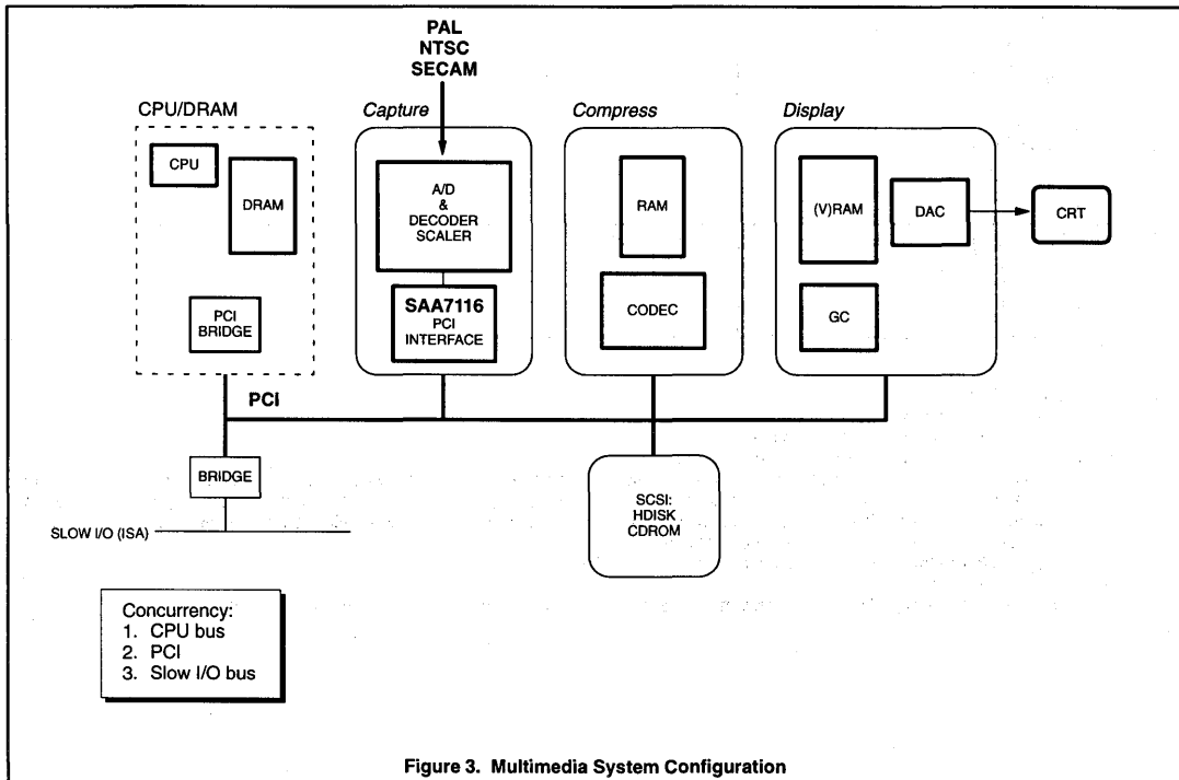
Figure 3. Multimedia System Configuration
