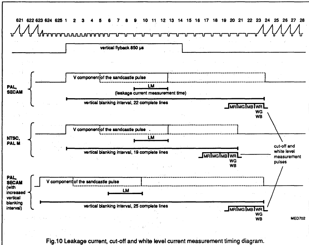
Fig.10 Leakage current, cut-off and white level current measurement timing diagram.
