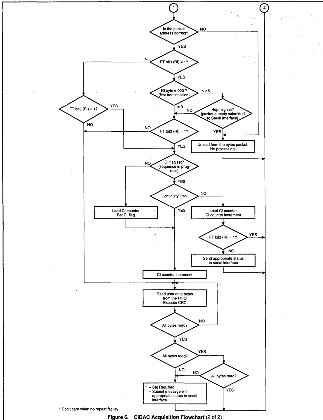
Figure 6. CIDAC Acquisition Flowchart (2 of 2)
