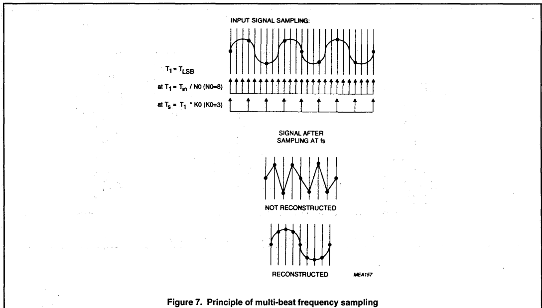
Figure 7. Principle of multi-beat frequency sampling
