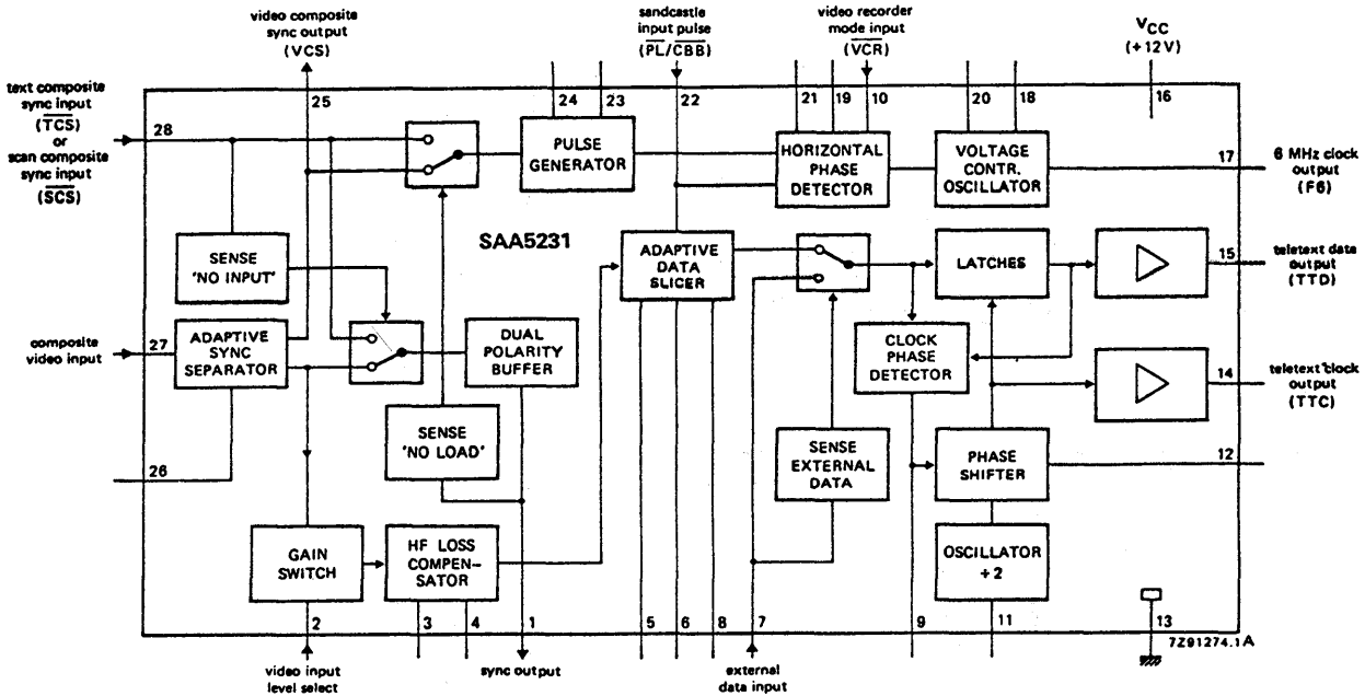
Fig. 1 Block diagram.
