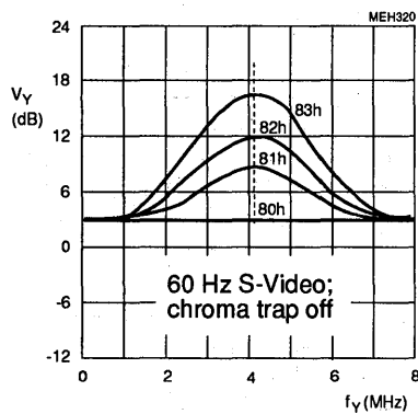
Fig.33 4.1 MHz luminance peaking control control as a function of four different aperture factors controllable by subaddress byte 06; pre-filter off; coring off and bandpass filter on.
