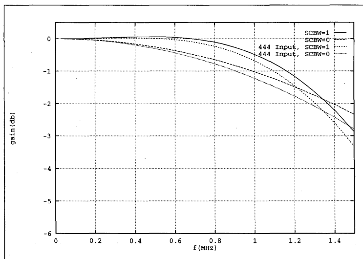
Fig. 8: Chrominance transfer characteristic [50 Hz]
