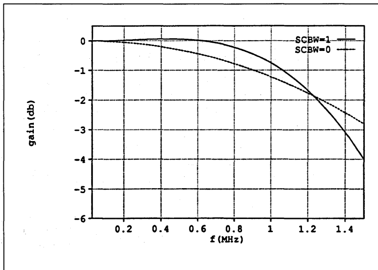
Fig. 4 : Chrominance transfer characteristic
