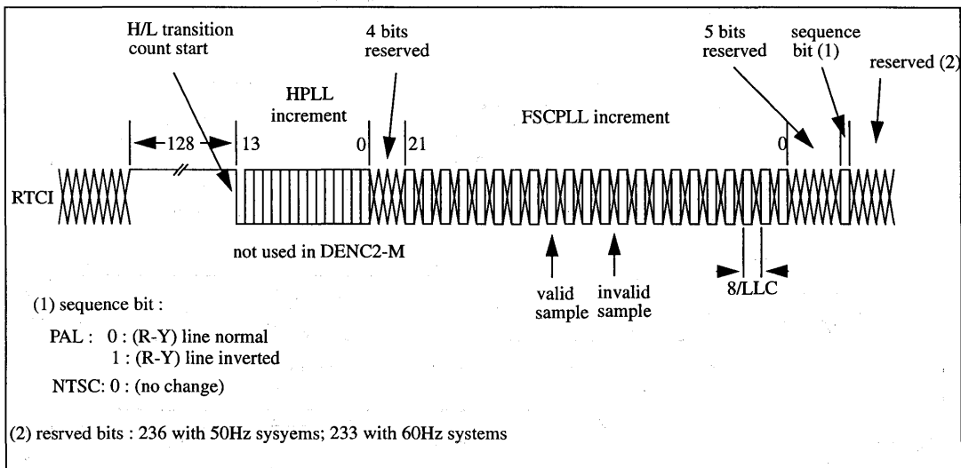
Fig.9 : RTCI timing
