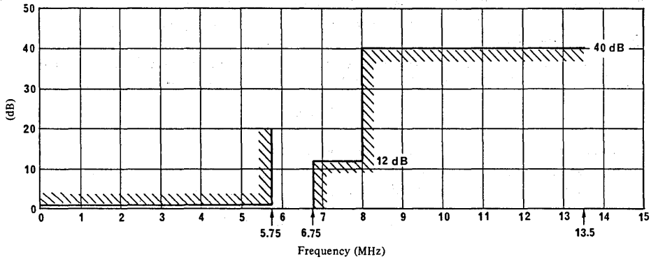
a) Template for insertion loss/frequency characteristic
