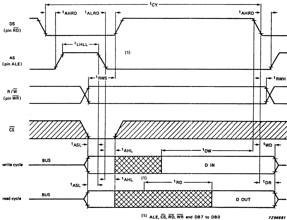
Fig. 12 Timing diagram for microcontroller interface (Motorola).
