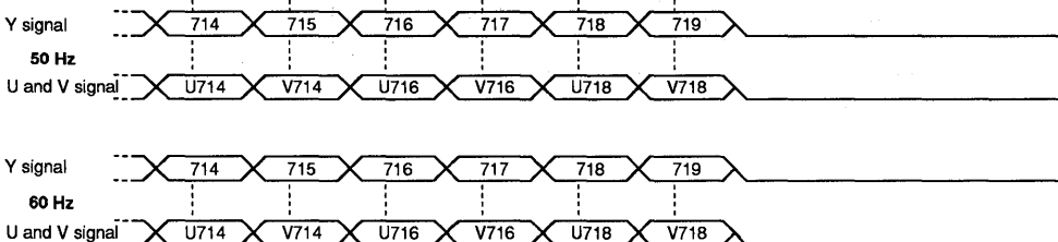
Fig.3 Line control by HREF for 4 : 2 : 2 format, CREF = 13.5 MHz; HREF = 720 pixel; 50 Hz and 60 Hz field.
