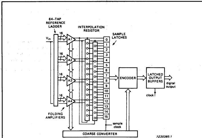
Figure 5. Block diagram of a complete folding and interpolating ADC
