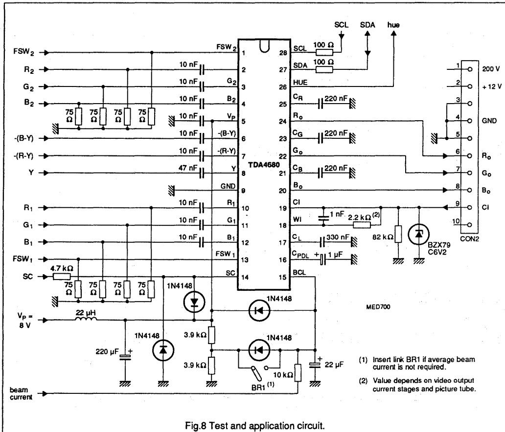
Fig. 8 Test and application circuit.
