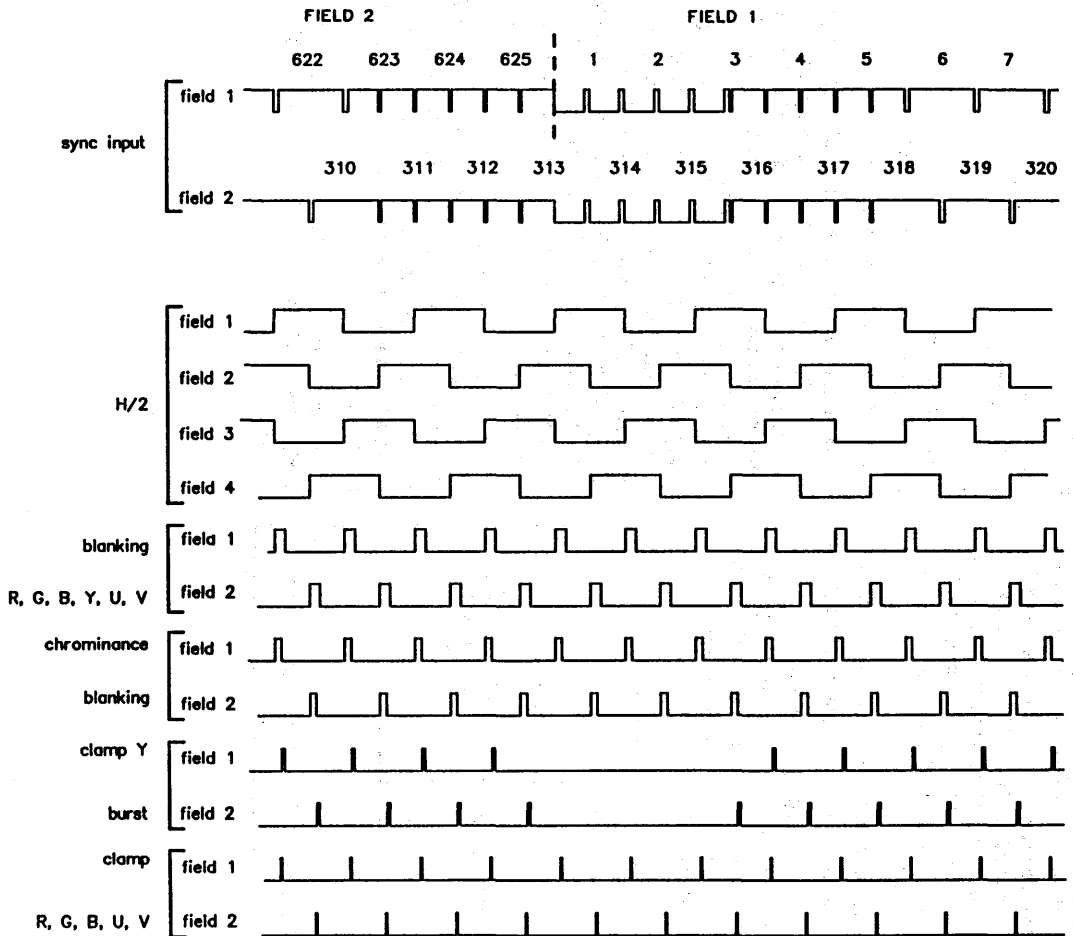
Fig.12 Sync separator and pulse shaper pulses.
