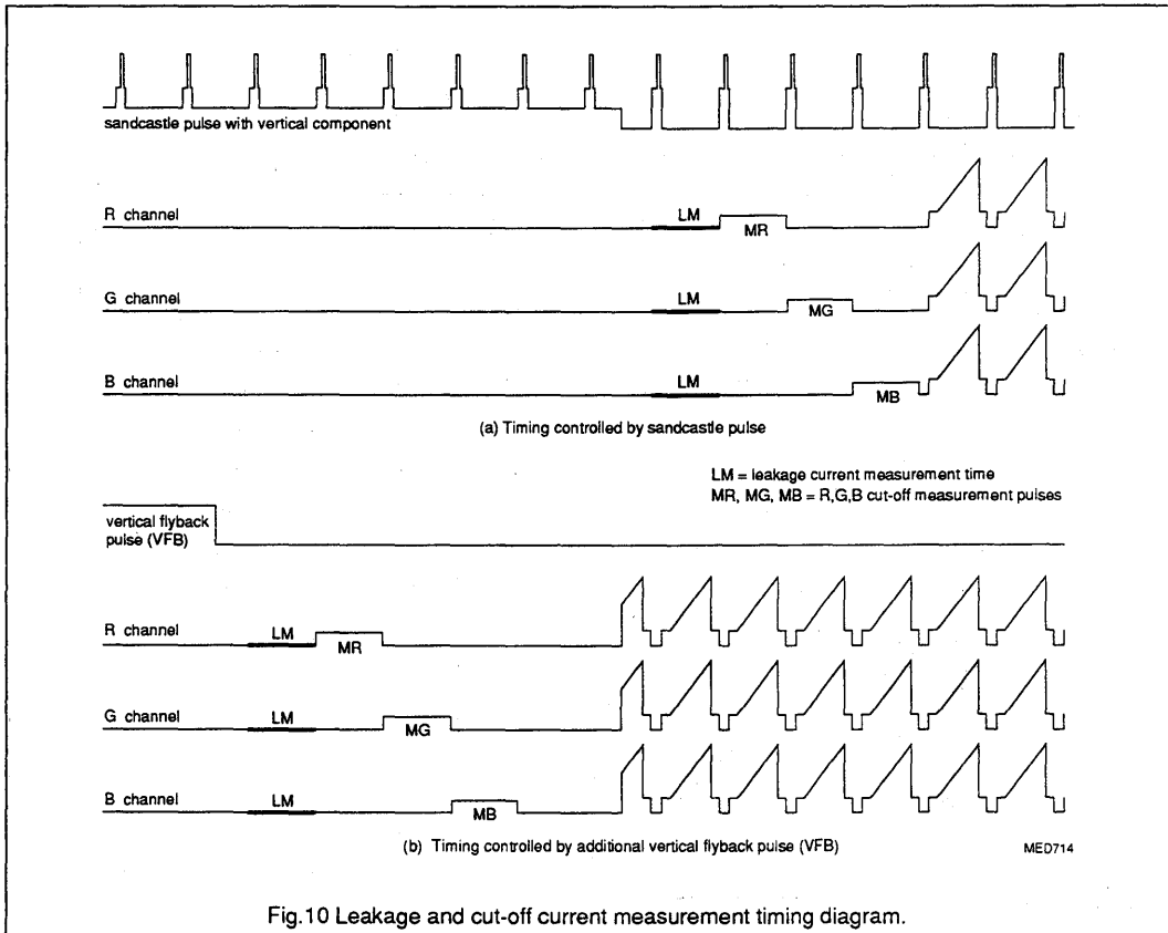
Fig.10 Leakage and cut-off current measurement timing diagram.
