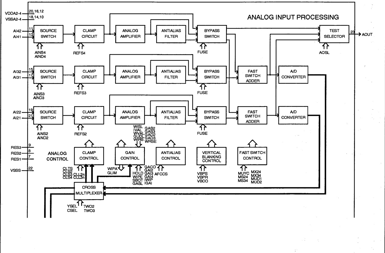
FIGURE 4. BLOCK PICTURE Analog Input and Analog Control Part
