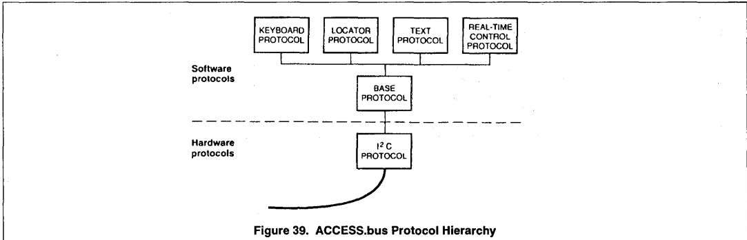
Figure 39. ACCESS.bus Protocol Hierarchy
