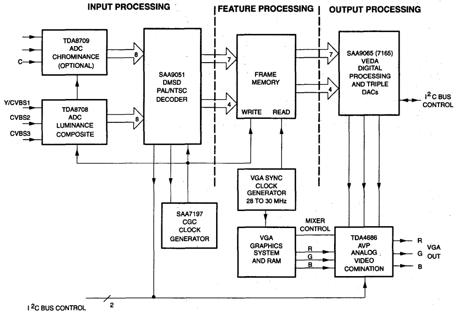
Figure 1. 7-Bit Low Cost Video Frame Grabber with VGA Out
