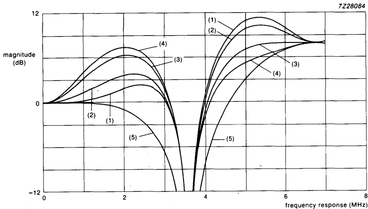
Fig.16 Magnitude of the frequency response of the unlimited summation signal (combining Channel 1 and Channel 2); NTSC mode; prefilter ON; Responses 1 to 5 show various comb-filter combinations programmable by bits BP2 and BP1, via the I 2 C-bus.
