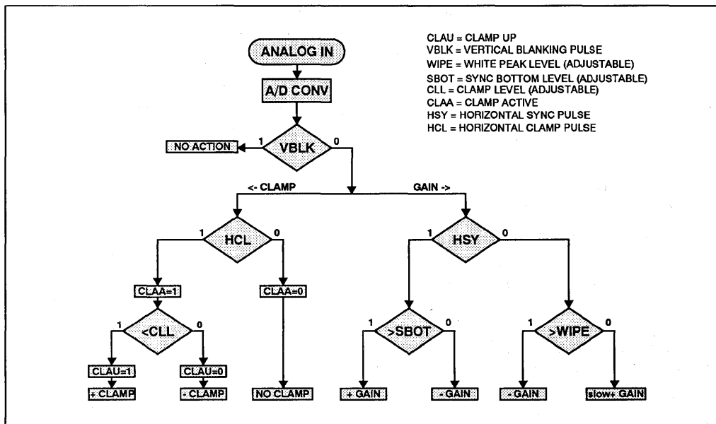
FIGURE 8. CLAMP AND GAIN FLOWCHART
