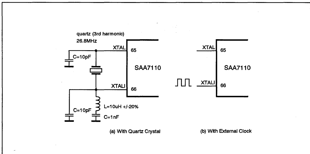
FIGURE 17. OSCILLATOR APPLICATION
