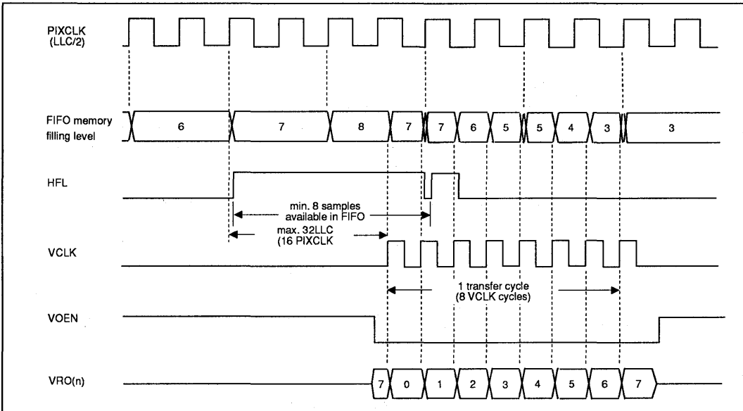
Fig.5 Output port transfer to VRAM at 32-bit data format without scaling. If VCLK cycles occur at VOEN = HIGH, the FIFO register is unchanged, but the outputs VRO(31-0) remain in 3-state position.
