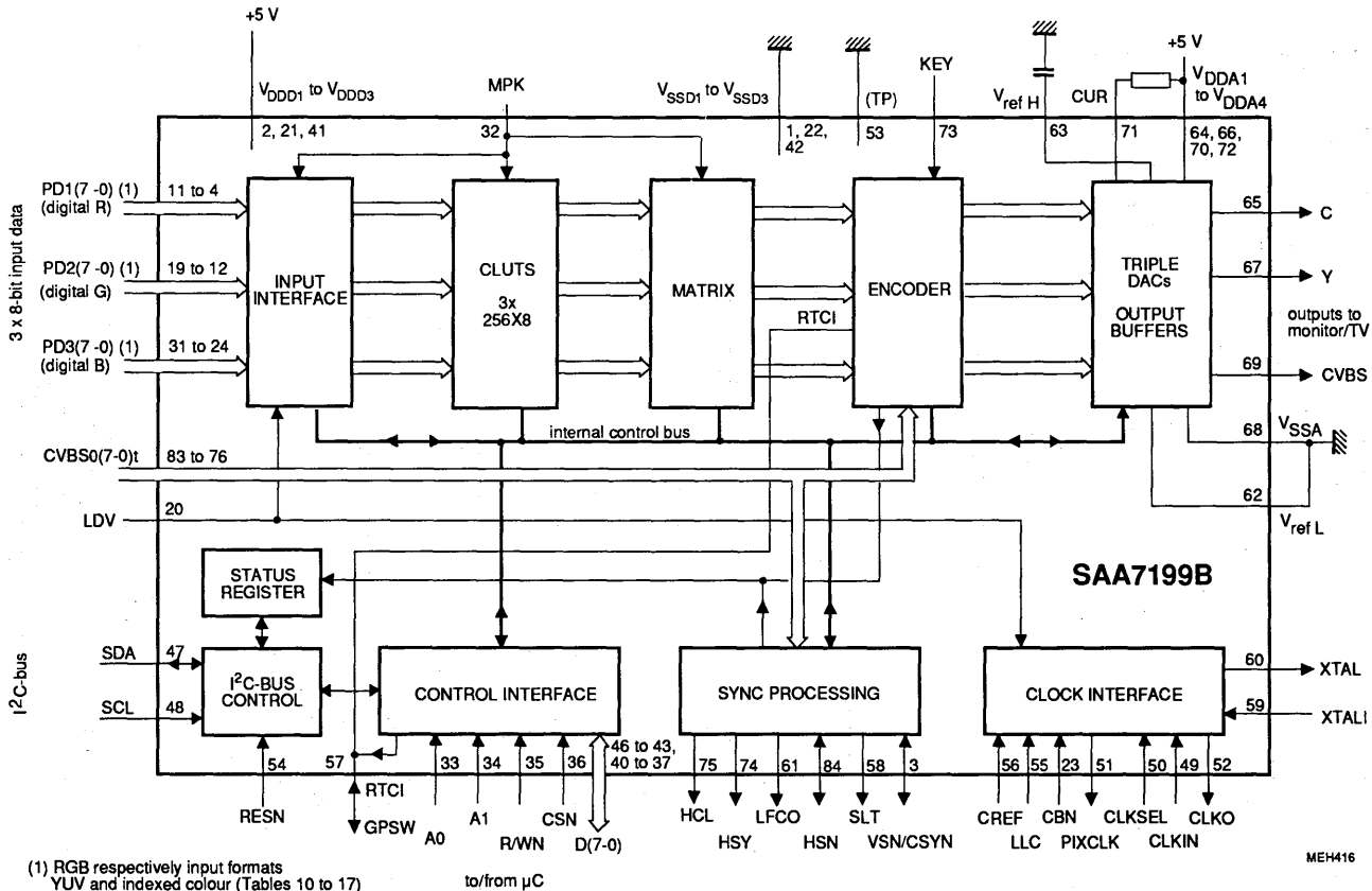
Fig. 1 Block diagram (application details Fig.4).
