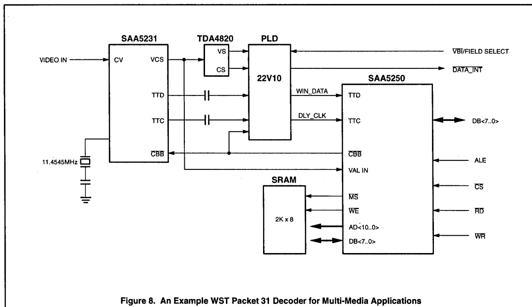
Figure 8. An Example WST Packet 31 Decoder for Multi-Media Applications
