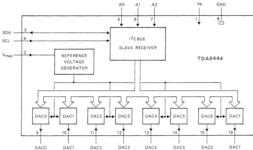
Fig. 1 Block diagram.
