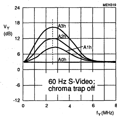
Fig.34 2.6 MHz luminance peaking control control as a function of four different aperture factors controllable by subaddress byte 06; pre-filter off; coring off and bandpass filter on.
