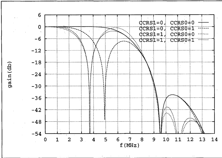
Fig. 9: Luminance transfer characteristic [50 Hz]
