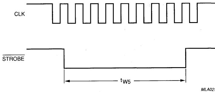
Fig.10 Strobe timing.
