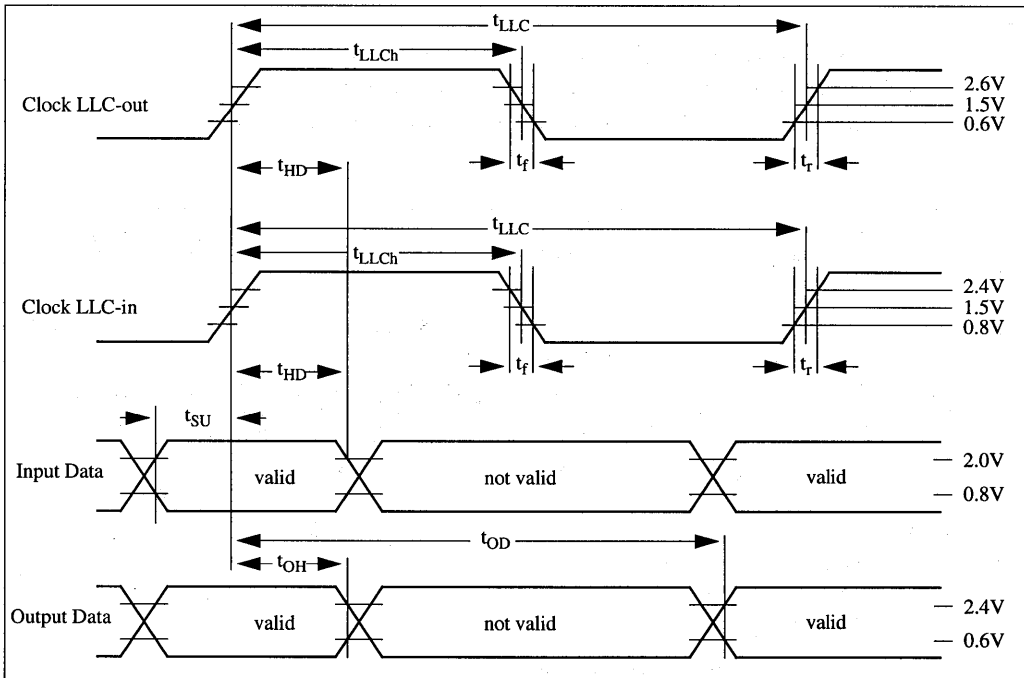
Fig. 11: Clock Data Timing
