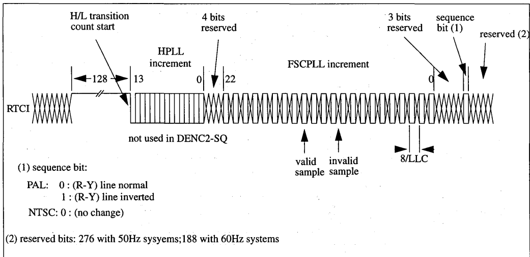
Fig. 13: RTCI timing
