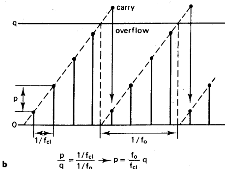
Fig. 5. Principle of the discrete time oscillator.
