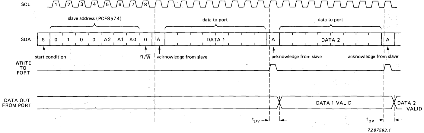
Fig.10 WRITE mode (output port).
