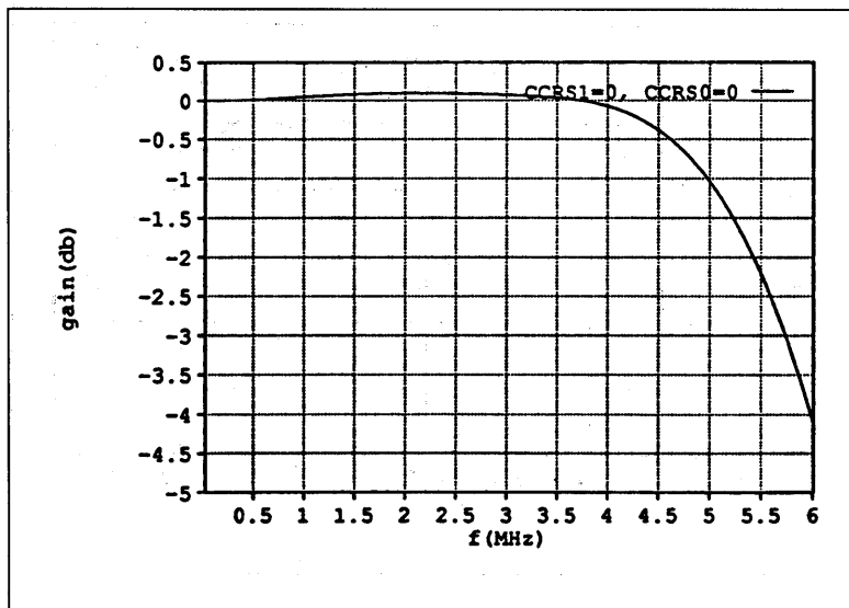
Fig.6 : Luminance transfer characteristic
