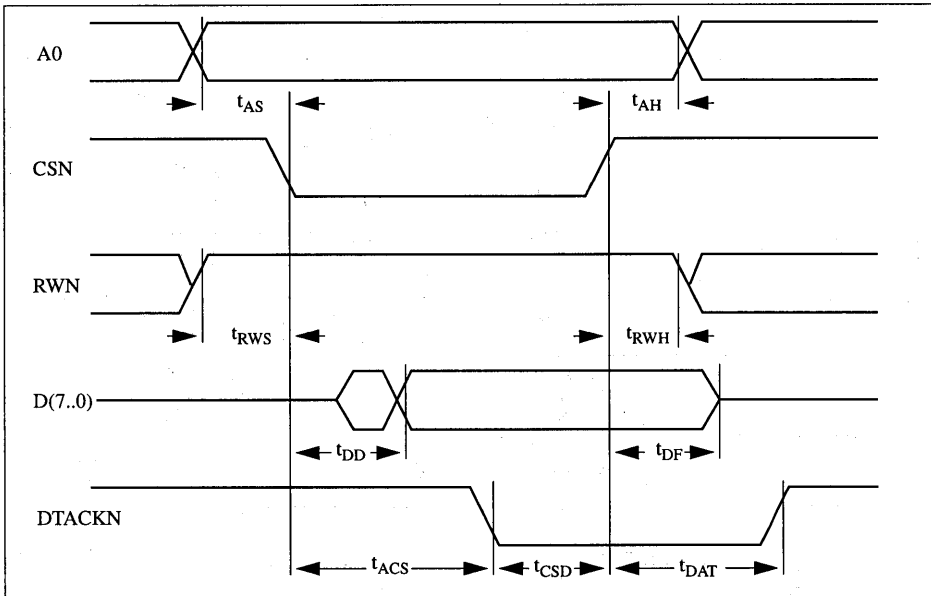
Fig. 14: MPU Interface Timing (Read cycle)
