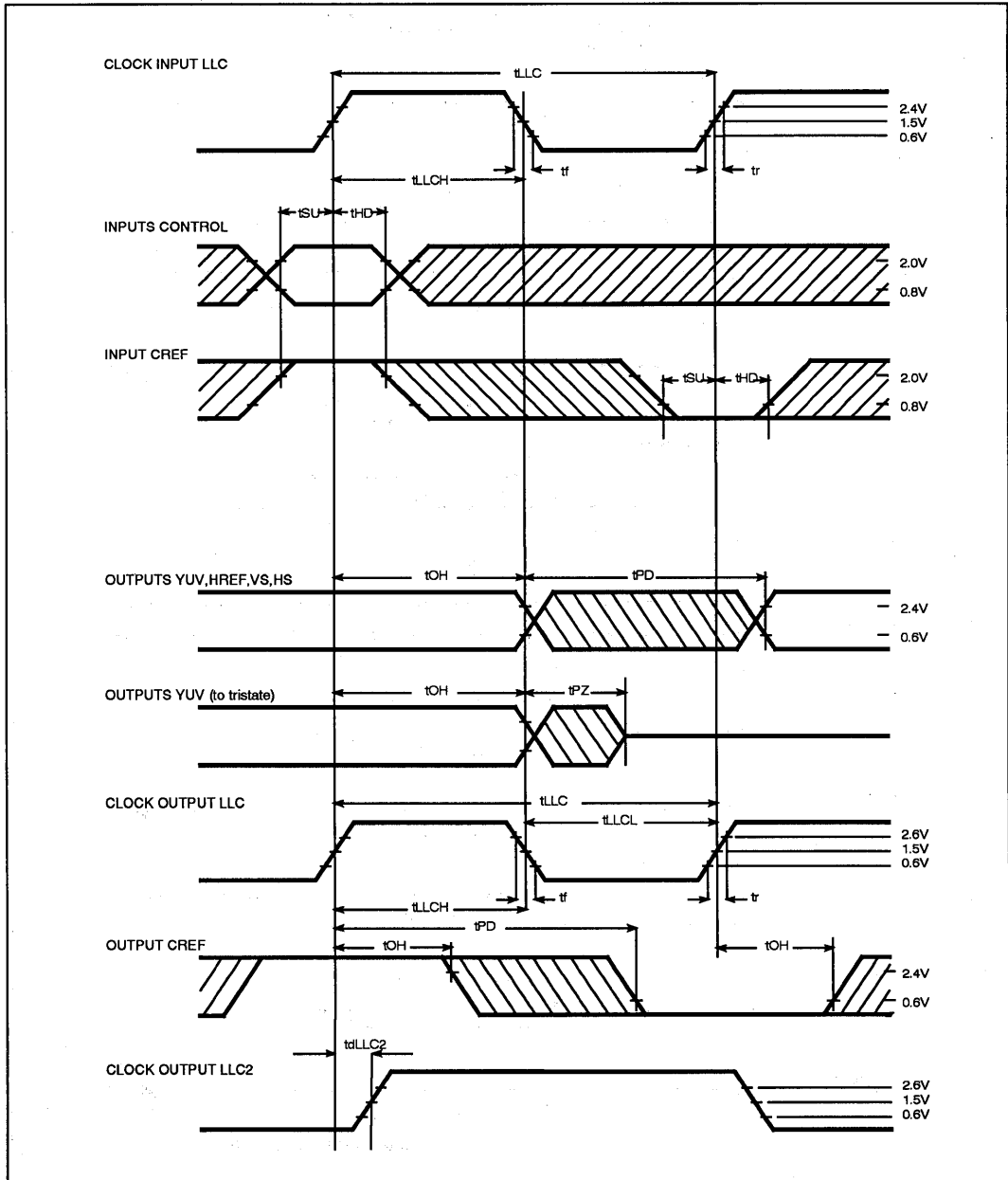
FIGURE 10. CLOCK/DATA TIMING
