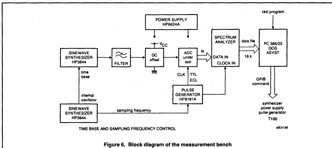
Figure 6. Block diagram of the measurement bench
