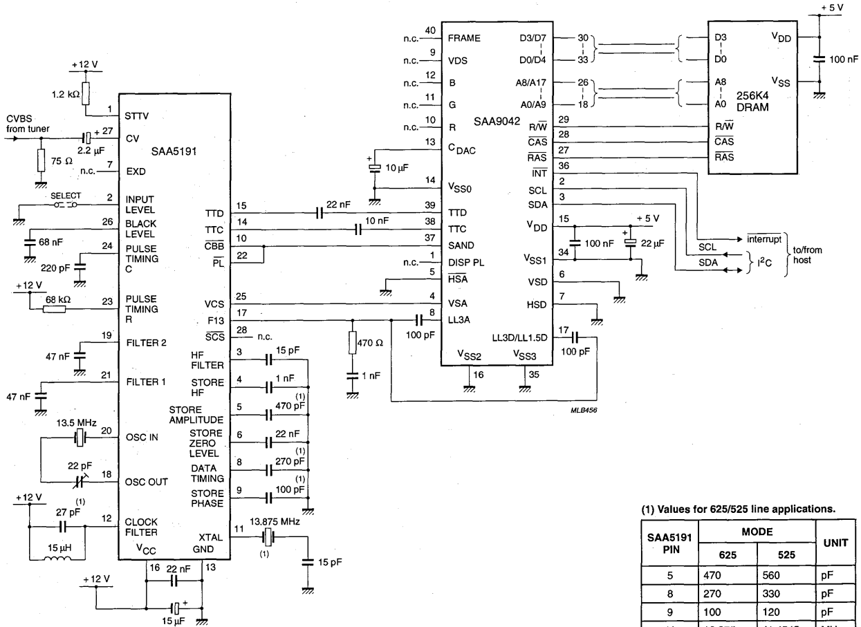
Fig.10 SAA9042 solution for multi-media applications.
