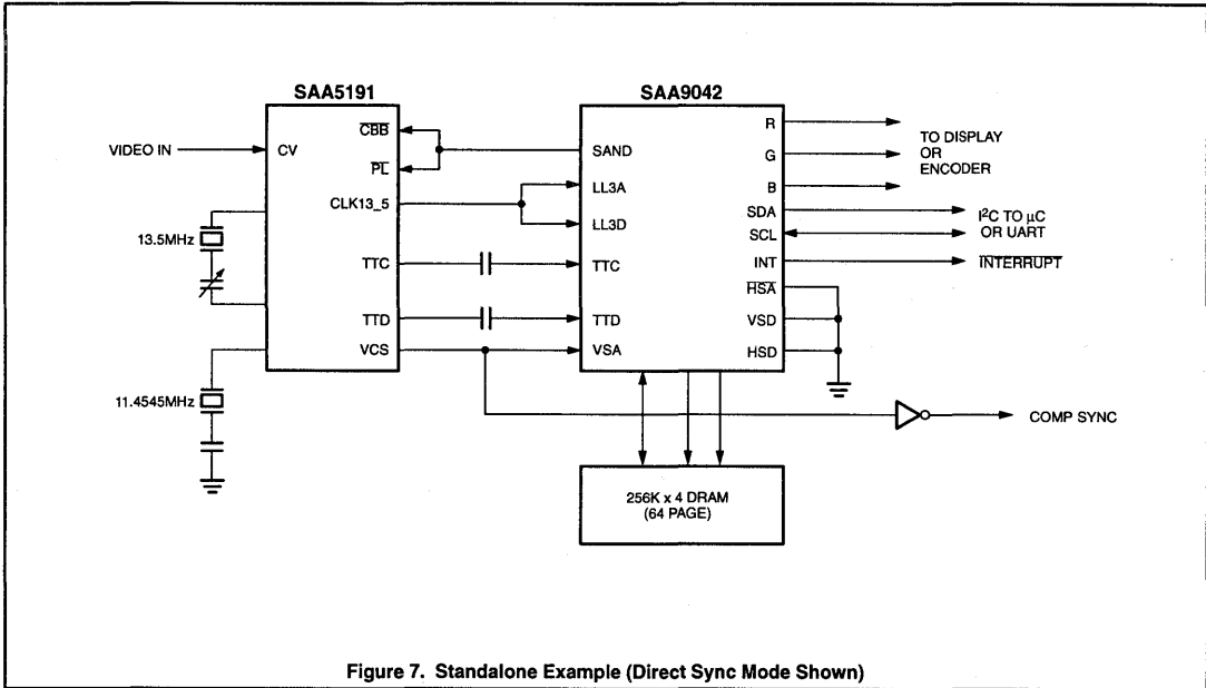
Figure 7. Standalone Example (Direct Sync Mode Shown)
