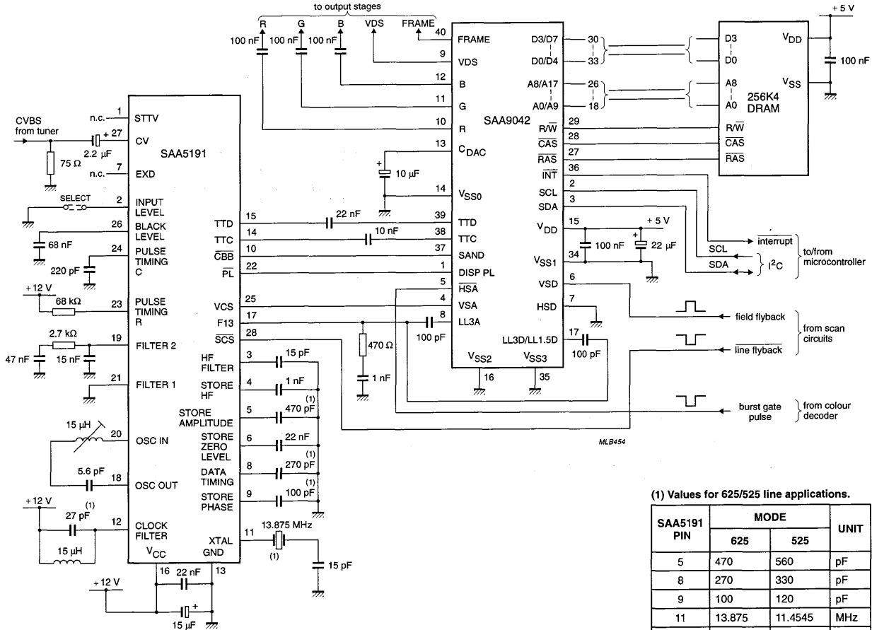
Fig.8 SAA9042 solution for 50/60 Hz analog TV (1H/1V) - scan sync mode.
