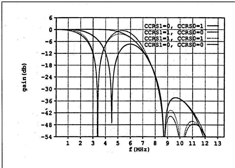
Fig. 5 : Luminance transfer characteristic
