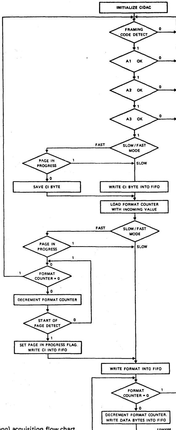
Fig. 4 DIDON (long) acquisition flow chart.
