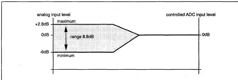
FIGURE 7. AUTOMATIC GAIN CONTROL RANGE
