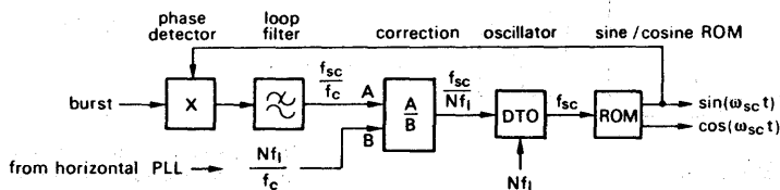
Fig. 8. Forward control of subcarrier DTO operating with line-locked clock.
