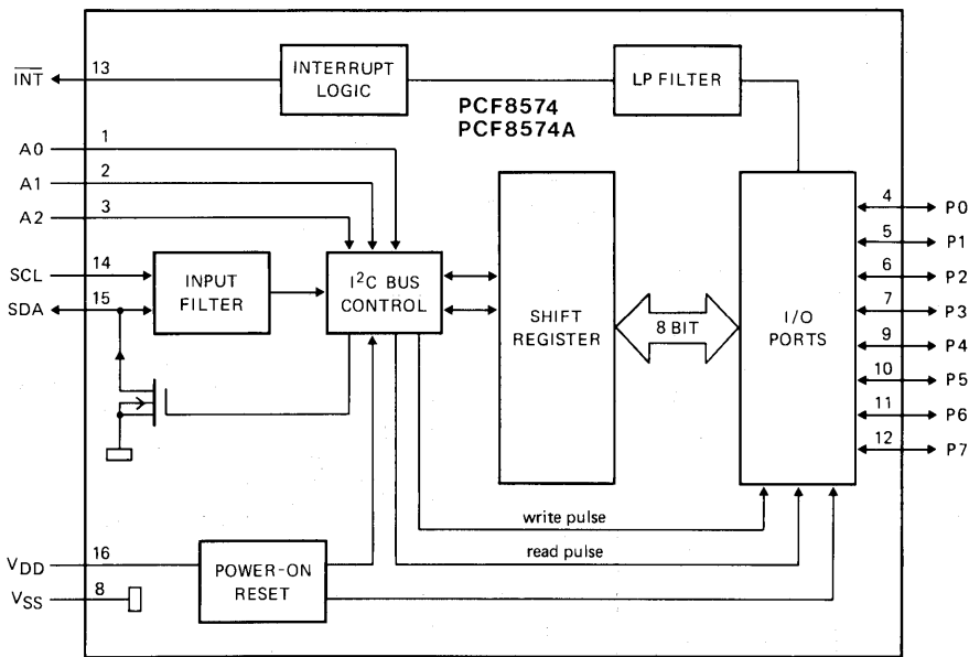
Fig.1 Block diagram.
