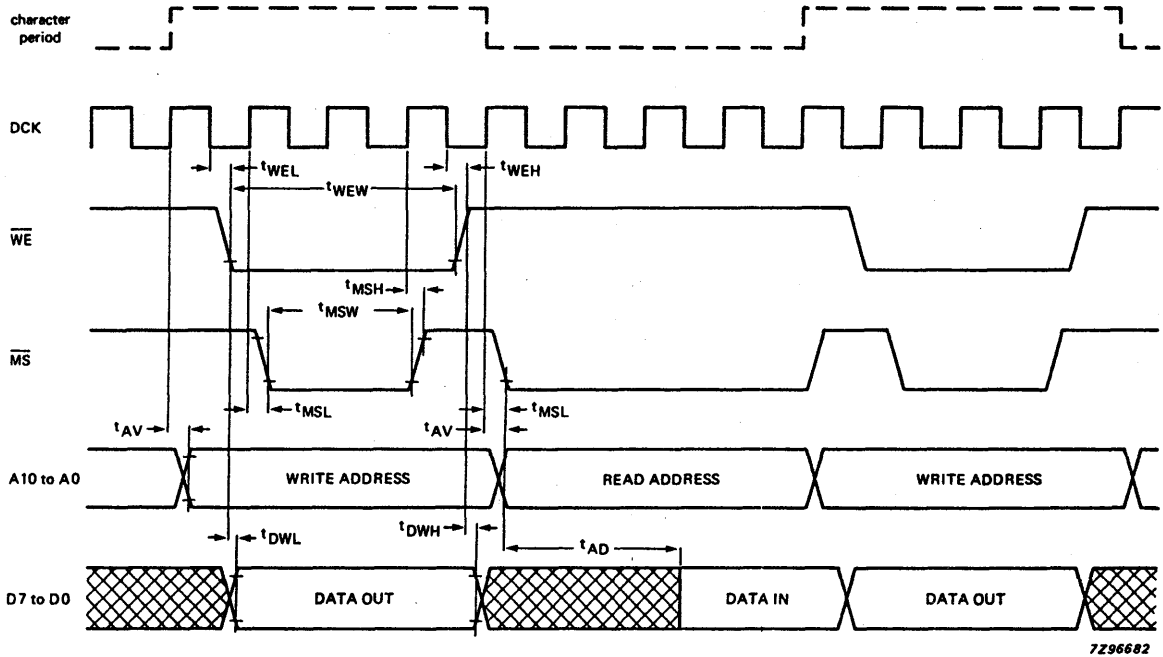
Fig. 13 Timing diagram for memory interface.
