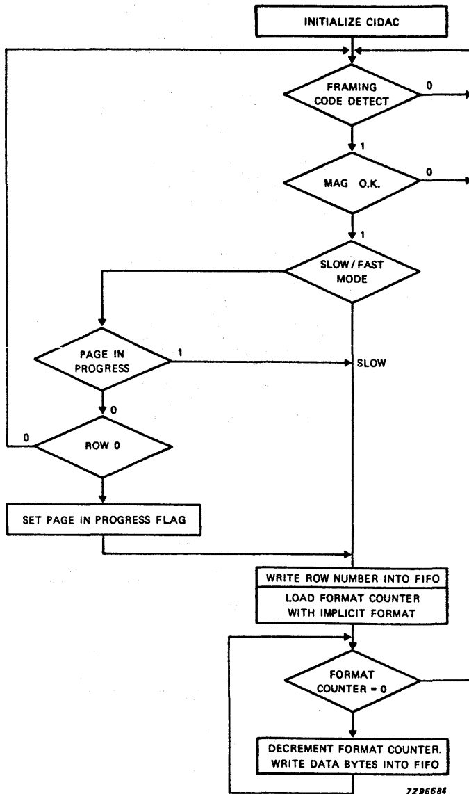
Fig. 8 U.K. teletext acquisition flow chart.
