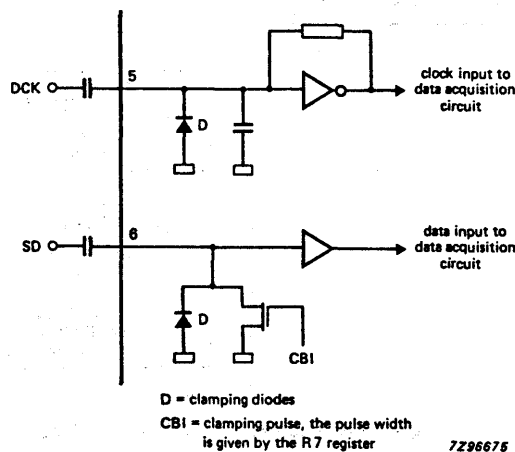
Fig. 10 SD and DCK input circuitry.
