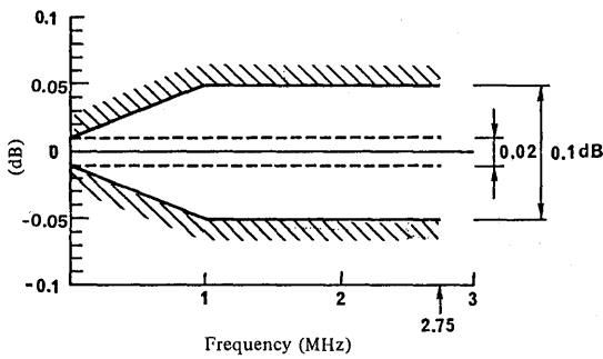
b) Passband ripple tolerance
