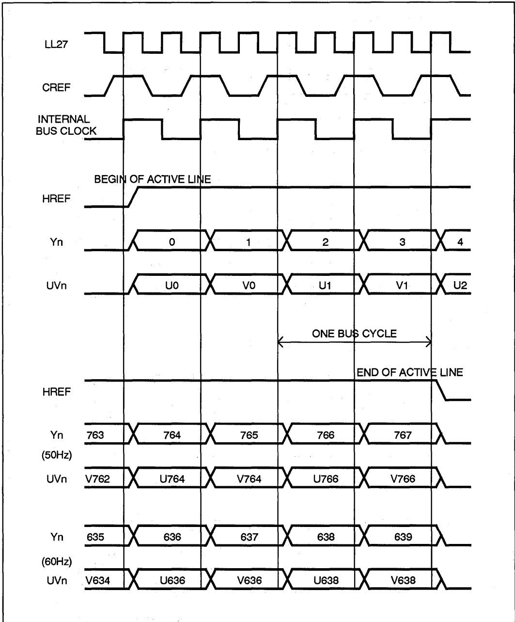
FIGURE 12. HREF TIMING
