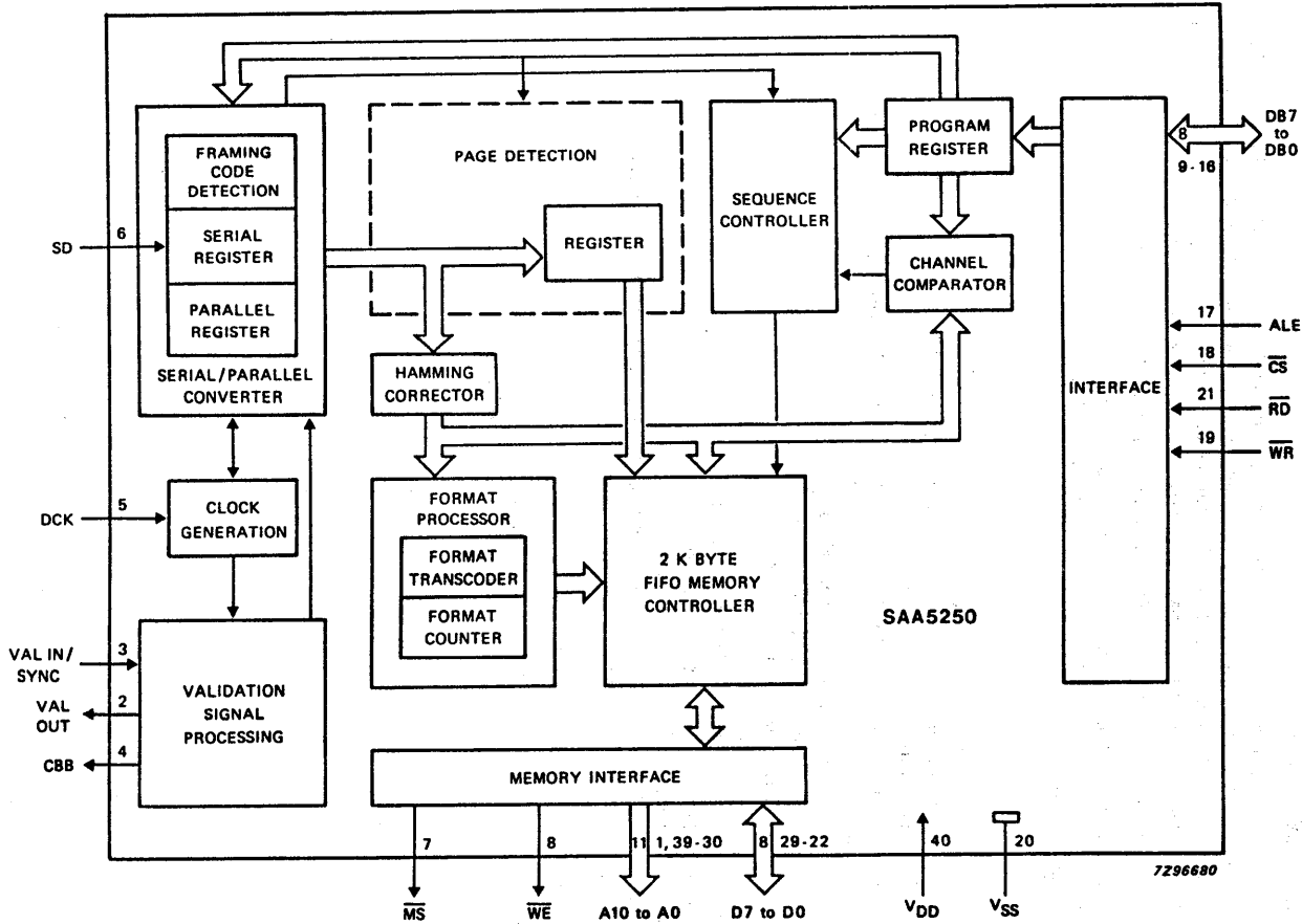
Fig. 1 Block diagram.
