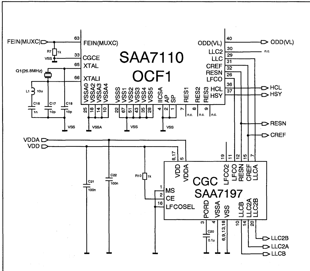
FIGURE 23. APPLICATION WITH EXTERNAL CGC
