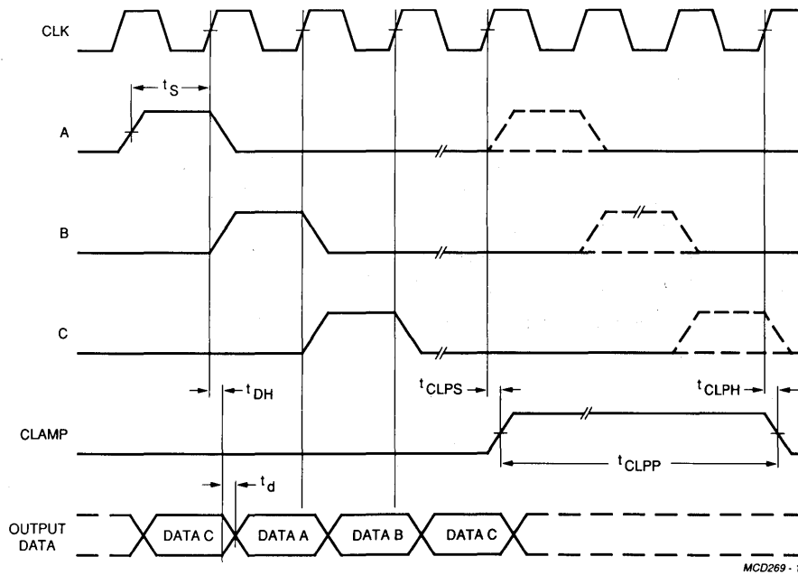
Fig.4 AC characteristics select signals; Clamp, Data.
