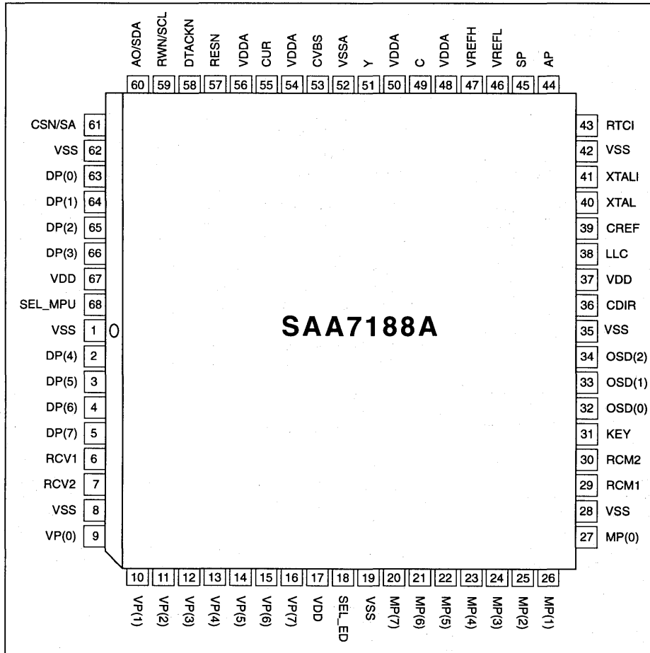
Fig. 2: Pinning Diagram
