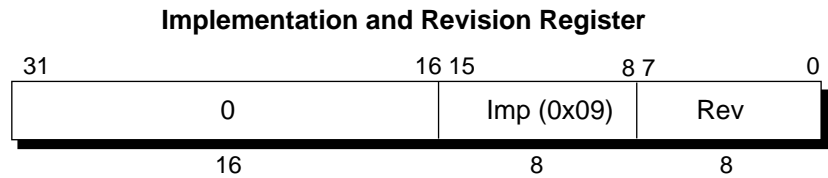
Figure 14-6 FP Implementation and Revision Register Format
