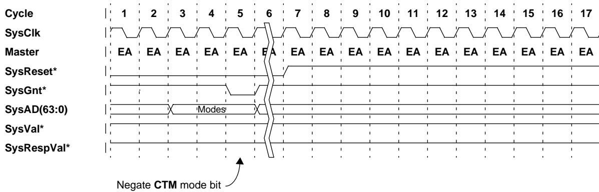
Figure 17-2 Cache Test Mode Exit Sequence
