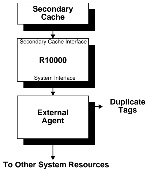
Figure 2-1 Uniprocessor System Organization
