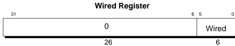
Figure 13-7 Wired Register
