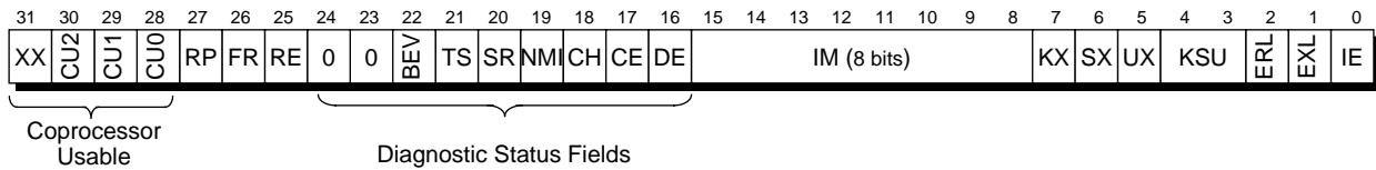
Figure 13-11 Status Register
