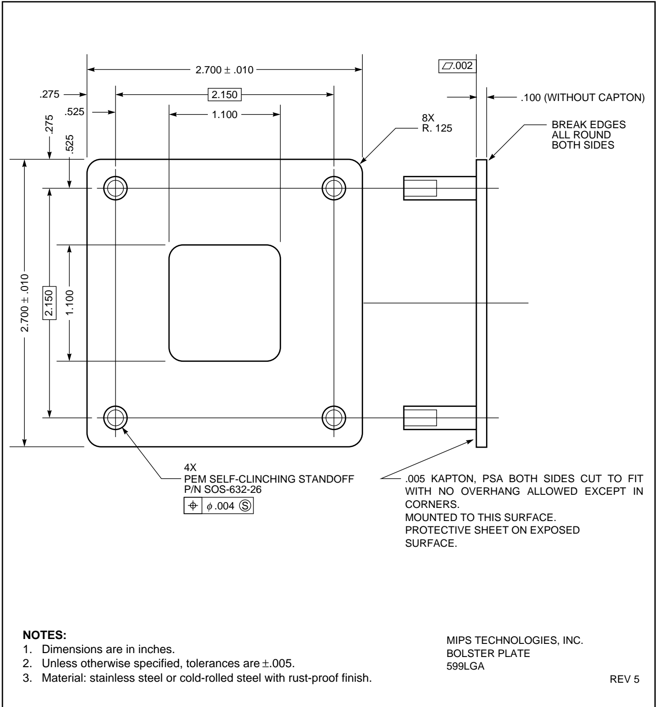
Figure 12-5 599LGA Bolster Plate
