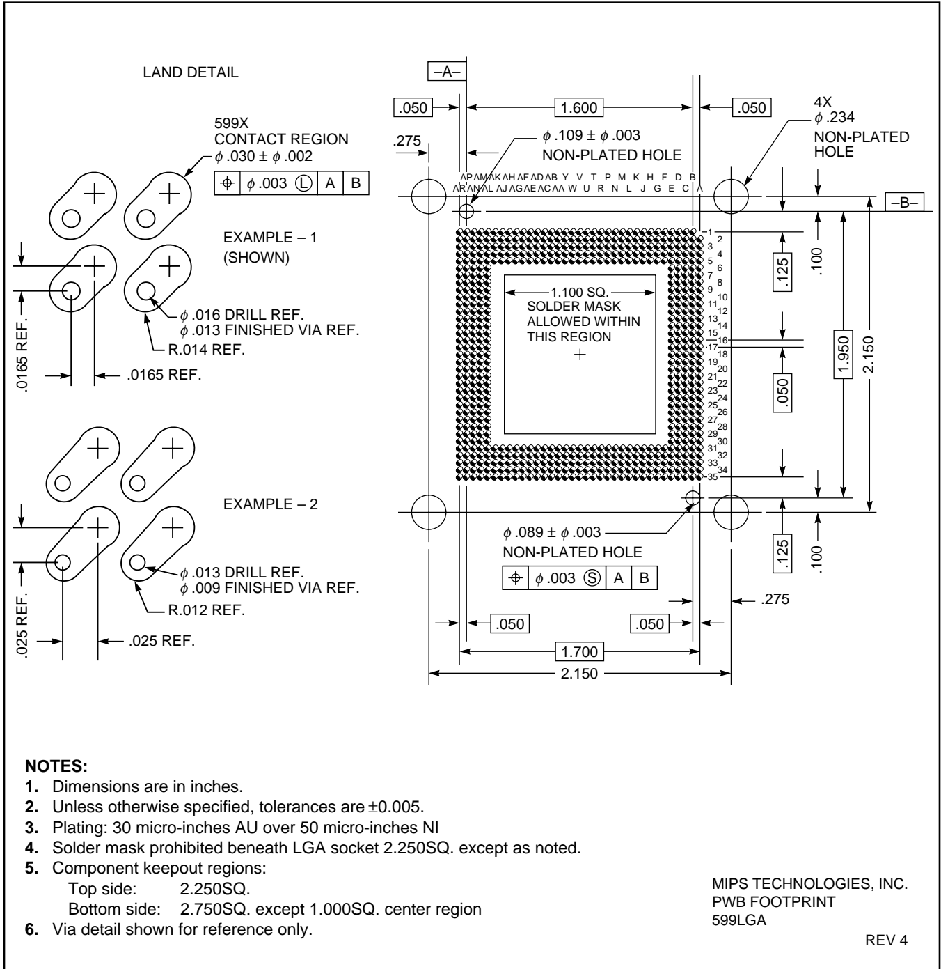
Figure 12-3 599LGA PWB Footprint
