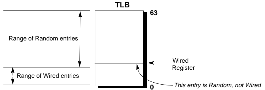
Figure 13-6 Wired Register Boundary
