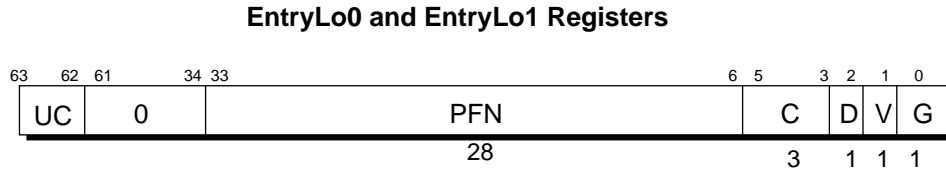
Figure 13-3 Fields of the EntryLo0 and EntryLo1 Registers
