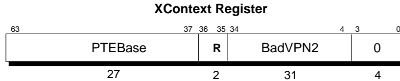
Figure 13-19 XContext Register Format
