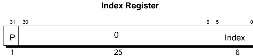
Figure 13-1 Index Register
