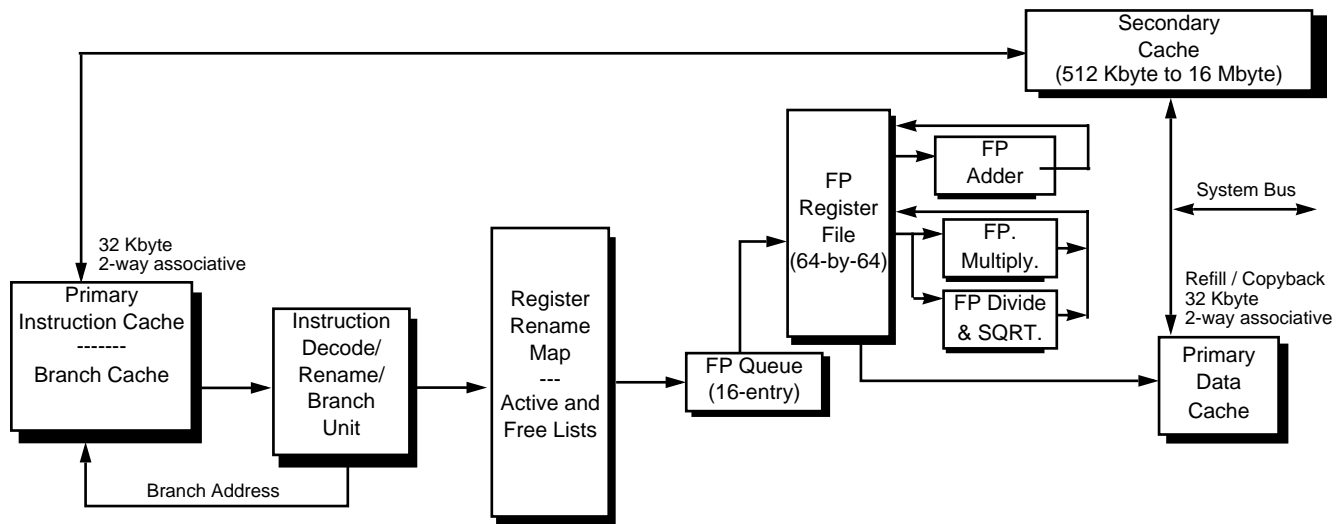
Figure 14-1 Logical Diagram of FP Operations
