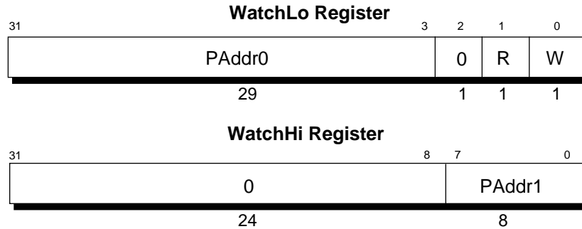
Figure 13-18 WatchLo and WatchHi Register Formats
