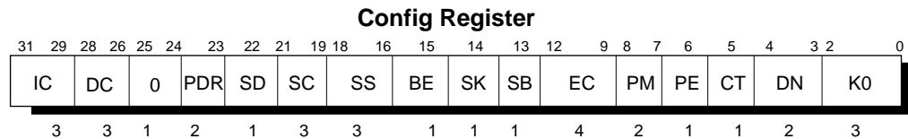
Figure 13-16 Config Register Format
