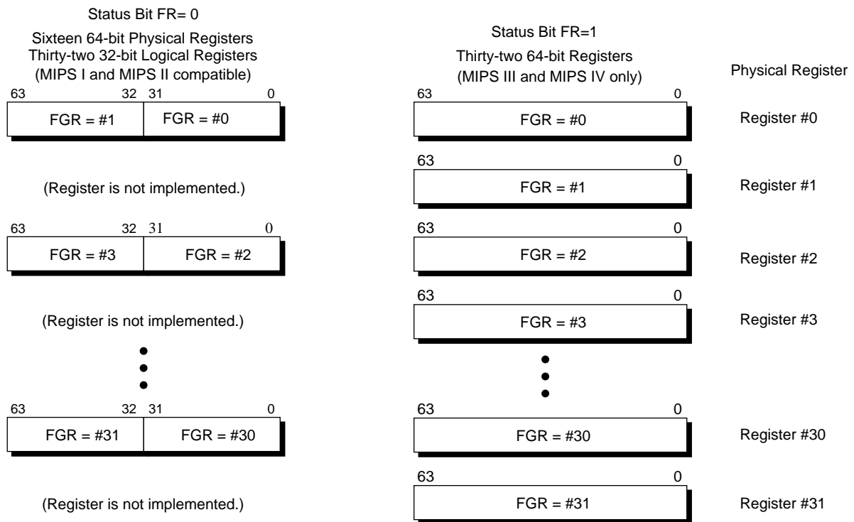
Figure 14-2 Floating-Point Registers
