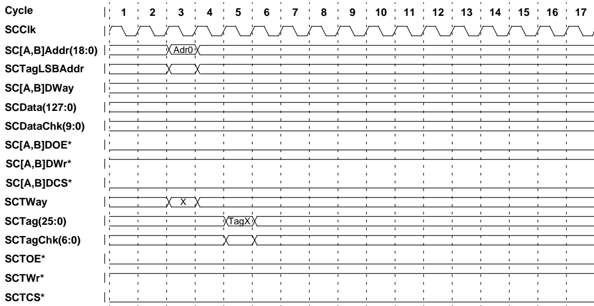
Figure 5-6 Tag Read Sequence
