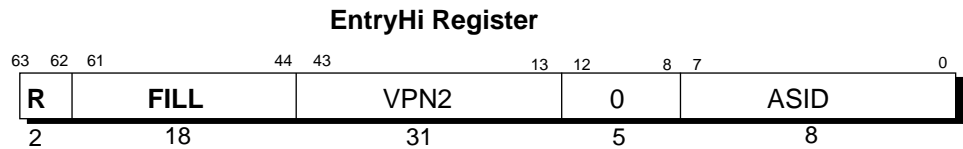
Figure 13-10 EntryHi Register
