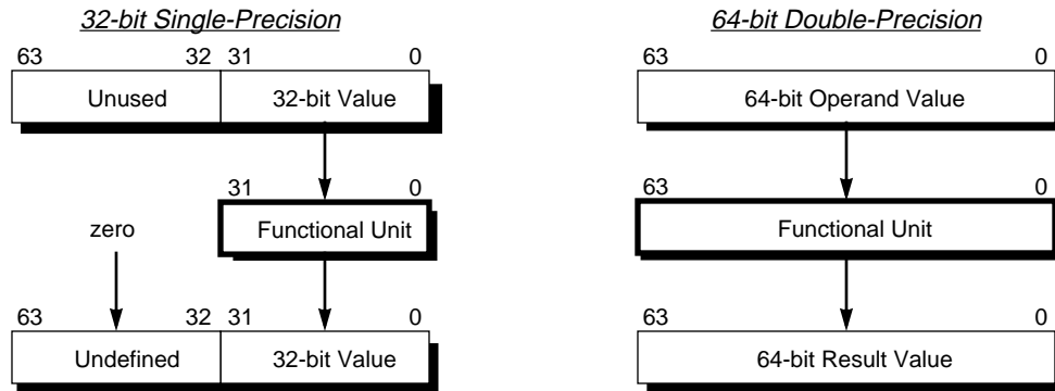
Figure 14-5 Operators on Floating-Point Registers
