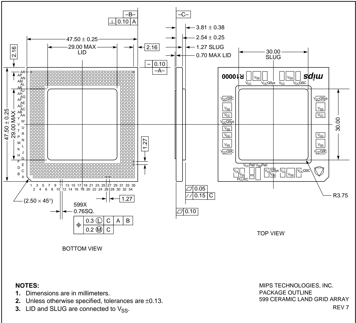
Figure 12-1 R10000 599CLGA Package Outline
