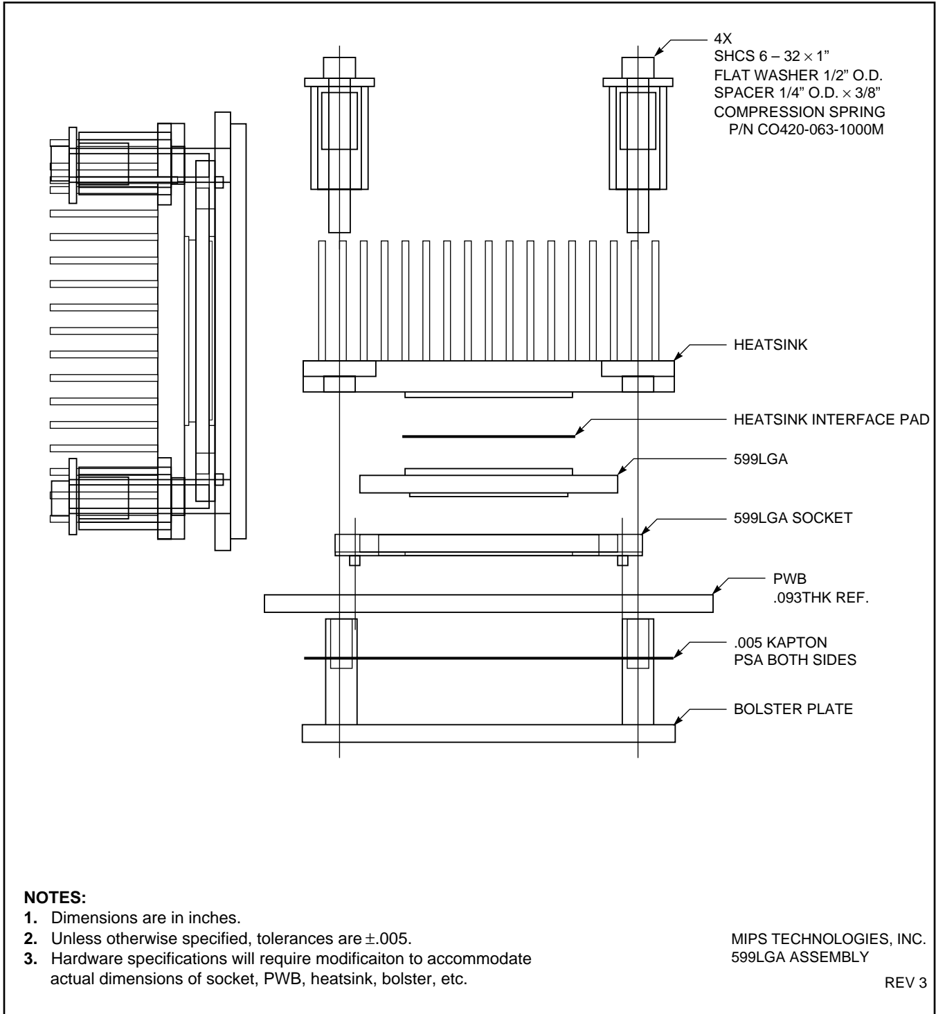
Figure 12-2 599LGA Assembly Drawing
