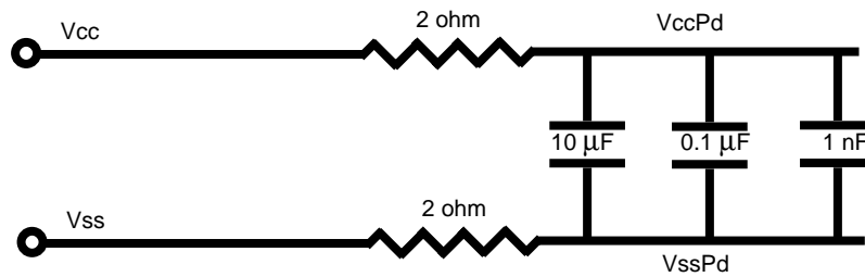
Figure 11-2 Decoupling VccPd and VssPd
