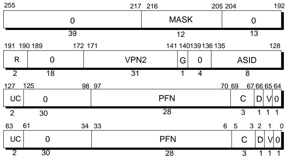
Figure 15-5 Format of a TLB Entry
