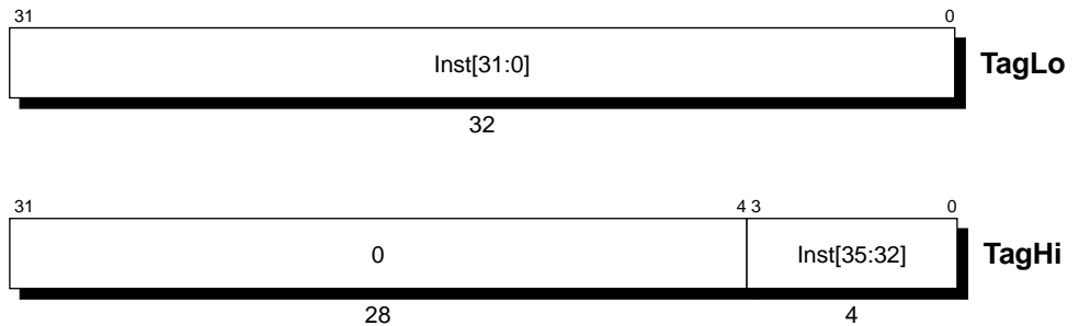
Figure 13-31 TagHi/Lo Register Fields in Primary Instruction Cache When CacheOp is Index Load/Store Data
