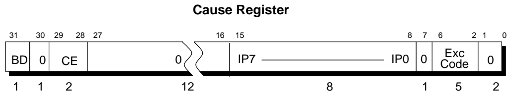
Figure 13-13 Cause Register Format
