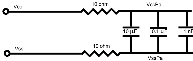
Figure 11-1 Decoupling VccPa and VssPa
