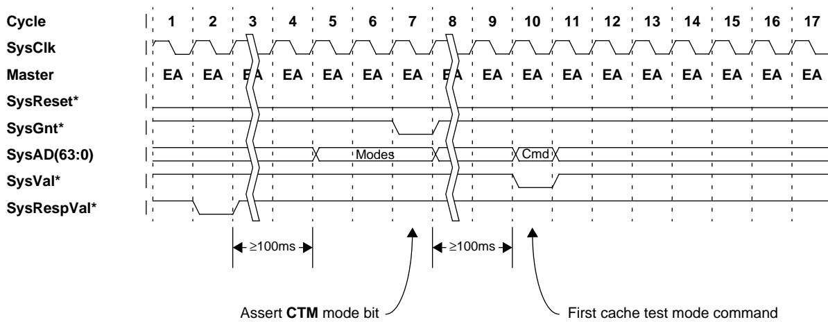
Figure 17-1 Cache Test Mode Entry Sequence
