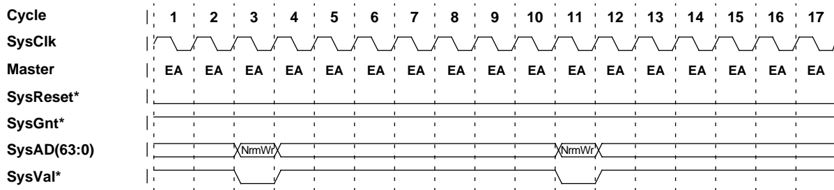
Figure 17-3 Cache Test Mode Normal Write Protocol
