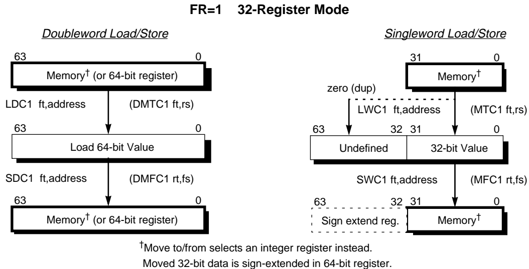
Figure 14-4 Loading and Storing Floating-Point Registers in 32-Register Mode
