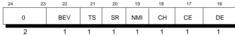
Figure 13-12 Diagnostic Status Field
