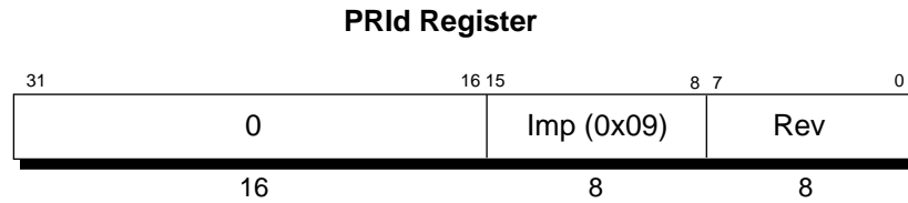
Figure 13-15 Processor Revision Identifier Register Format
