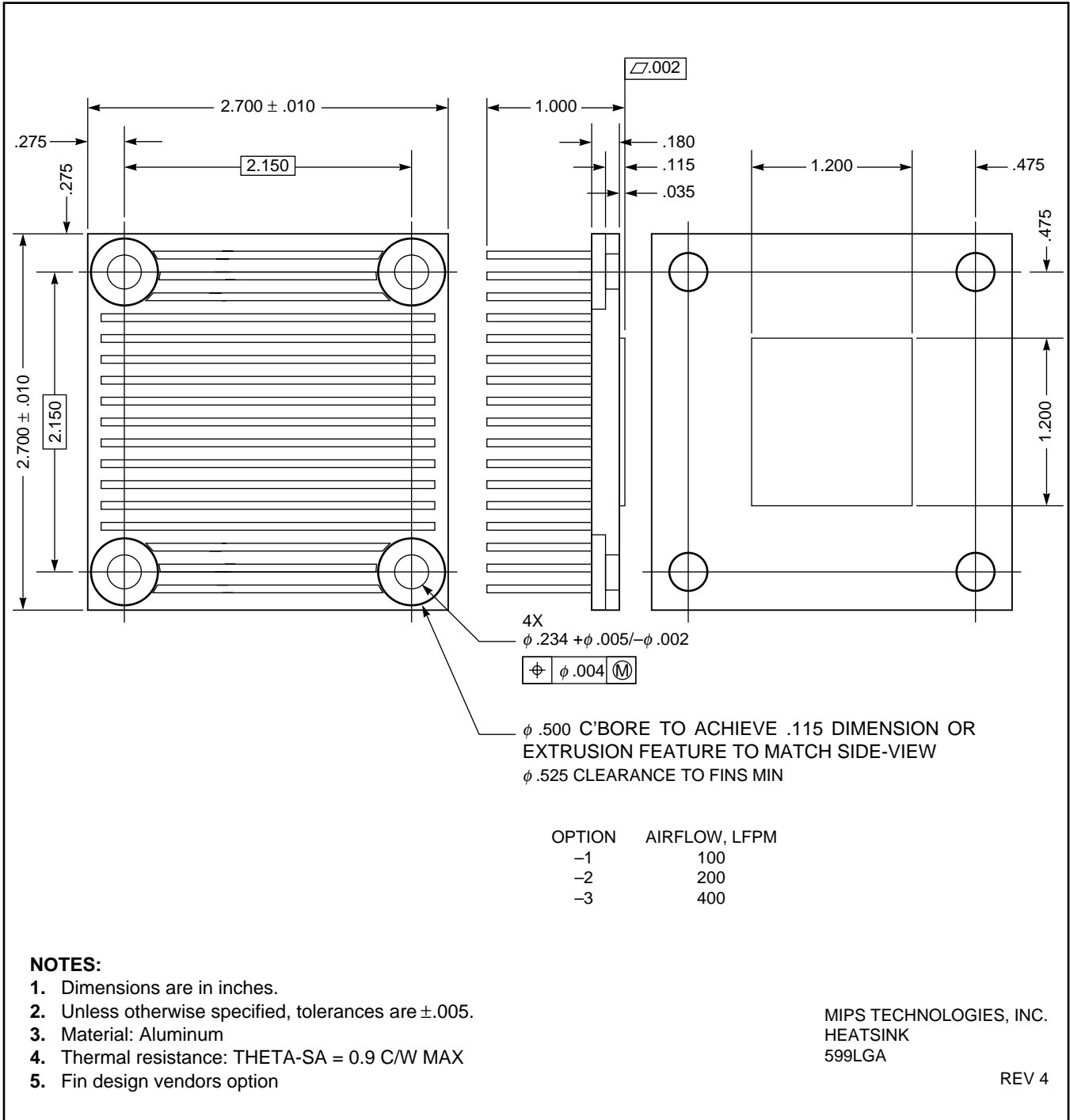
Figure 12-4 599LGA Heatsink
