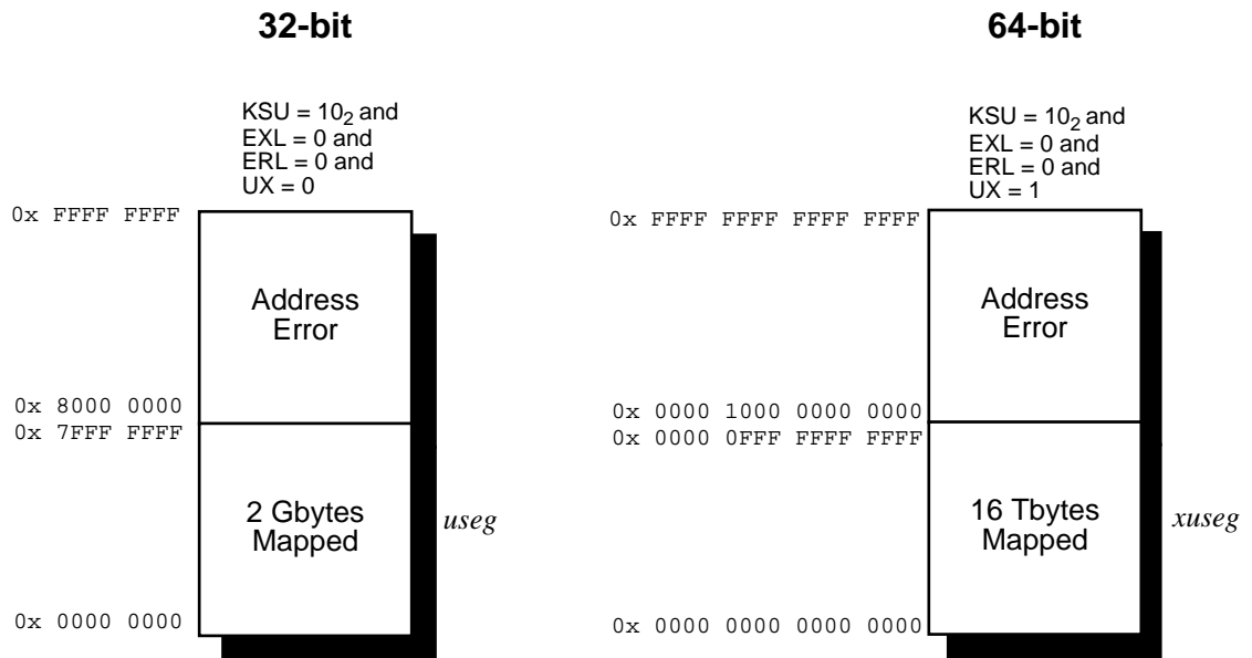
Figure 15-1 User Mode Virtual Address Space
