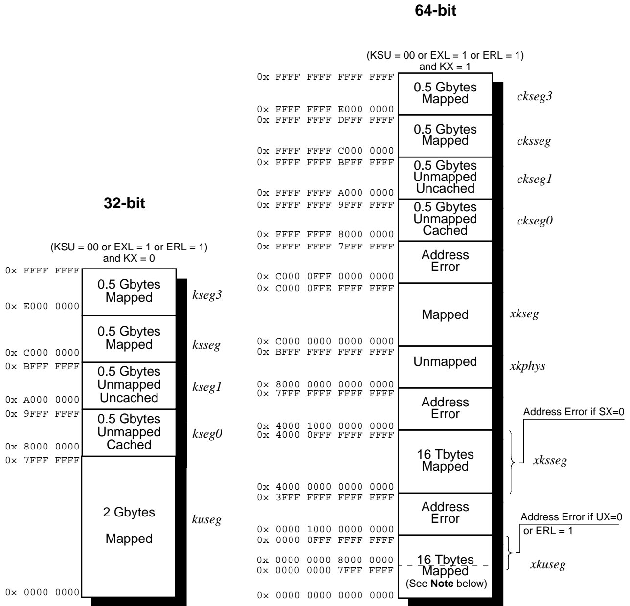
Figure 15-3 Kernel Mode Address Space
