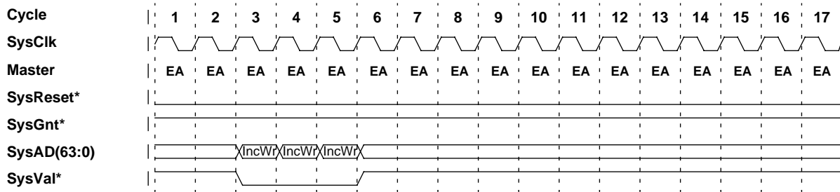
Figure 17-4 Cache Test Mode Auto-Increment Write Protocol
