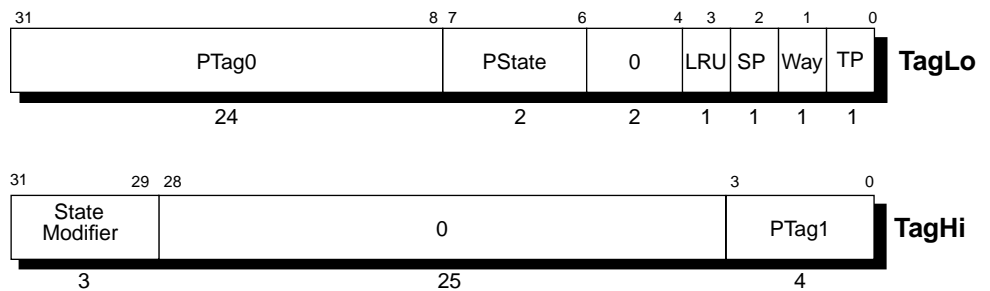
Figure 13-29 TagHi/Lo Register Fields in Primary Data Cache When CacheOp is Index Load/Store Tag
