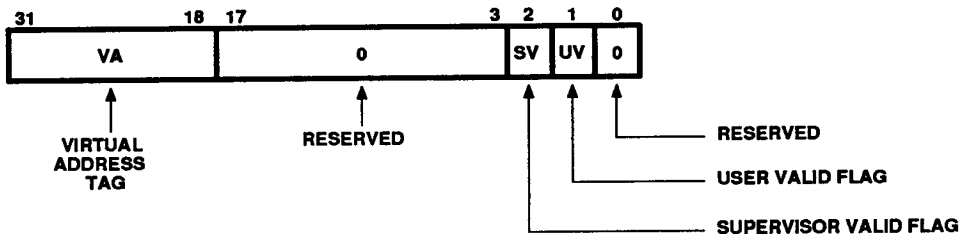
(b) TLB VA FIELD ACCESS FORMAT
