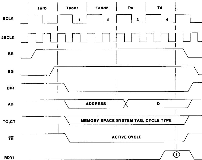
Figure 46 Single Word Write (1 Wait State)
