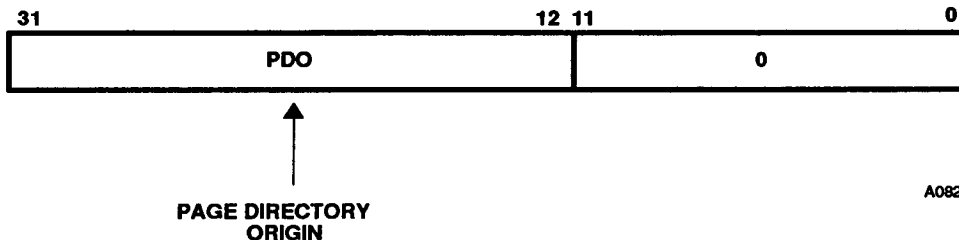
Figure 33 PDO Register Access Format
