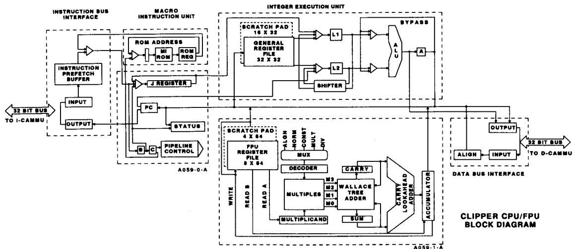
Figure 3 Detailed CPU/FPU Block Diagram
