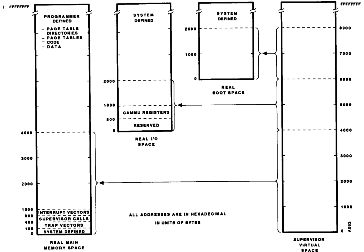
Figure 5 Real Address Spaces—HTLB Mapping
