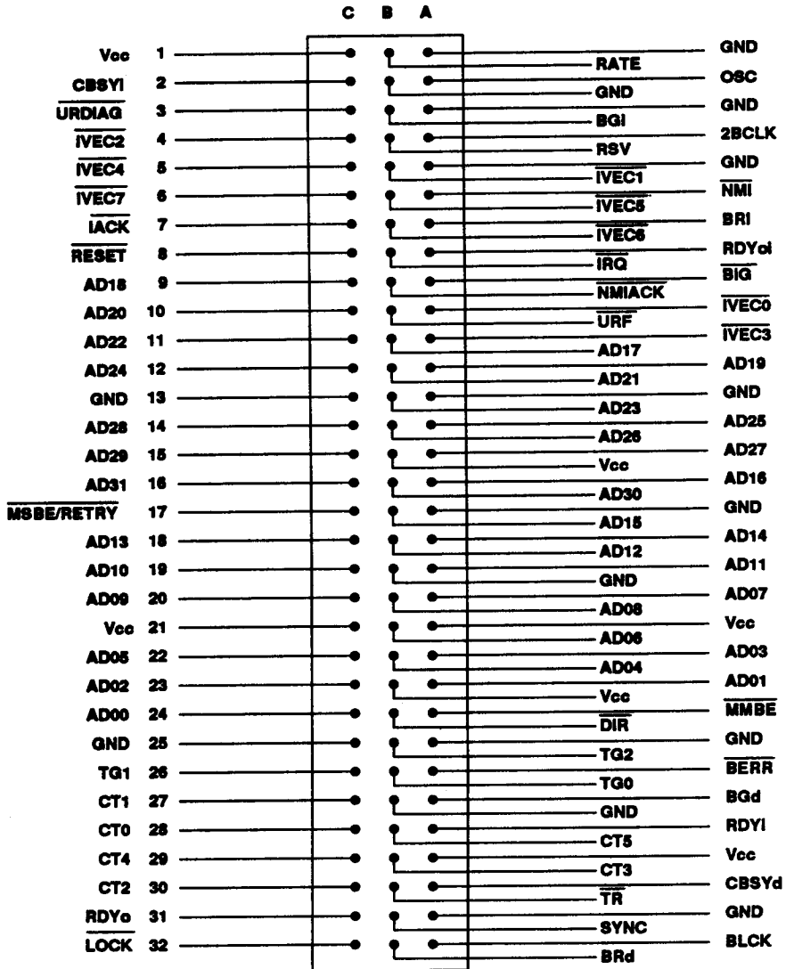
Figure 70 Pinout of CLIPPER C300 Module C300C3BLX Box Connector
