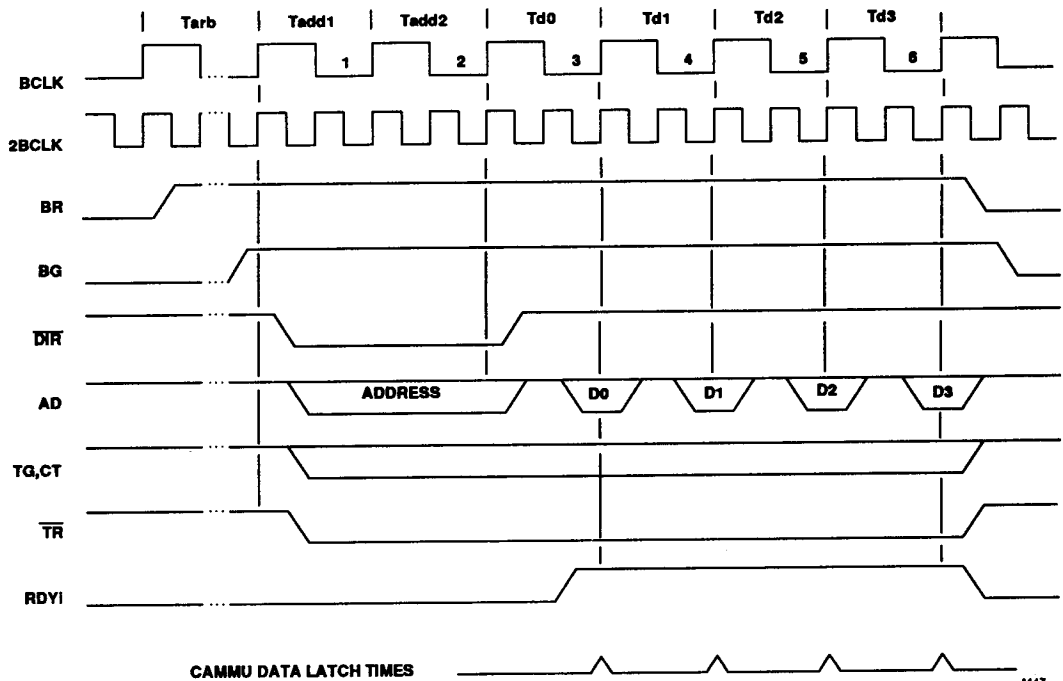
Figure 44 Quadword Read (No Wait States)
