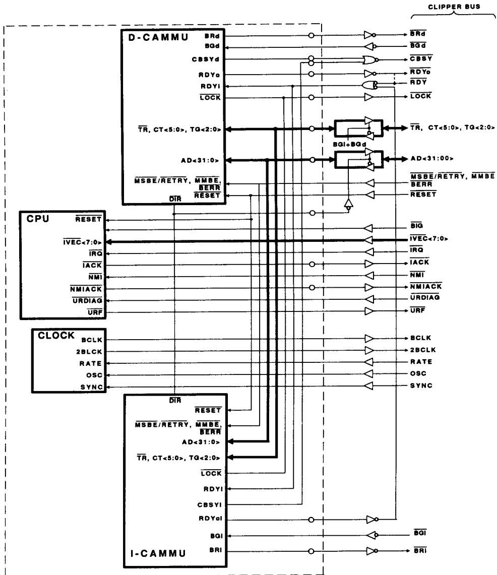
Figure 37 CLIPPER C300 Bus Interface
