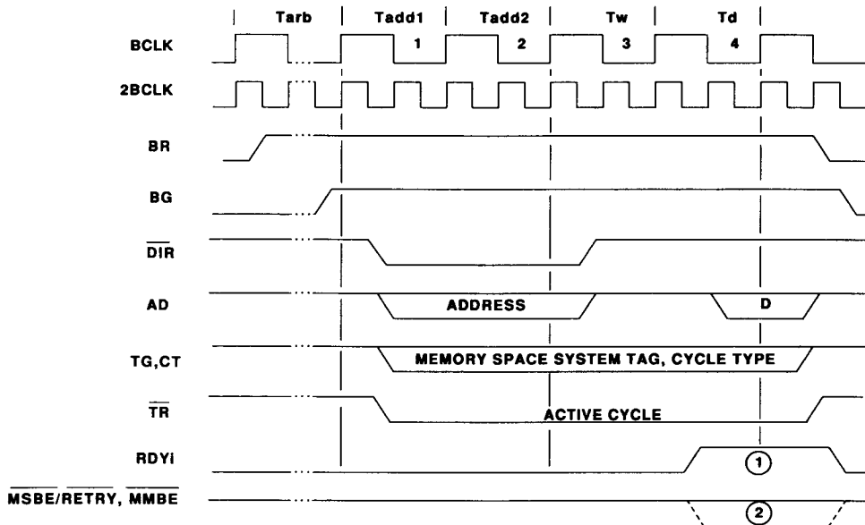
Figure 41 Single Word Read (1 Wait State)
