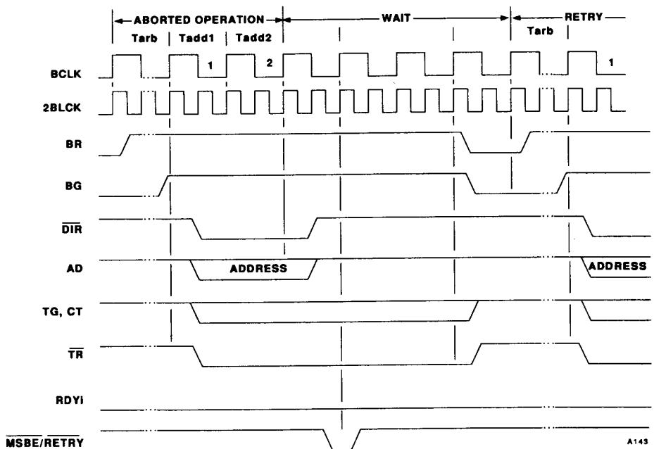
Figure 42 Bus Retry (Single Word Read Example)
