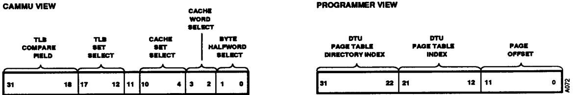
Figure 17 CPU Virtual Address Format
