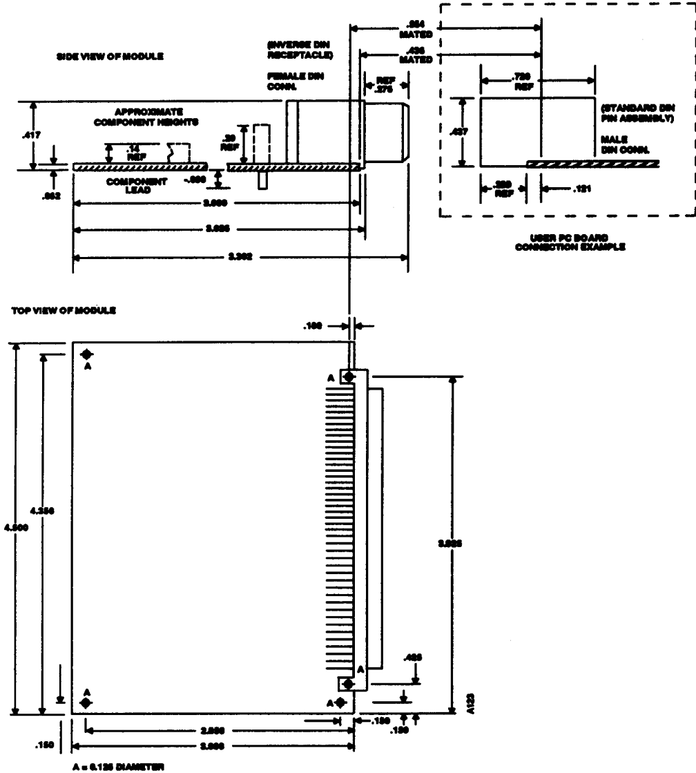
Figure 67 CLIPPER C300 Module C300C3MLX with Standard Connector
