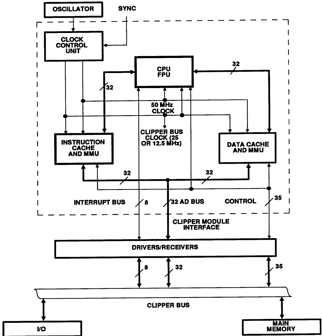
Figure 1 CLIPPER C300 Module Block Diagram
