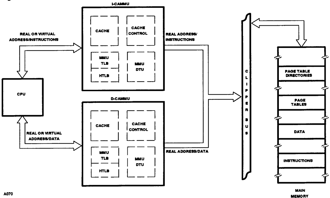
Figure 15 CAMMU Interface
