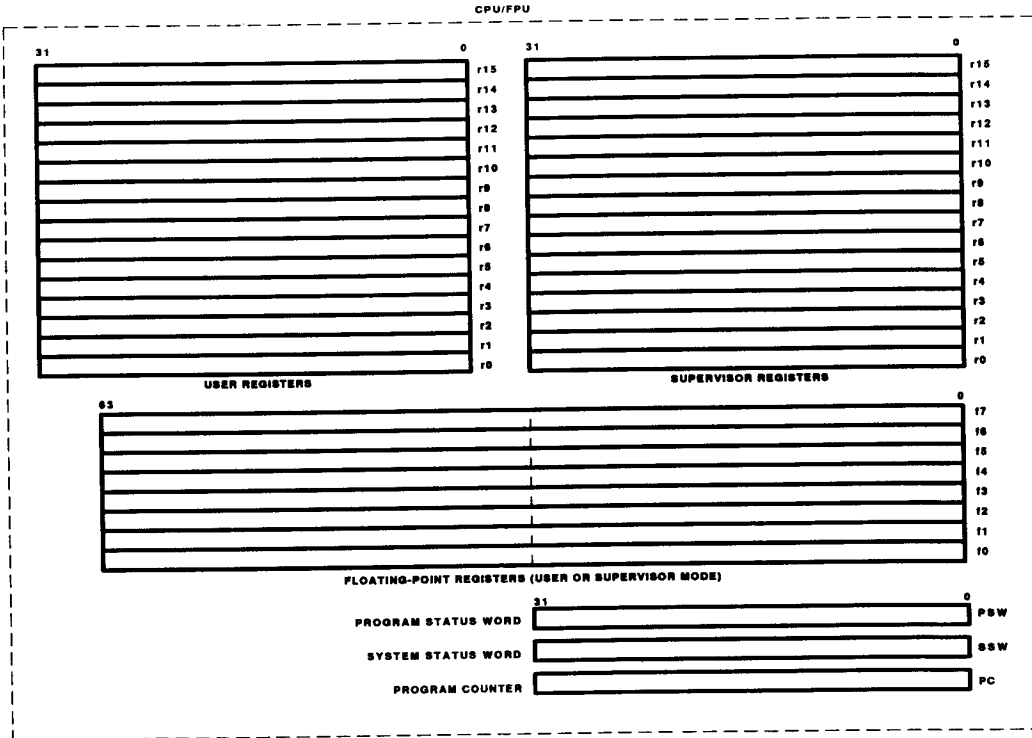
Figure 8 C300 Programming Model
