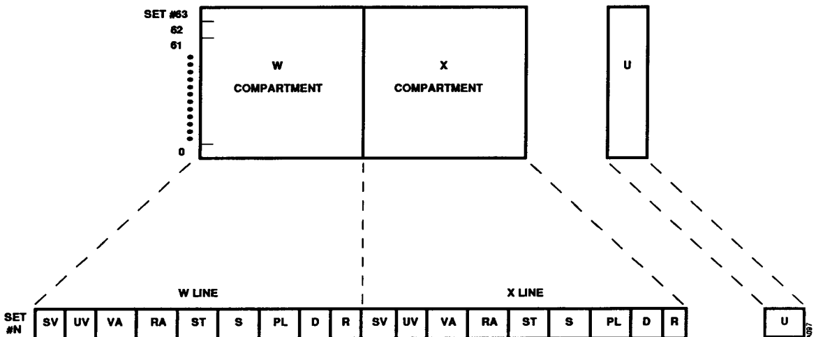
Figure 20 CLIPPER TLB
