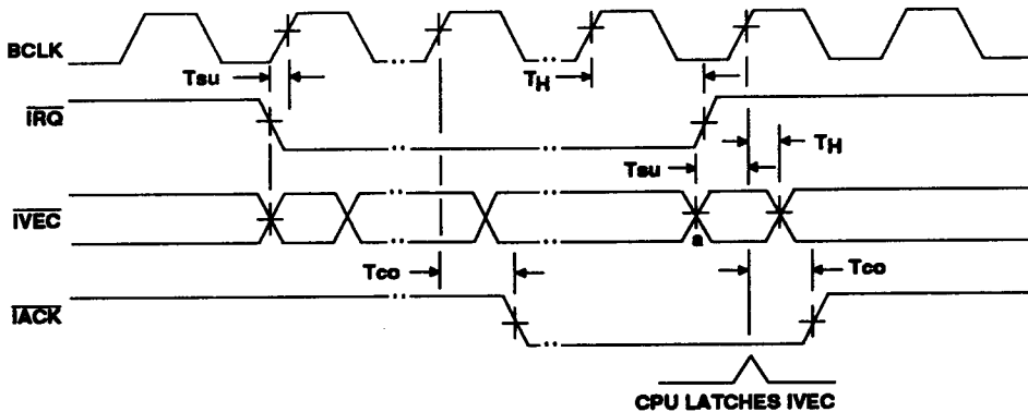
Figure 59 Maskable Interrupt Request/Acknowledge Timing
