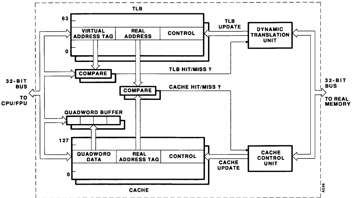
Figure 18 Simplified CAMMU Block Diagram
