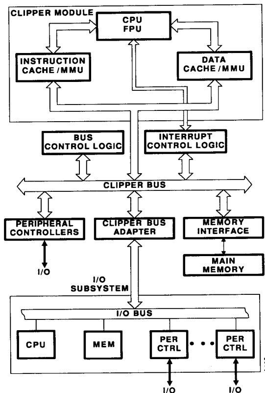
Figure 39 CLIPPER System
