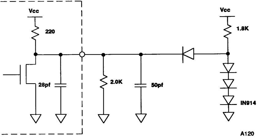
Figure 64 Module Output Test Load
