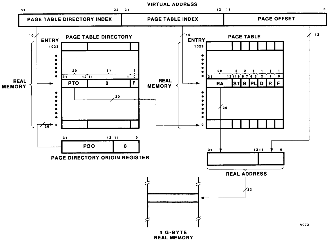
Figure 23 DTU Virtual Address Translation
