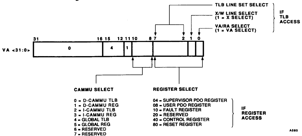
Figure 31 CAMMU Addressing
