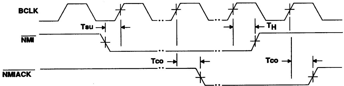
Figure 60 Non-Maskable interrupt Request/Acknowledge Timing
