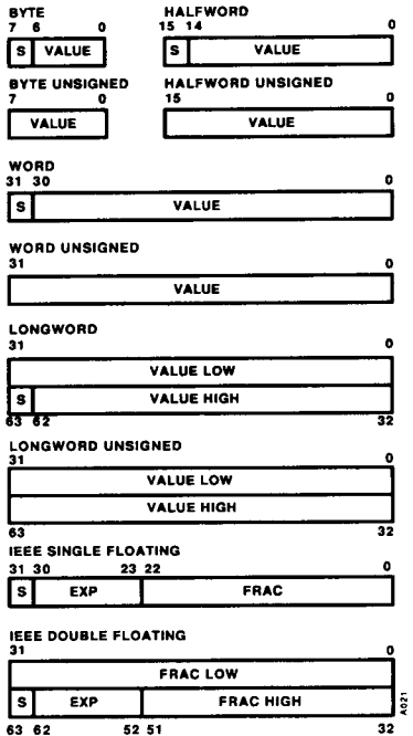
Figure 7 Representation of Data In Memory
