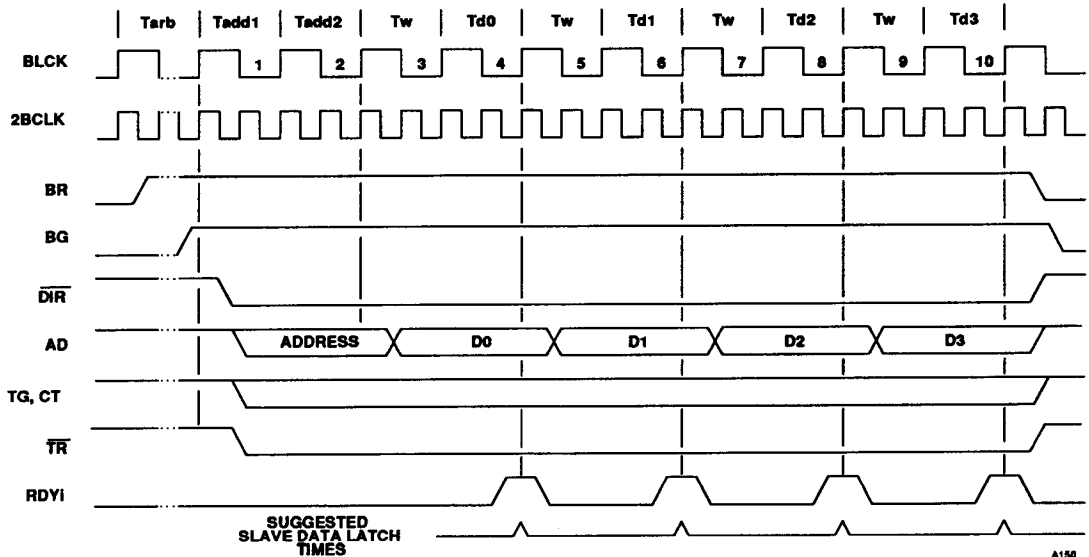
Figure 48 Quadword Write (4 Wait States)
