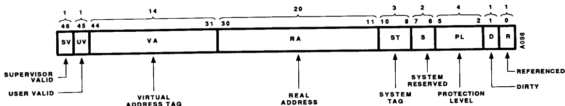
Figure 21 TLB Line Format and Description
