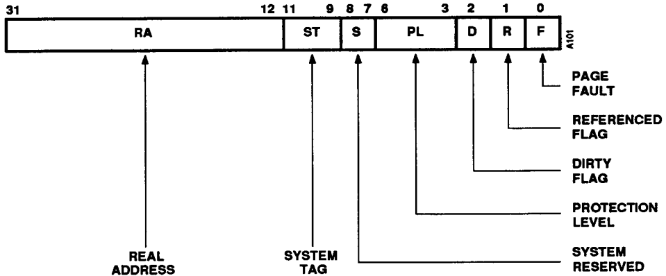
Figure 25 Page Table Entry Format
