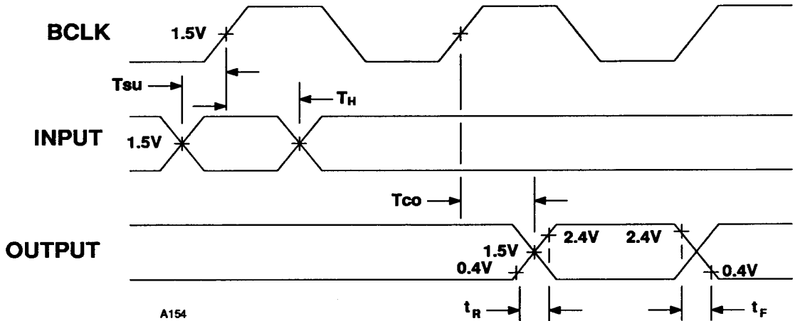
Figure 51 AC Measurement Points
