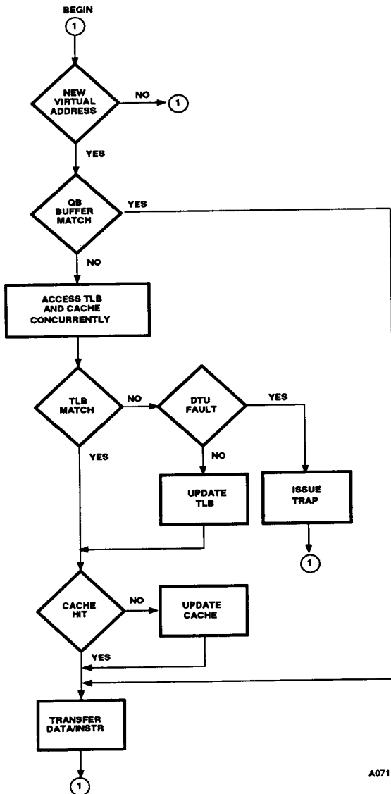
Figure 16 Basic CAMMU Functional Flow
