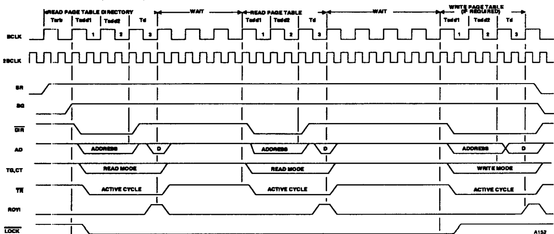
Figure 50 Read-Modify-Write (DTU Operation)
