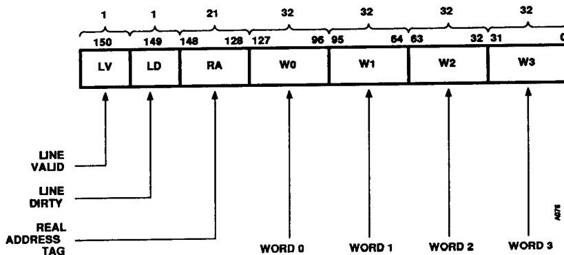
Figure 27 CLIPPER Cache Line Format
