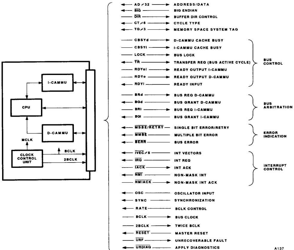
Figure 36 CLIPPER Bus Signals
