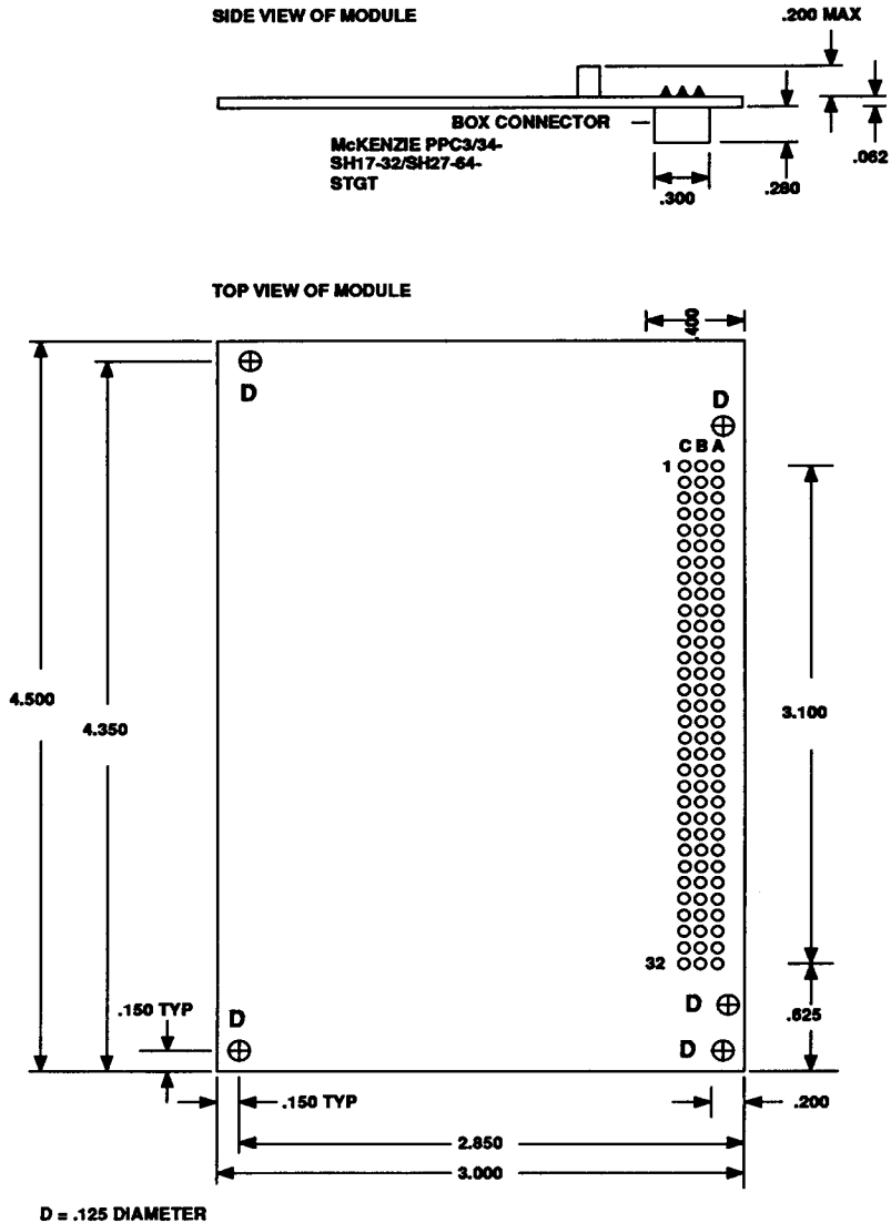
Figure 69 CLIPPER C300 Module C300C3BLX with Box Connector
