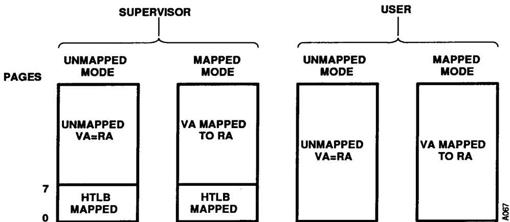
Figure 11 Address Mapping—Mapped/Unmapped Modes
