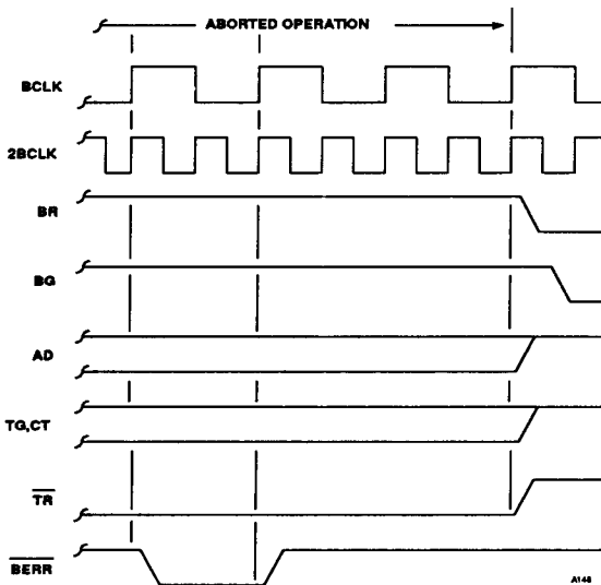
Figure 43 Bus Error
