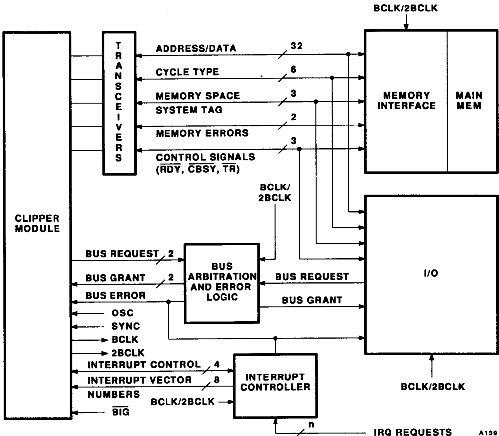
Figure 38 Example CLIPPER System (Block Diagram)
