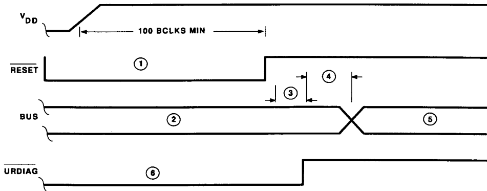
Figure 35 Reset Timing
