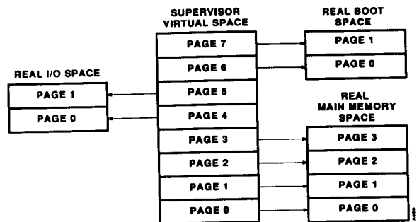
Figure 22 Hardwired TLB Mapping
