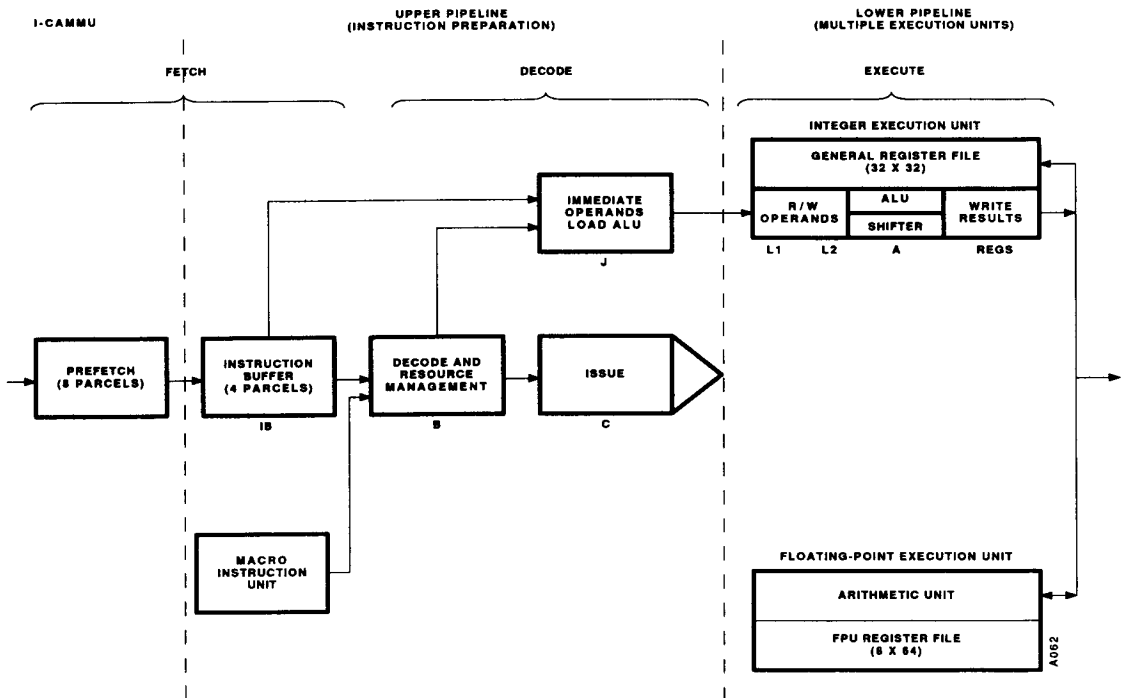
Figure 4 CLIPPER Pipeline
