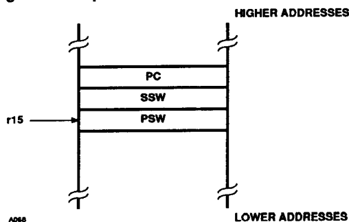
Figure 13 Supervisor Stack After INTRAP
