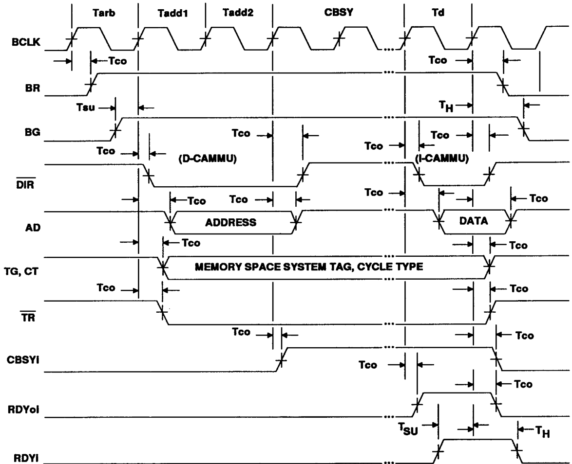
Figure 57 D-CAMMU Read from Companion I-CAMMU
