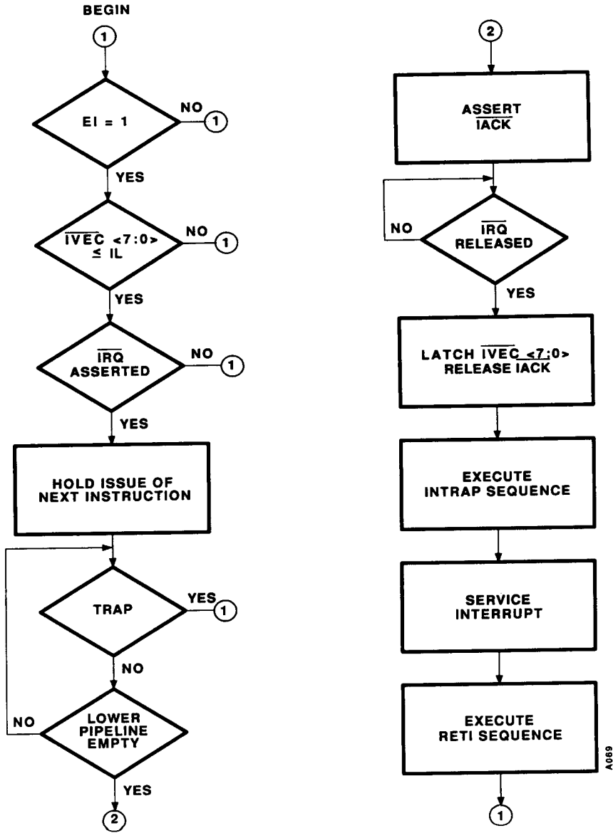
Figure 14 Interrupt Flow Diagram
