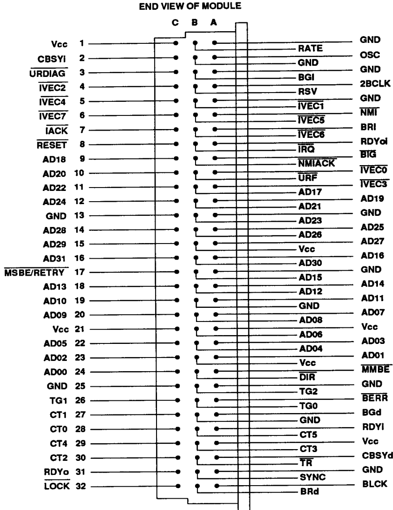
Figure 68 Pinout of CLIPPER C300 Module C300C3MLX Connector
