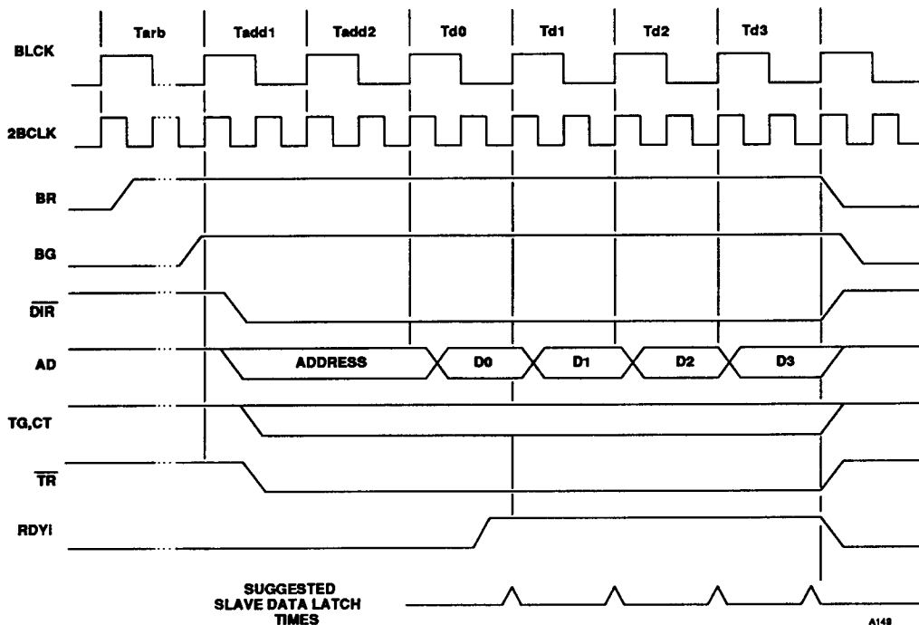
Figure 47 Quadword Write (No Wait States)
