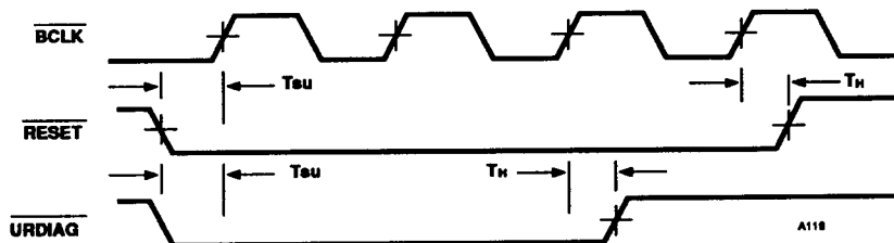
Figure 63 \overline{\text{RESET}} and \overline{\text{URDIAG}} Timing
