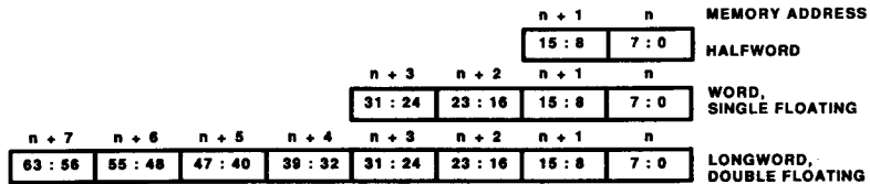
Figure 7 Representation of Data In Memory
