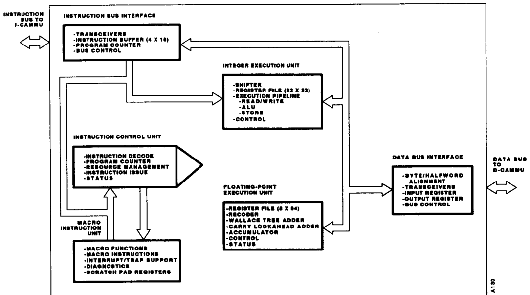
Figure 2 Simplified CPU Block Diagram
