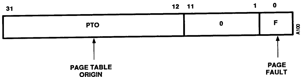
Figure 24 Page Table Format
